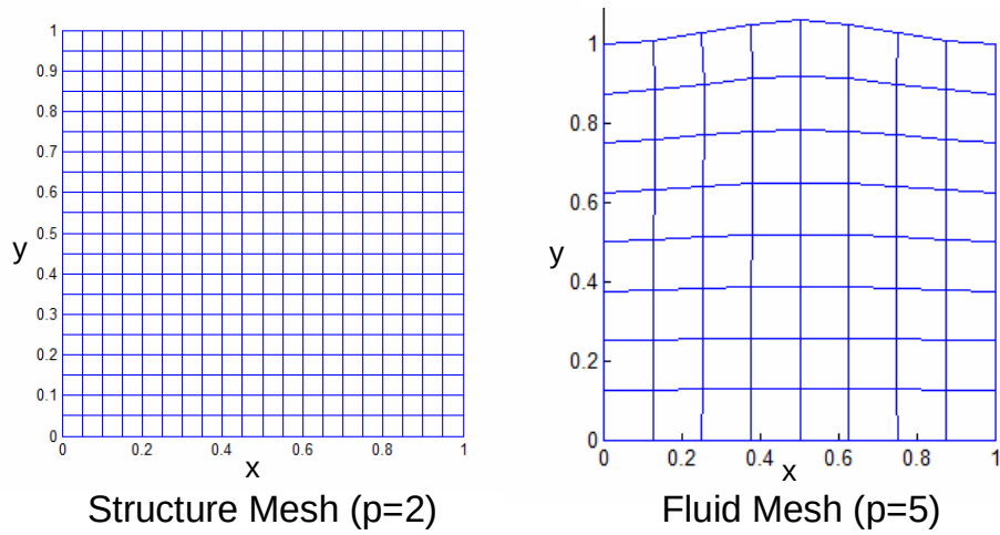
Figure 7.32 Sample Nonconformal Meshes for Case A (MMS FSI Problem)
