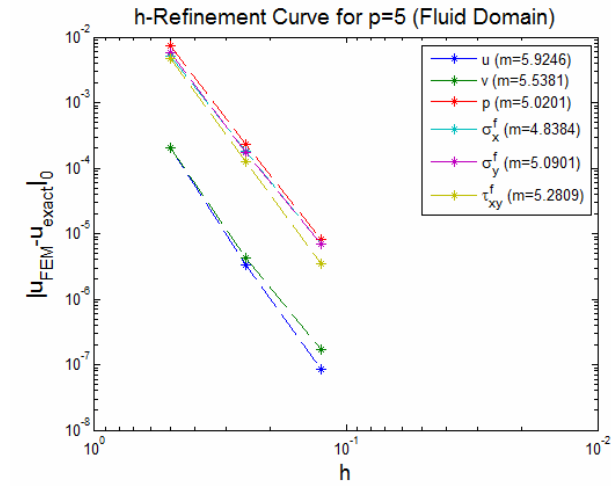
Figure 7.19 h -Refinement Curve for All Fluid Responses Using a p -value of 5 for MMS Problem
