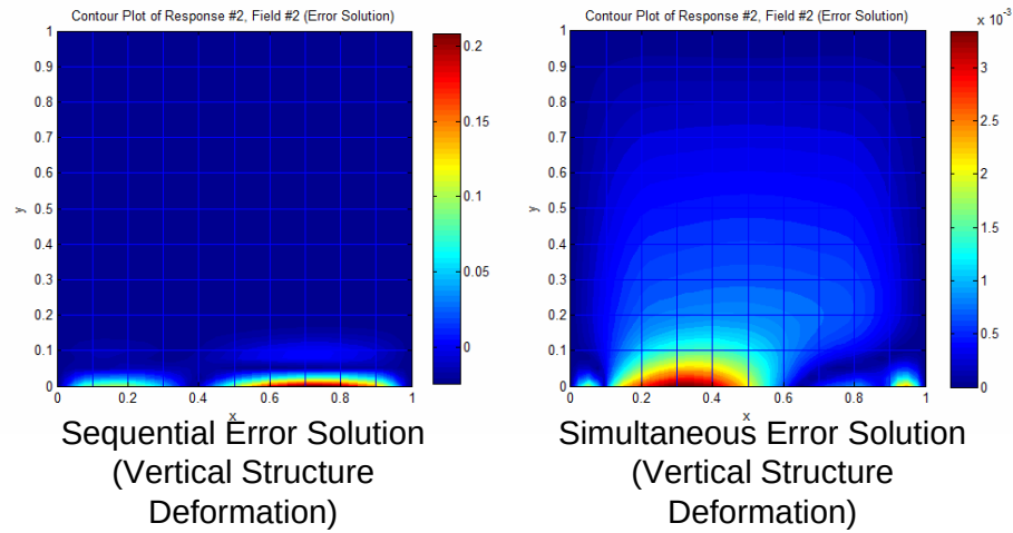
Figure 8.4 Vertical Structure Displacement Error Contour Plot for Sequential vs. Simultaneous Comparison for Transient MMS FSI Problem ( t=0.25 sec)
