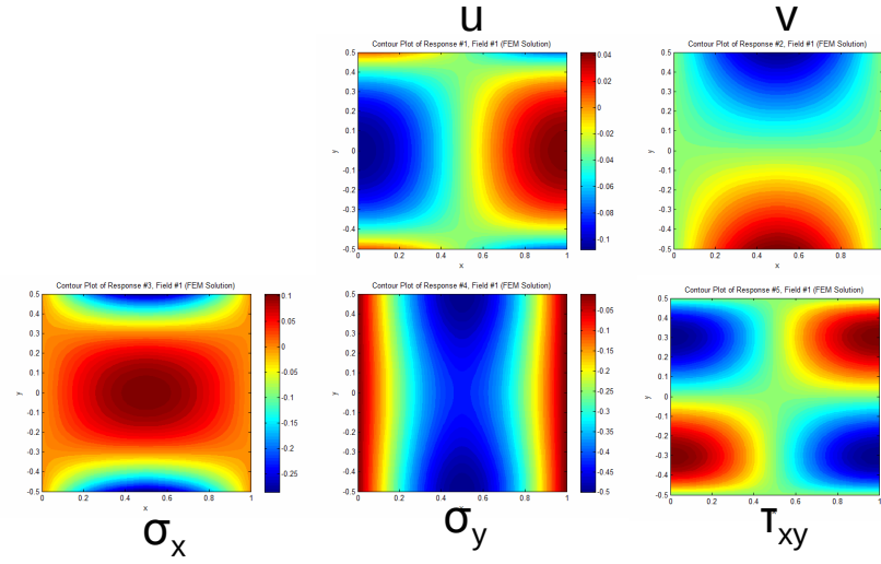
Figure 4.4 Thumbnail Plots of Exact Solution of Timoshenko and Goodier Problem
