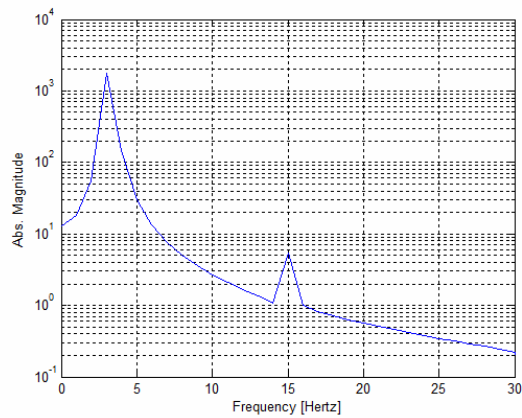
Figure 4.22 FFT of the Double Clamped Beam Transient Response Using LSFEM 2D Elasticity (Mid-Node Vertical Deformation Power Spectrum Plot)
