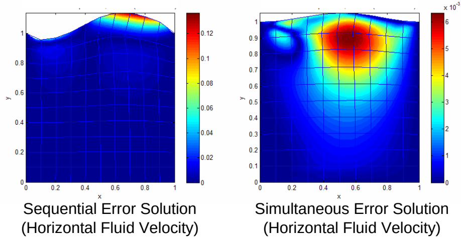
Figure 8.3 Horizontal Fluid Velocity Error Contour Plot for Sequential vs. Simultaneous Comparison for Transient MMS FSI Problem ( t=0.25 sec)
