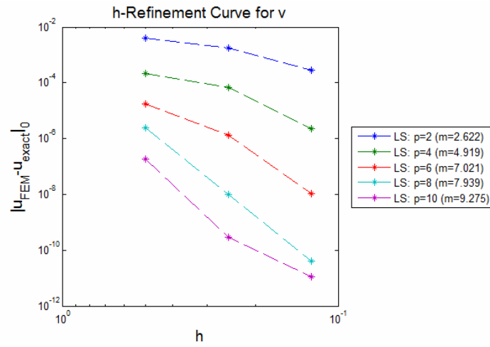
Figure 7.14 h -Refinement Curve for Fluid Primary Response ( v ) for MMS Problem
