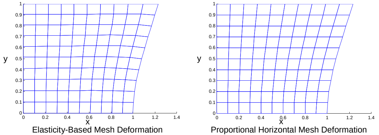
Figure 7.5 Comparison of Different Mesh Movement Schemes for Driven Cavity Flow with Flexible Right Wall Problem
