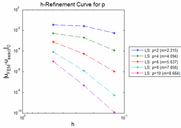
Figure 7.15 h -Refinement Curve for Fluid Secondary Response ( p ) for MMS Problem
