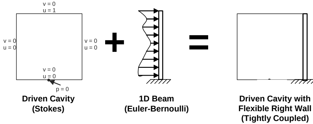
Figure 7.1 Assembly of Driven Cavity Flow with Flexible Right Wall with Two-Fields
