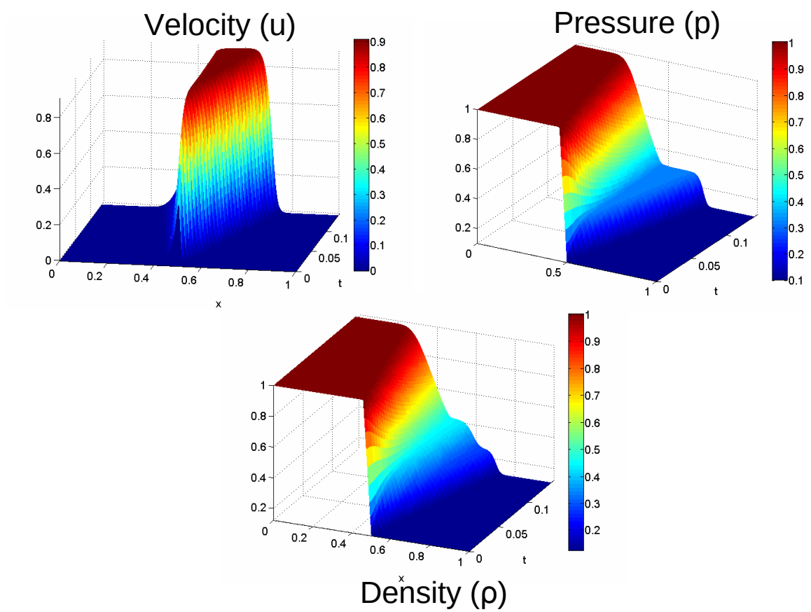
Figure 5.8 Time History of The Shock Tube Problem ( 0 \leq T \leq 0.14 )
