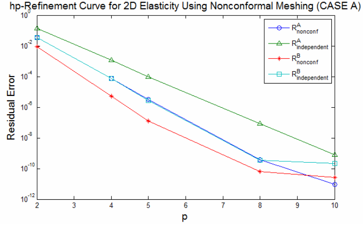
Figure 6.9 hp -Refinement Curve for Case A Examining Consistent Error Rates Between Nonconformal and Independent Solutions
