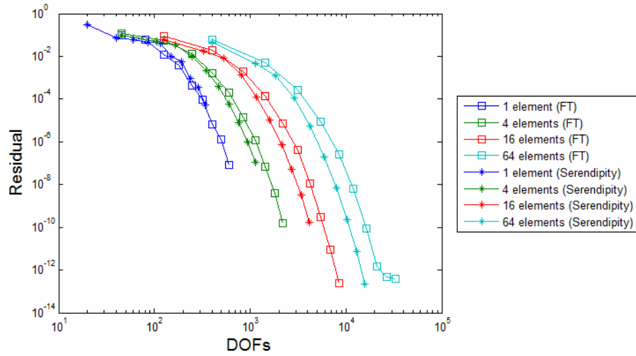
Figure 4.5 Comparison Between Serendipity Shape Functions and Full Tensor Product (FT) Shape Functions for Timoshenko and Goodier Elasticity Problem
