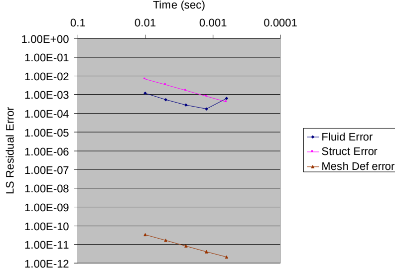
Figure 8.1 \Delta t -Refinement Examining the LSFEM Residual for Transient MMS FSI Problem Using Simultaneous Method ( t = 0.01 seconds, 100 Elements with p -value of 4)
