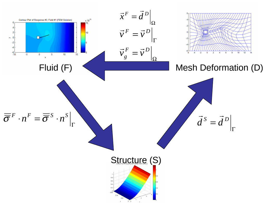
Figure 6.2 Sequential Fluid-Structure Interaction Process
