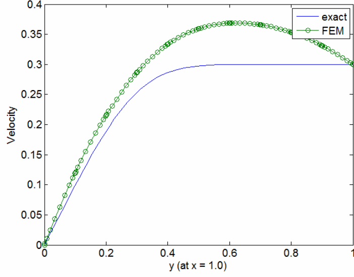
Figure 5.6 Blasius Plate Velocity Results Compared to Exact Solution at x = 1.0
