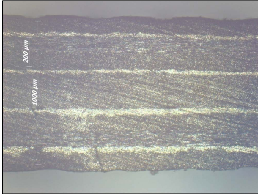
Figure 15. Configuration I (Inter-laminar), 200 gsm nickel (note four distinct layers of 50 gsm nickel evenly dispersed).
