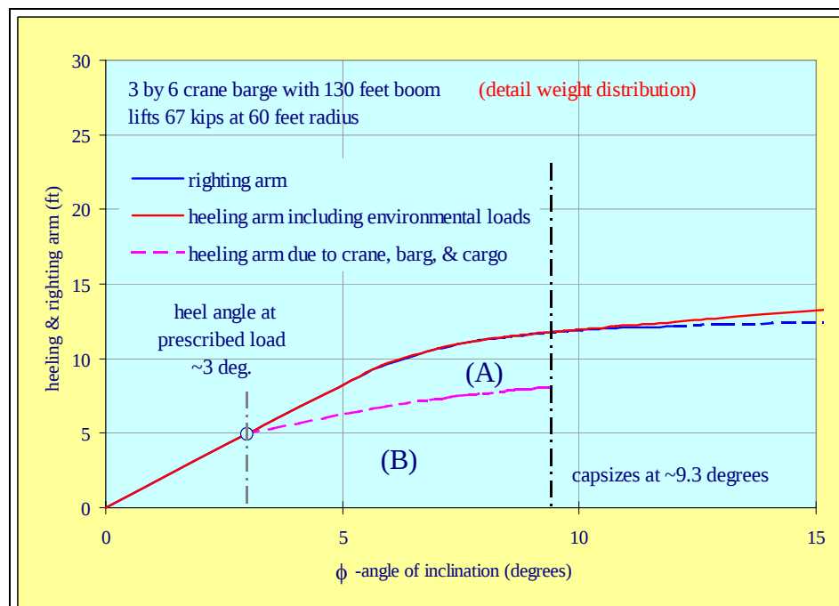
Figure 23. Reserve stability of 3 by 6 barge with 67-kip load at 60 feet radius.
