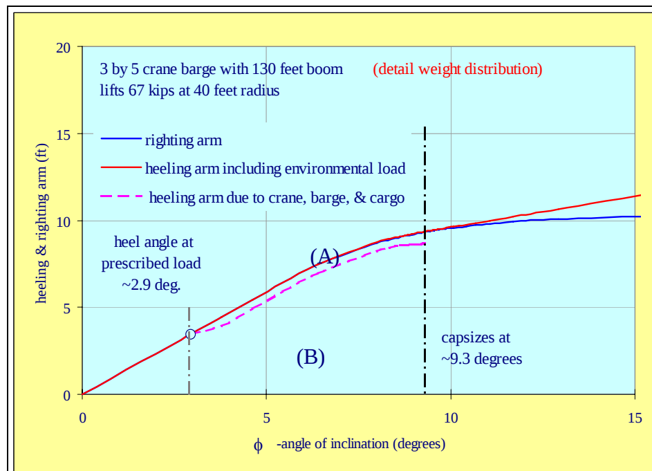
Figure 25. Reserve stability of 3 by 5 barge with 67-kip load at 40 feet radius.
