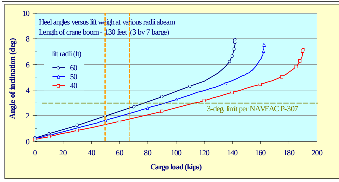
Figure 16. Performance of 3 by 7 barge: Set No. 1.
