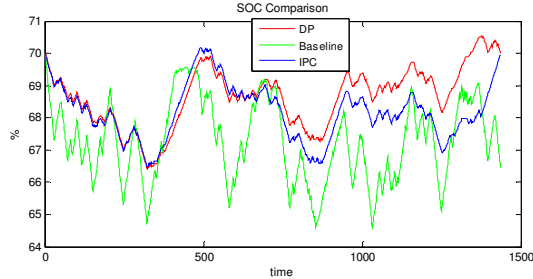
(c) SOC compensation during driving cycle LA92
