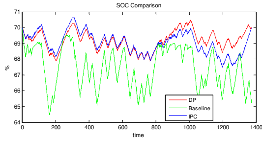
(a) SOC compensation during driving cycle UDDS
