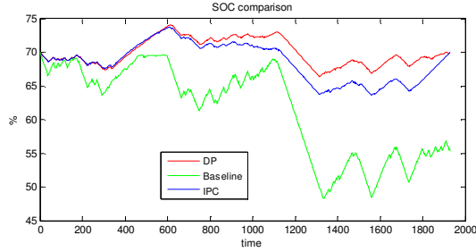
(b) SOC compensation during driving cycle UNIF01
