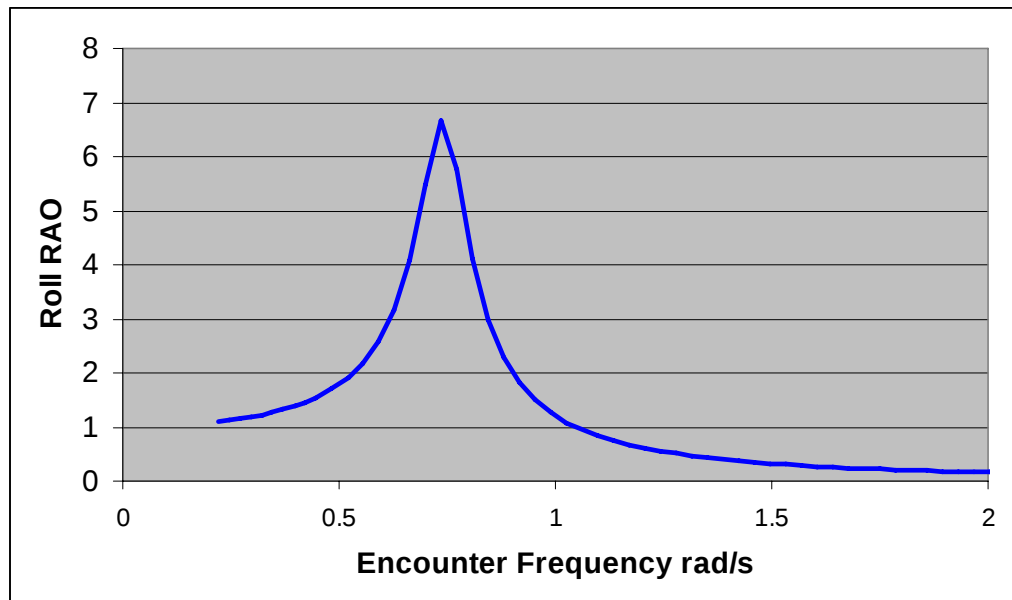
Figure 16 – Roll RAO for the GFS Station Ship in Beam Seas
