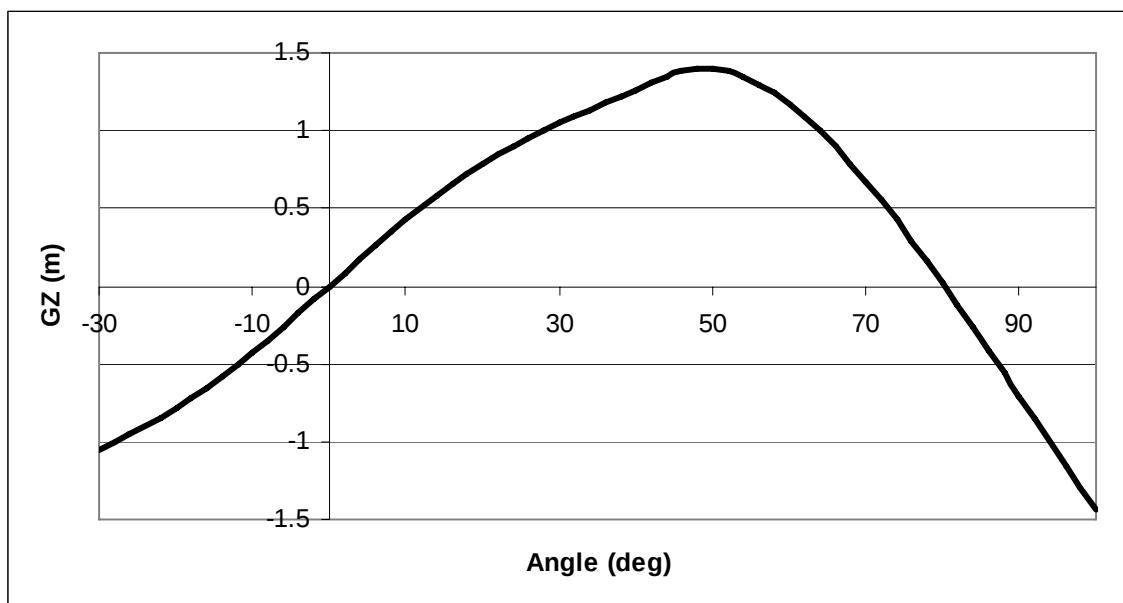
Figure 14 - GZ Curve
