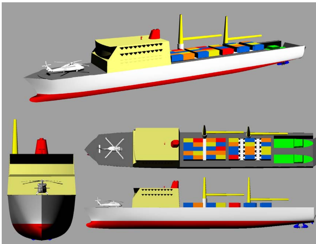
Figure 8 – GFS Station Ship Concept
