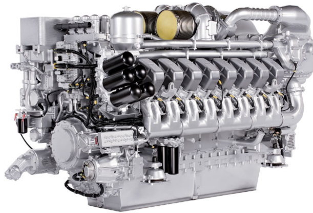
Figure 7: Detroit MTU Diesel Engine Model 16v4000 M61R
