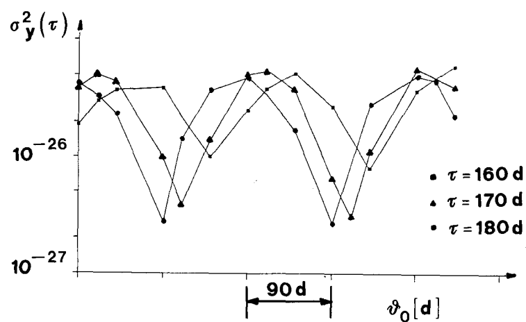
Fig. 9 - \sigma_y^2(\tau) of Cs9 vs. the measurement starting point or phase \vartheta_0 for three \tau values.
