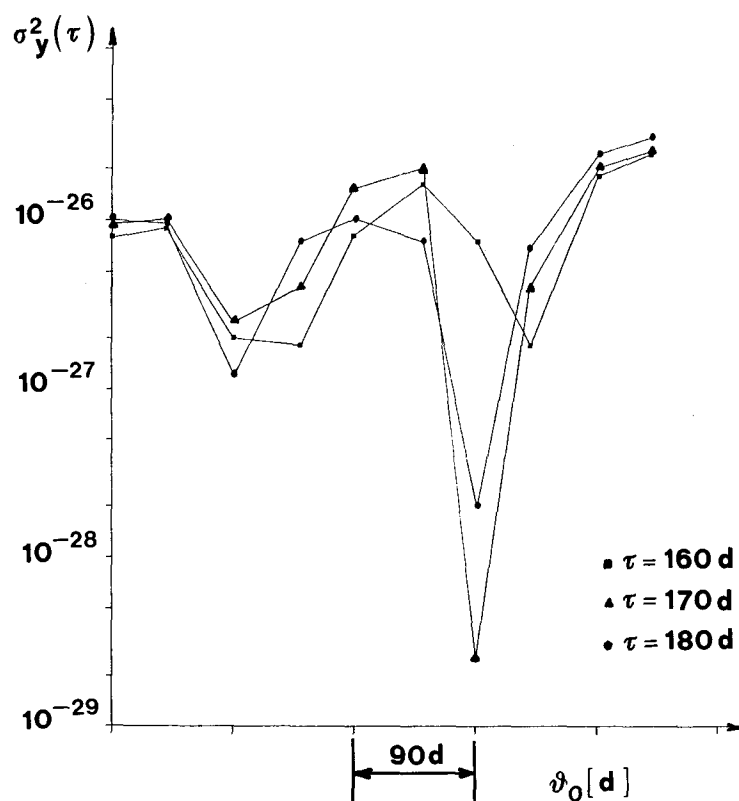
Fig. 10 - \sigma_y^2(\tau) of Cs6 vs. the measurement starting point or phase \vartheta_0 for three \tau values.
