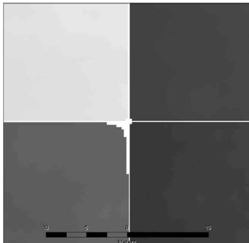
Step 2: Digital Elevation Models (DEMs) created from TINs. Gaps are slightly larger.
