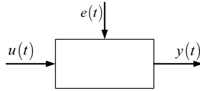
Figure 78: Black box structure. u(t) is the input, y(t) denotes the output and e(t) represents the model error.
