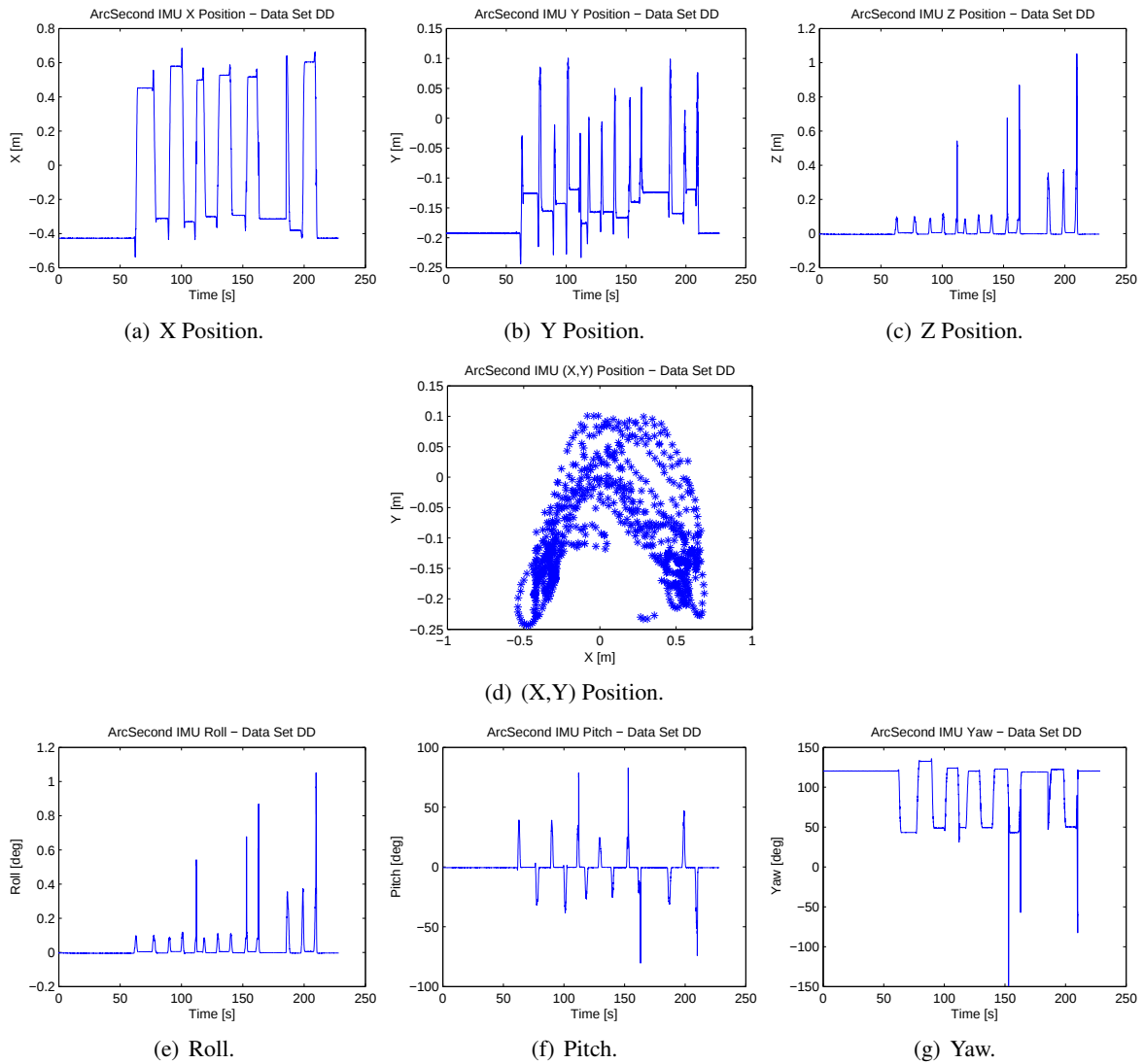
Figure 91: ArcSecond ground truth for data set 'DD'.
