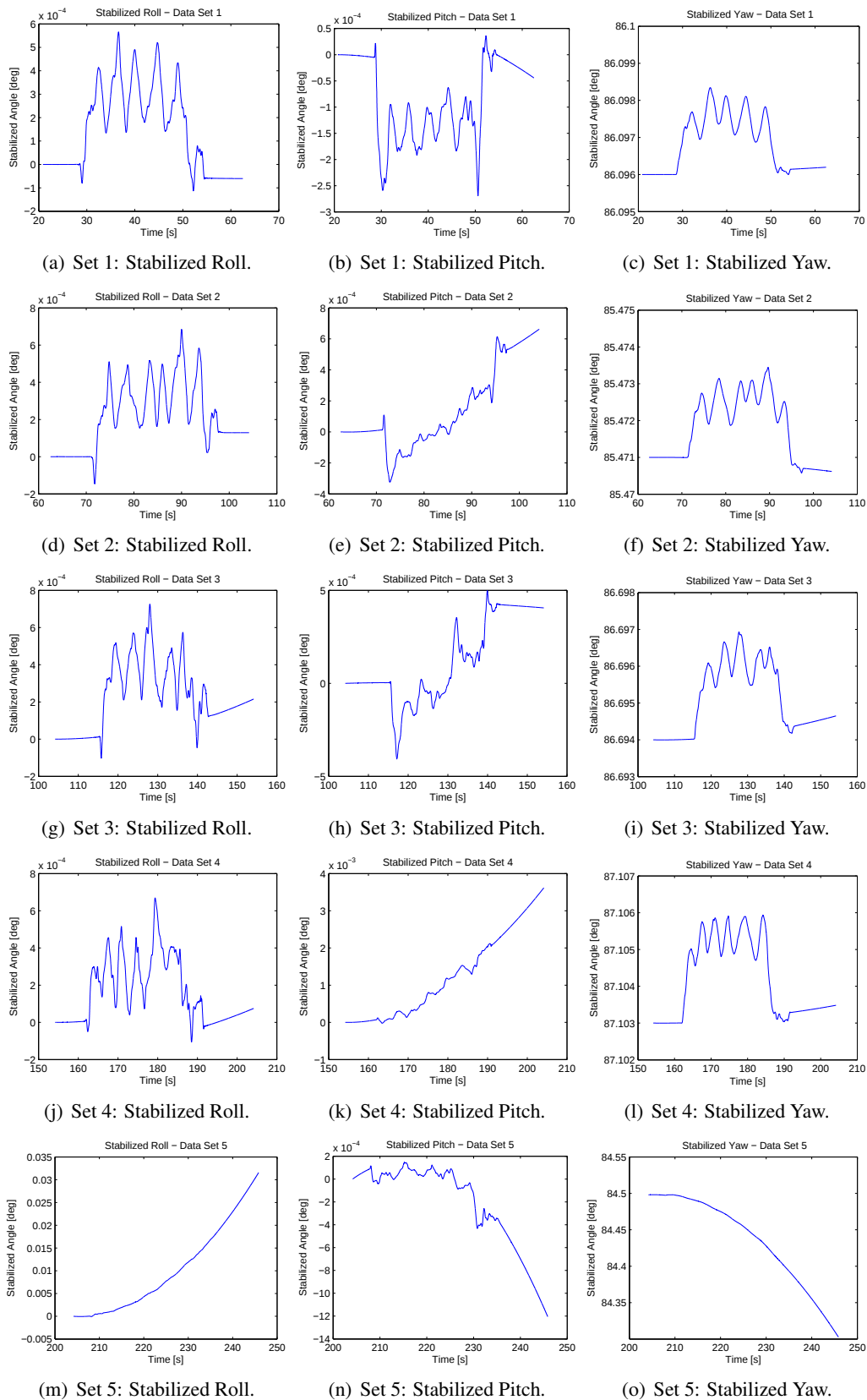
Figure 122: Stabilized attitude angles (roll, pitch, yaw) after bias and trend removal.
