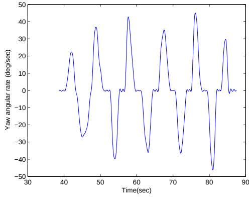
Figure 49: Yaw angular rate of nonlinear motion of handheld UXO sensor.
