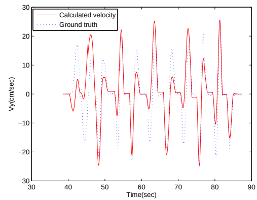
Figure 59: Calculated velocity along Y orientation based on raw acceleration. Zero velocity points are accurately determined. Sweeping motion.
