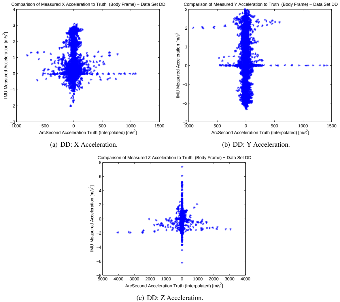
Figure 106: Comparisons of true and measured accelerations (in IMU body frame) for data set 'DD'.
