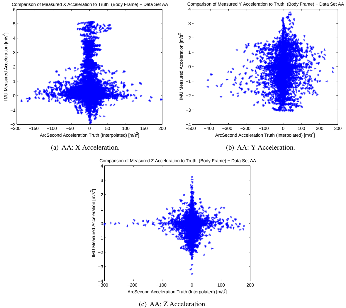
Figure 103: Comparisons of true and measured accelerations (in IMU body frame) for data set 'AA'.
