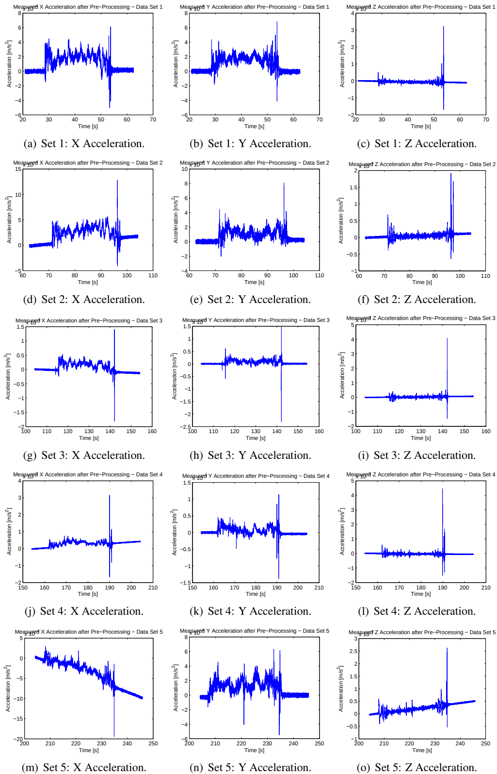
Figure 118: Measured accelerations after pre-processing.
