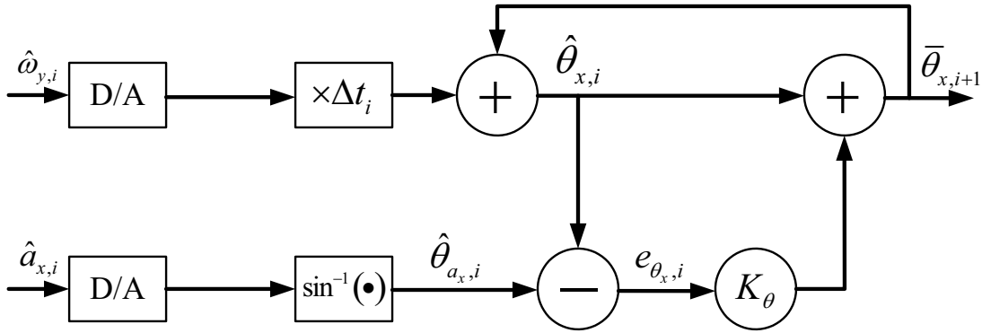
Figure 21: Iterative integration correction algorithm for pitch angle calculation.
