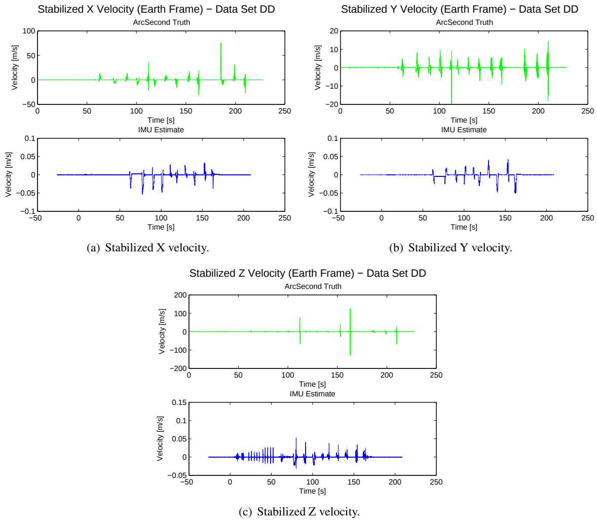
Figure 98: Stabilized velocities (in Earth frame) and comparison to ground truth for data set 'DD'.
