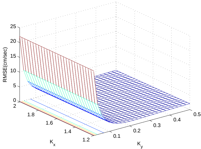
Figure 25: Root of mean square error versus gains K_x and K_y for calculating position of hand-held UXO sensor system along X orientation.
