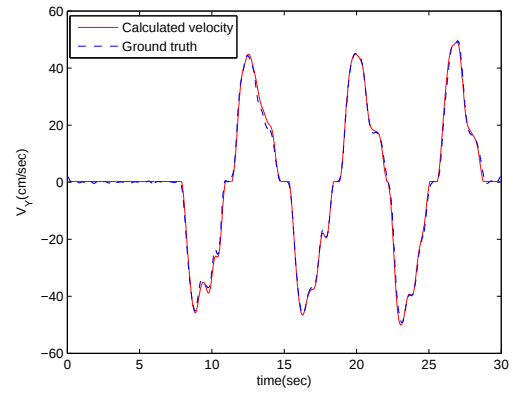
Figure 73: Calculated velocity along Y orientation based on estimated acceleration. Linear motion.
