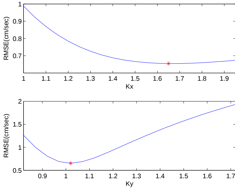
Figure 28: Top panel: Root of mean square error versus gain K_x for calculating position of hand-held UXO sensor system along Y orientation. Bottom panel: Root of mean square error versus gain K_y for calculating position of hand-held UXO sensor system along Y orientation.
