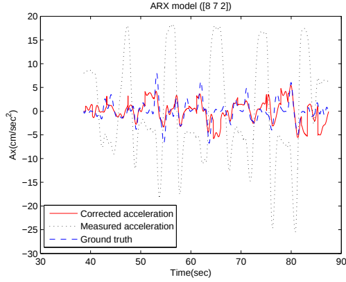
Figure 79: Estimated acceleration along x orientation. a_{meas} is input and \frac{d}{dt}a_{true} is output. na = 8 , nb = 7 and nk = 2 .
