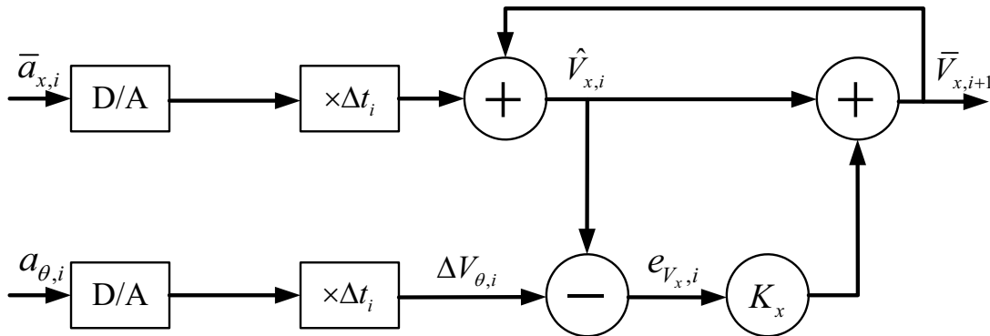
Figure 24: Iterative integration correction algorithm for velocity stabilization along x axes.
