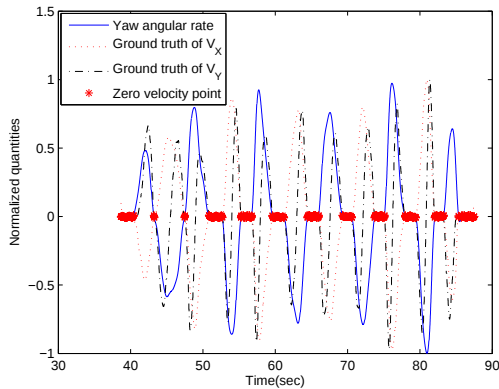
Figure 47: Comparison of zero velocity points in X and Y directions. Sweeping motion.
