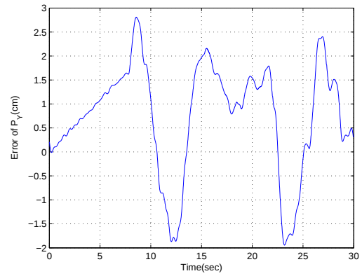
Figure 77: Calculated position error along Y orientation based on estimated acceleration. Linear motion.
