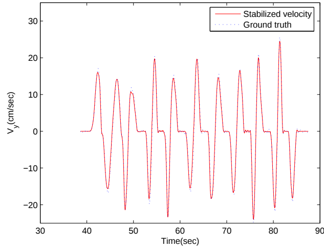
Figure 43: Stabilized velocity along Y axes with adaptive optimal gains K_x^{(Y),s} = 0.5000 , K_x^{(Y),f} = 1.9900 , K_y^{(Y),s} = 1.9900 and K_y^{(Y),f} = 1.9000 .
