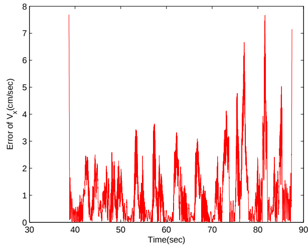
Figure 32: Calculated error of stabilized velocity along X orientation with fixed optimal gains K_x = 1.9800 and K_y = 0.2800 .
