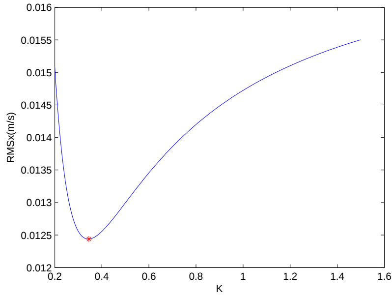
Figure 7: Example illustrating choosing K_x .
