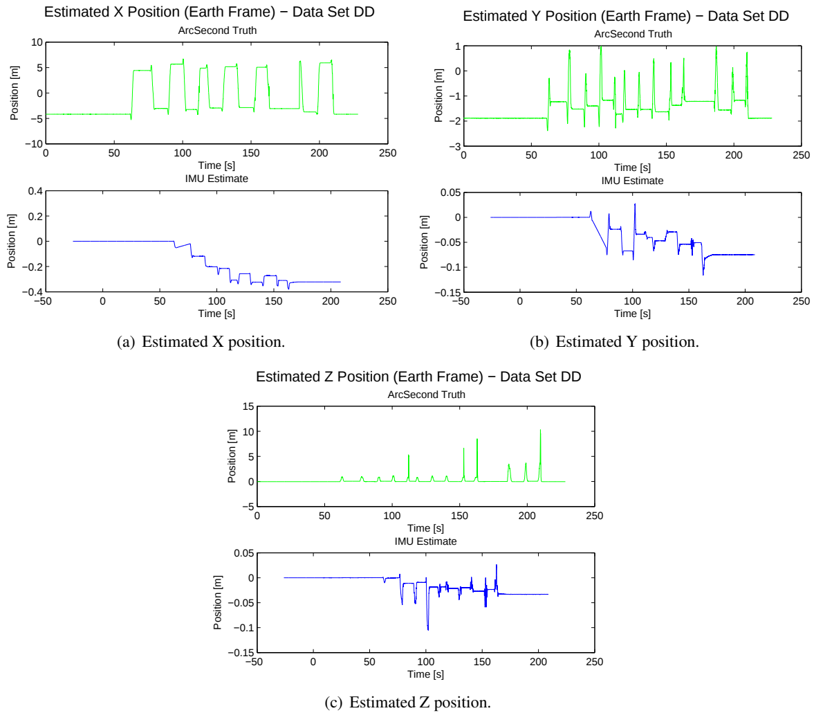
Figure 102: Estimated positions (in Earth frame) and comparison to ground truth for data set 'DD'.
