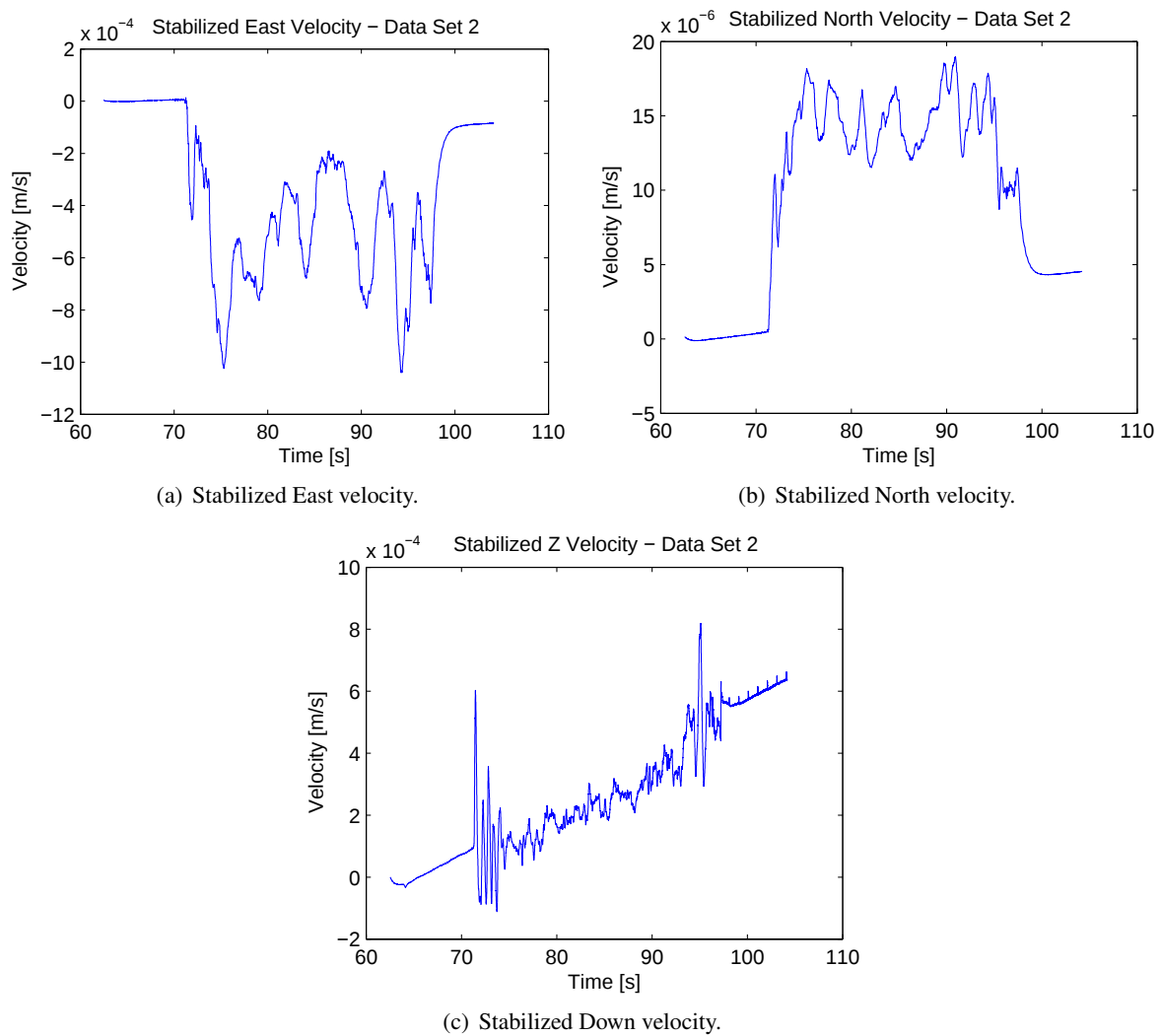
Figure 129: Stabilized velocities (in Earth frame) for data set 2, afternoon collection.
