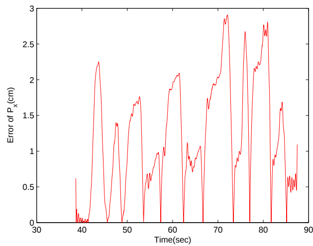
Figure 34: Calculated error of stabilized position along X axes with fixed optimal gains K_x = 1.9800 and K_y = 0.2800 .
