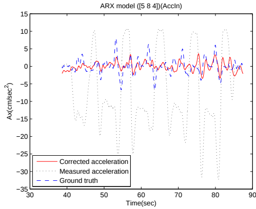
Figure 81: Estimated acceleration along x orientation. a_{meas} is input and a_{true} is output. na = 6 , nb = 1 and nk = 1 .
