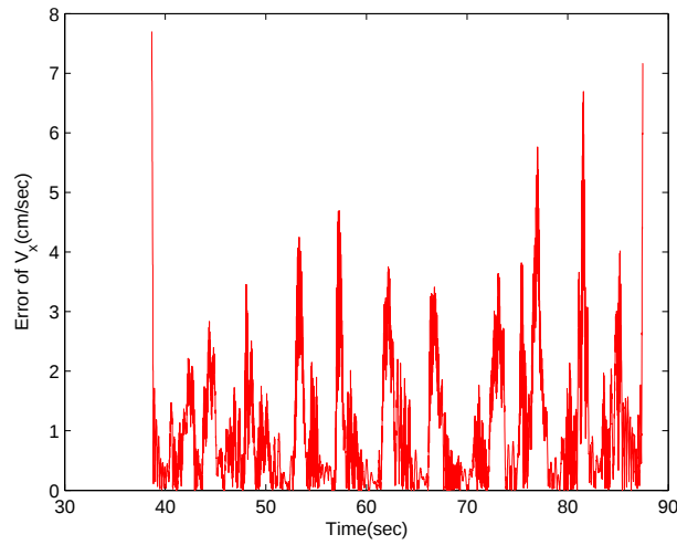
Figure 40: Calculated error of stabilized velocity along X axes with adaptive optimal gains K_x^{(X),s} = 1.9950 , K_x^{(X),f} = 1.5800 , K_y^{(X),s} = 0.0950 and K_y^{(X),f} = 0.2600 .
