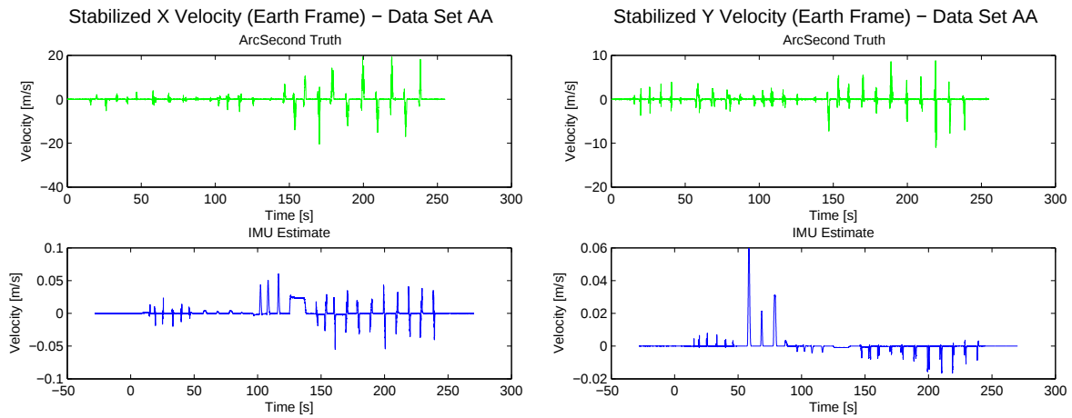
(a) Stabilized X velocity.
