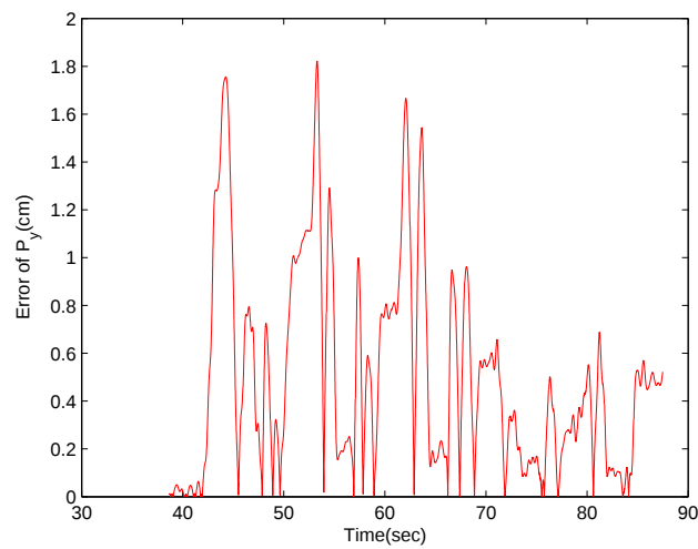
Figure 38: Calculated error of stabilized position along Y axes with fixed optimal gains K_x = 1.9000 and K_y = 1.8500 .
