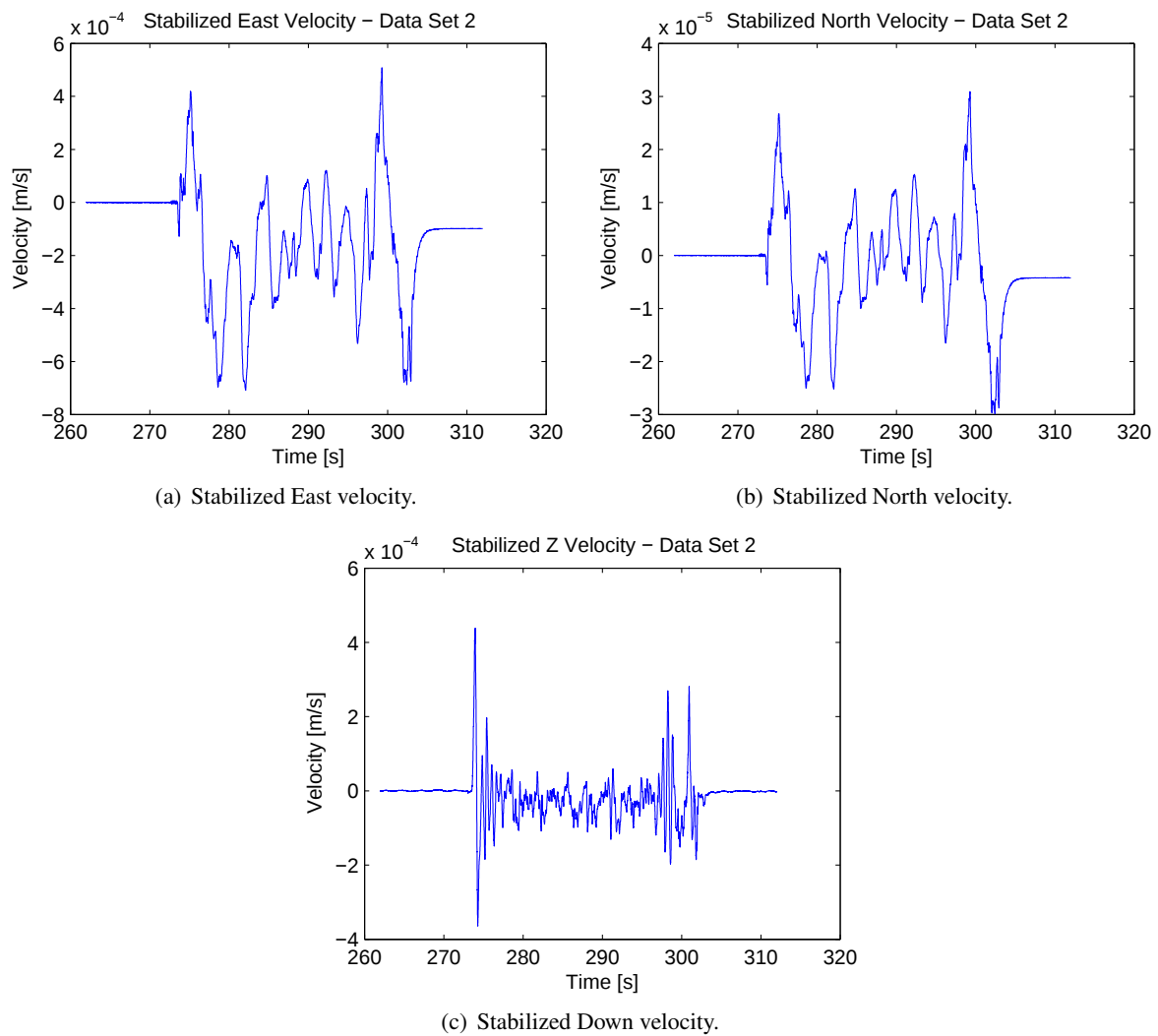
Figure 124: Stabilized velocities (in Earth frame) for data set 2, morning collection.
