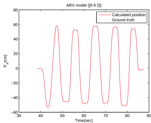
Figure 60: Position along X orientation calculated from the estimated velocity by direct integration method. Sweeping motion.
