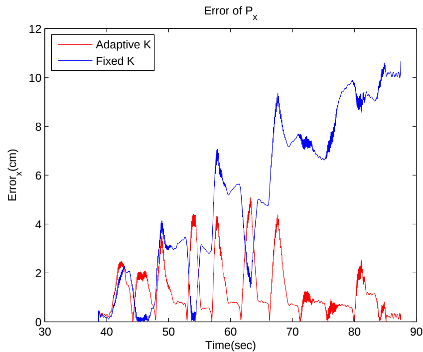
Figure 13: Errors in stabilized positions along the x axis with adaptive K and fixed K algorithms.
