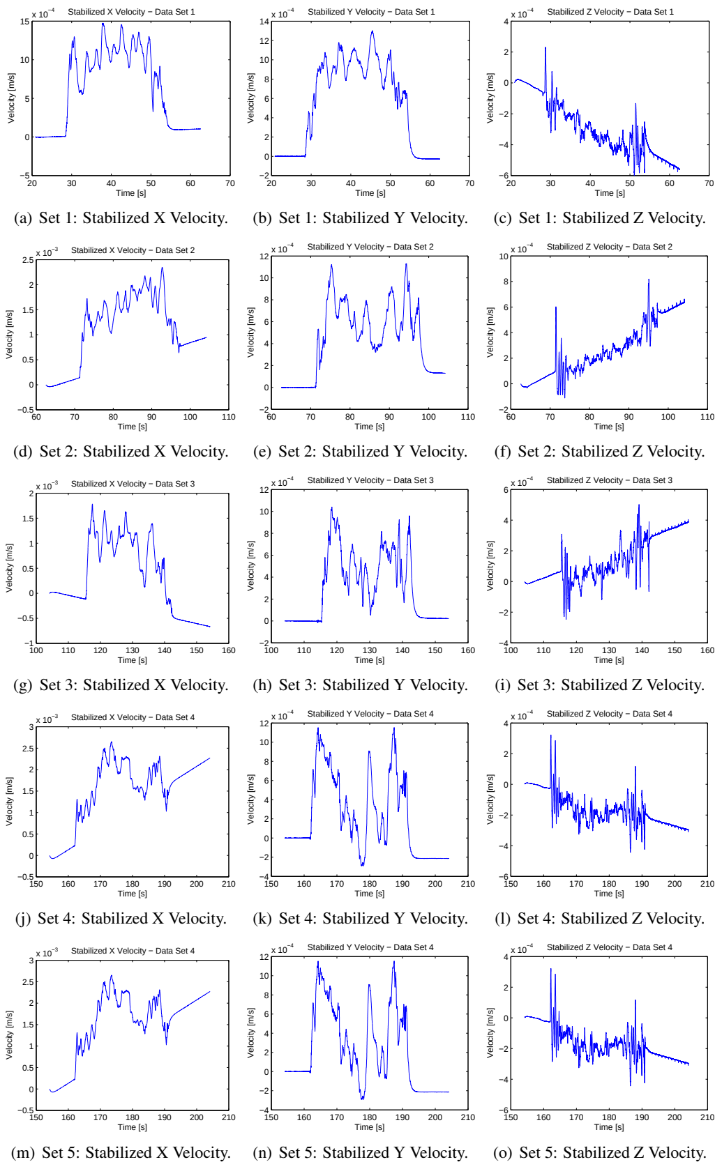
Figure 120: Stabilized velocities after bias and trend removal.
