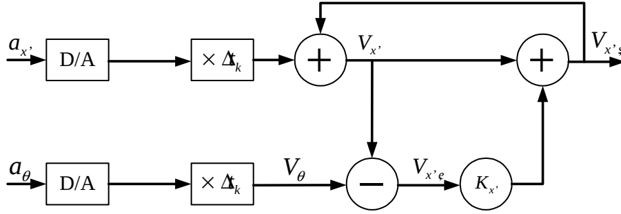
Figure 4: Iterative integration correction algorithm for velocity stabilization along the x' axis.
