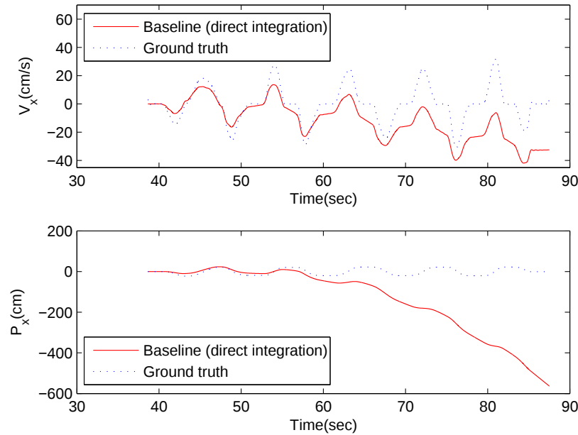
Figure 29: Calculated velocity and position along X orientation directly using the conventional integration method.
