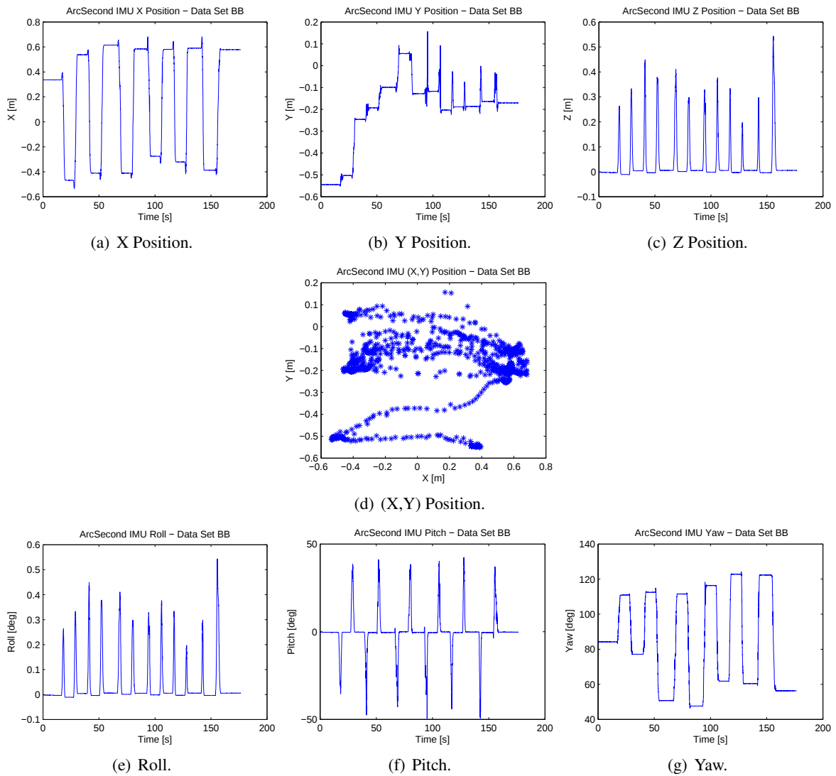
Figure 89: ArcSecond ground truth for data set 'BB'.
