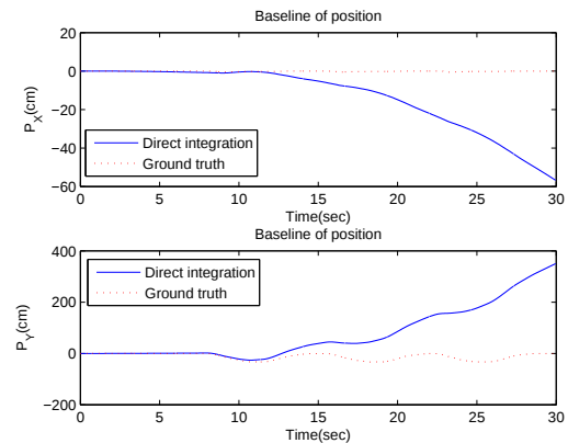
Figure 71: Position calculated from raw acceleration by the conventional numerical integration. Linear motion.
