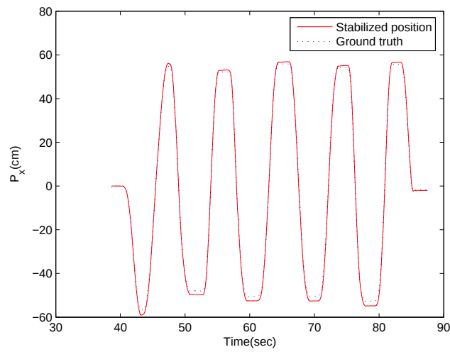
Figure 33: Stabilized position along X axes with fixed optimal gains K_x = 1.9800 and K_y = 0.2800 .
