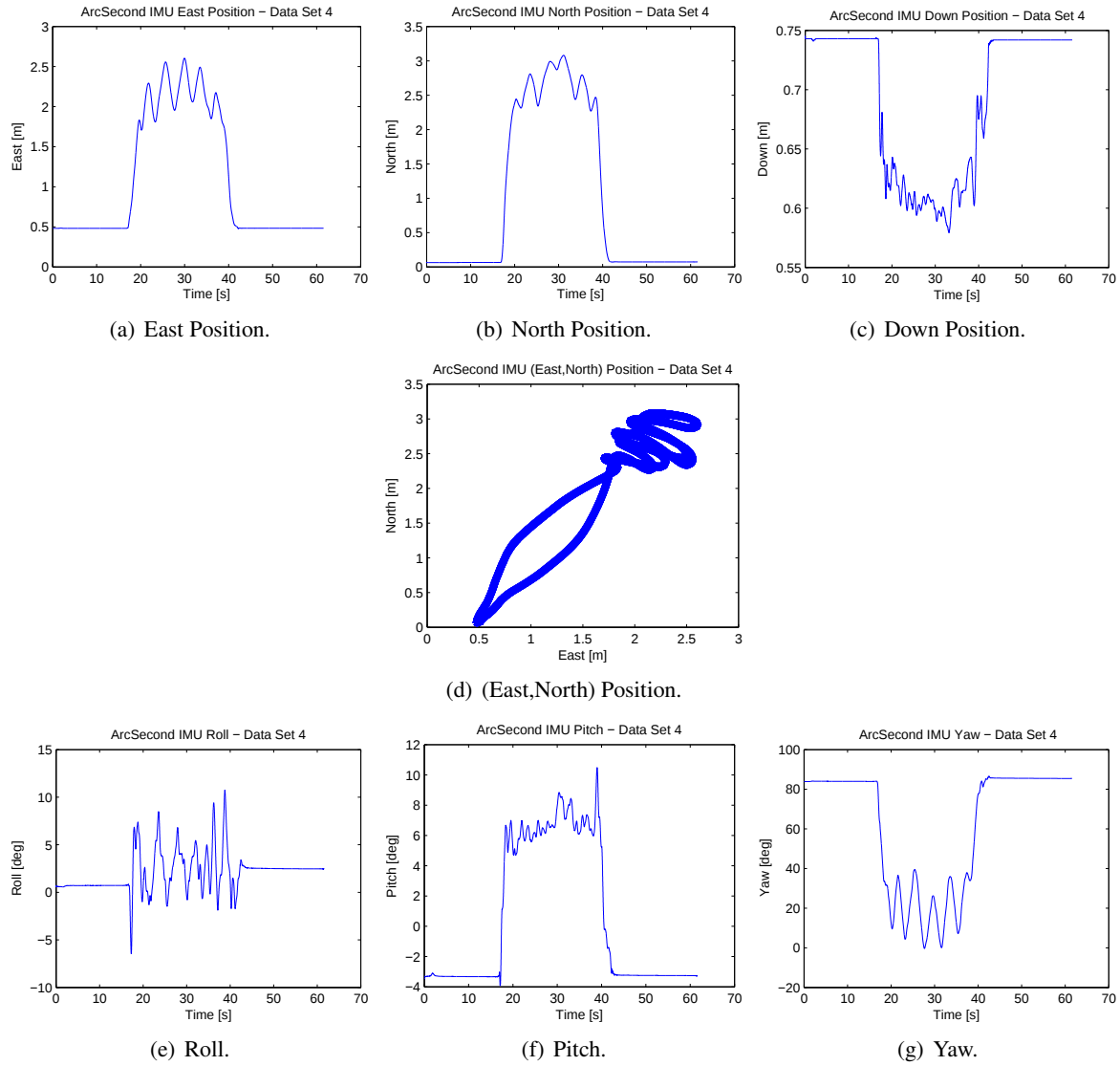
Figure 110: ArcSecond ground truth for data set 4 from the morning collection.
