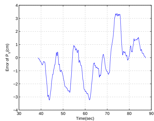
Figure 65: Position error along Y orientation calculated from the estimated velocity by direct integration method. Sweeping motion.
