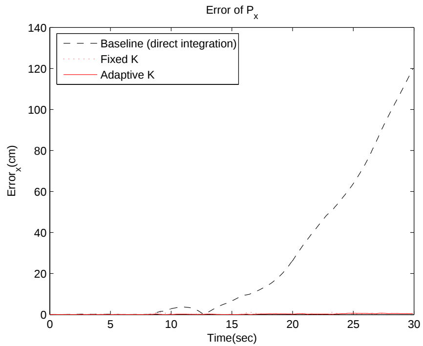
Figure 19: Estimation error of the position along the x axis based on the linear data.
