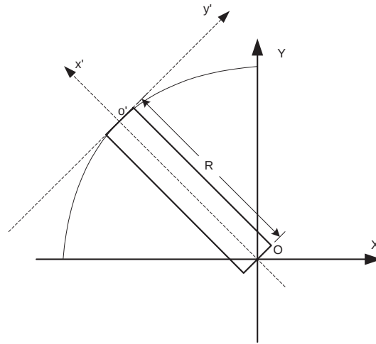
Figure 1: Body frame and earth frame geometry. (X, Y) represent the earth frame coordinates and (x', y') represent the body frame coordinates.
