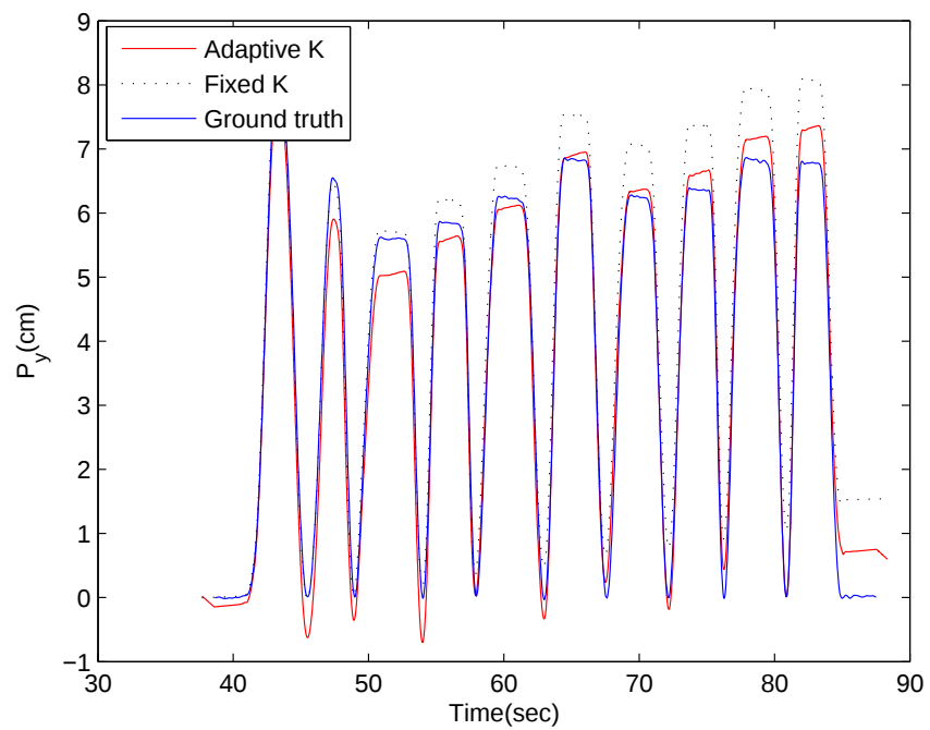
Figure 12: Stabilized positions along the y axis with adaptive K and fixed K algorithms.
