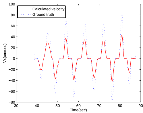
Figure 58: Calculated velocity along X orientation based on raw acceleration. Zero velocity points are accurately determined. Sweeping motion.
