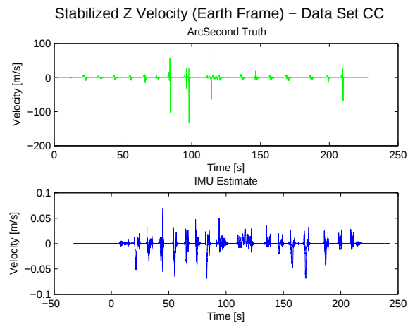
(c) Stabilized Z velocity.
