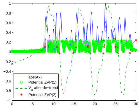
Figure 68: Searching for zero velocity points by relying on acceleration in linear motion. The zero velocity points are the green circle points that are between the red star points.
