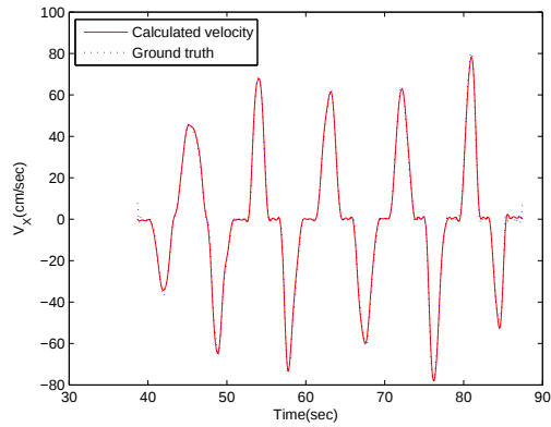
Figure 56: Calculated velocity along X orientation based on estimated acceleration. Sweeping motion.
