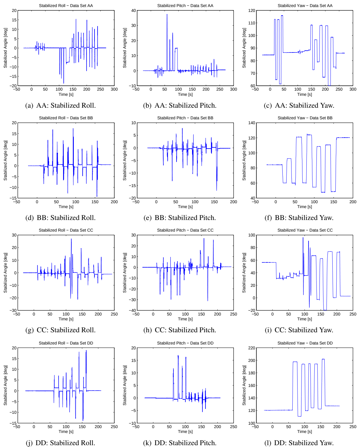
Figure 94: Stabilized attitude angles (roll, pitch, yaw) after bias and trend removal.
