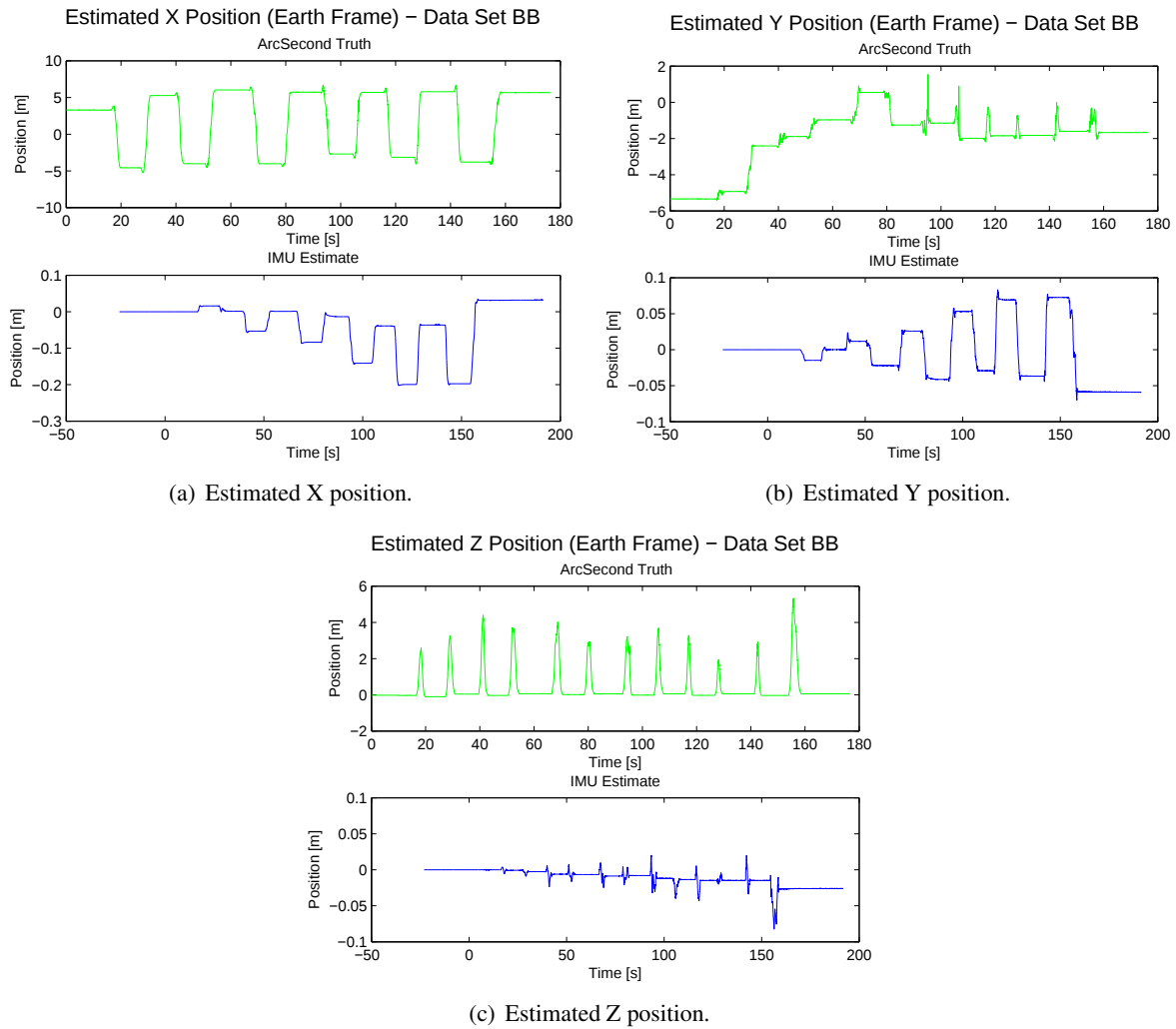
Figure 100: Estimated positions (in Earth frame) and comparison to ground truth for data set 'BB'.
