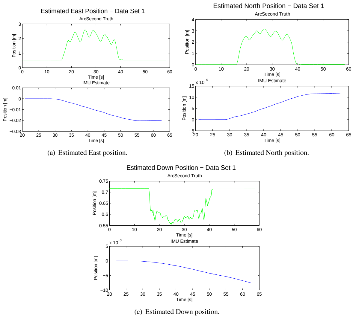
Figure 138: Estimated positions (in Earth frame) and comparison to ground truth for data set 1, afternoon collection.
