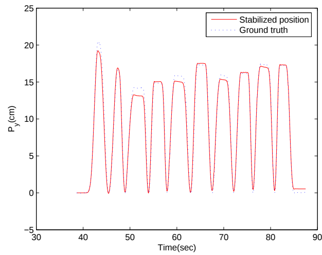
Figure 37: Stabilized position along Y axes with fixed optimal gains K_x = 1.9000 and K_y = 1.8500 .
