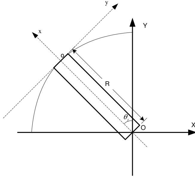
Figure 22: Geometry of earth frame and body frame. xoy is the coordinate system of the body frame and XOY is the coordinate system of the earth frame.
