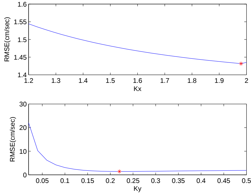
Figure 26: Top panel: Root of mean square error versus gain K_x for calculating position of hand-held UXO sensor system along X orientation. Bottom panel: Root of mean square error versus gain K_y for calculating position of hand-held UXO sensor system along X orientation.
