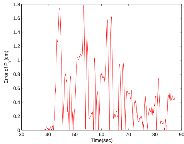
Figure 46: Calculated error of stabilized position along Y axes with adaptive optimal gains K_x^{(Y),s} = 0.5000 , K_x^{(Y),f} = 1.9900 , K_y^{(Y),s} = 1.9900 and K_y^{(Y),f} = 1.9000 .
