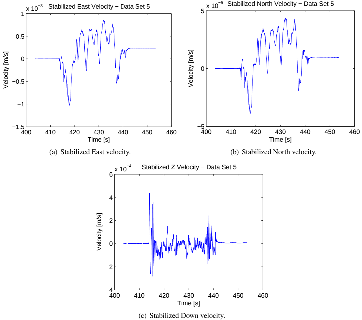
Figure 127: Stabilized velocities (in Earth frame) for data set 5, morning collection.
