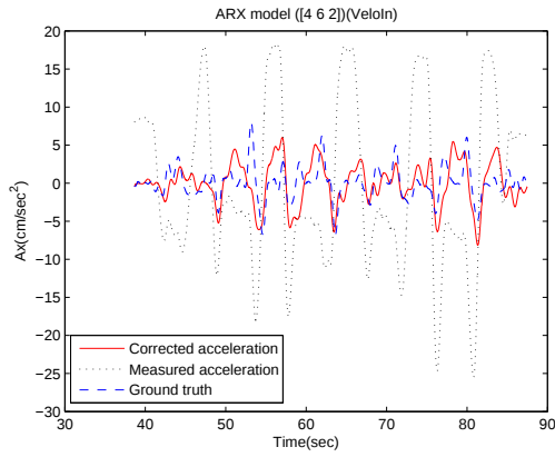
Figure 83: Estimated acceleration along x orientation. a_{meas} is input and v_{true} is output. na = 4 , nb = 6 and nk = 2 .
