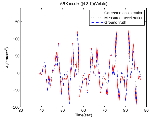
Figure 84: Estimated acceleration along y orientation. a_{meas} is input and v_{true} is output. na = 4 , nb = 3 and nk = 1 .
