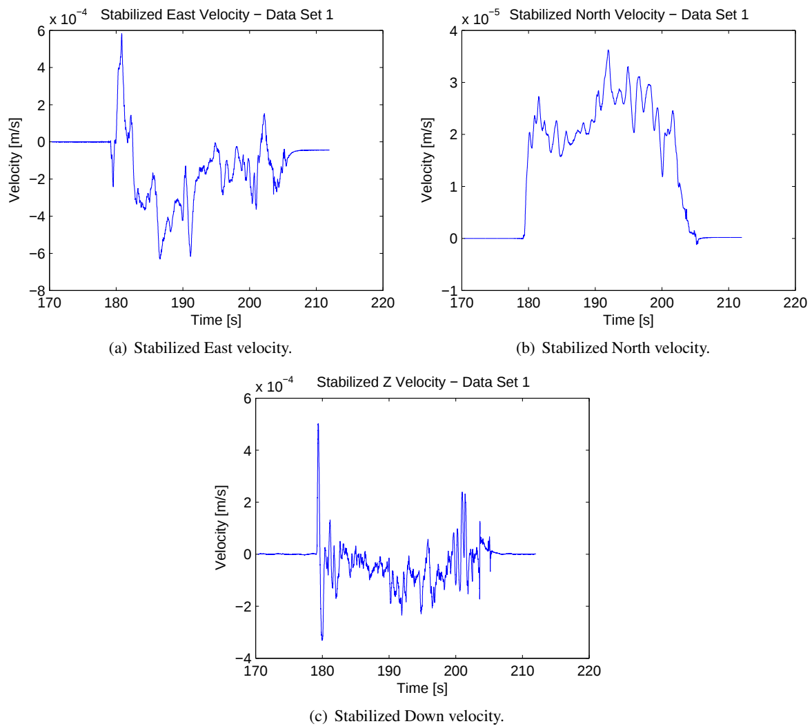
Figure 123: Stabilized velocities (in Earth frame) for data set 1, morning collection.
