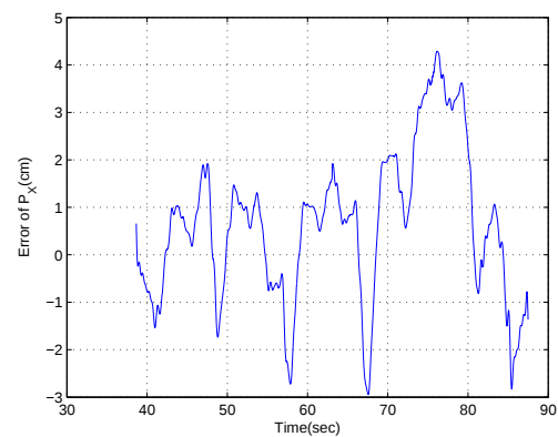
Figure 61: Position error along X orientation calculated from the estimated velocity by direct integration method. Sweeping motion.
