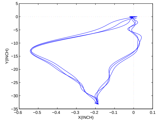
Figure 69: Example of zero-position updates for linear motion. The solid lines are the actual track of the sensor. The dash lines are the coordinate axes of the earth frame.
