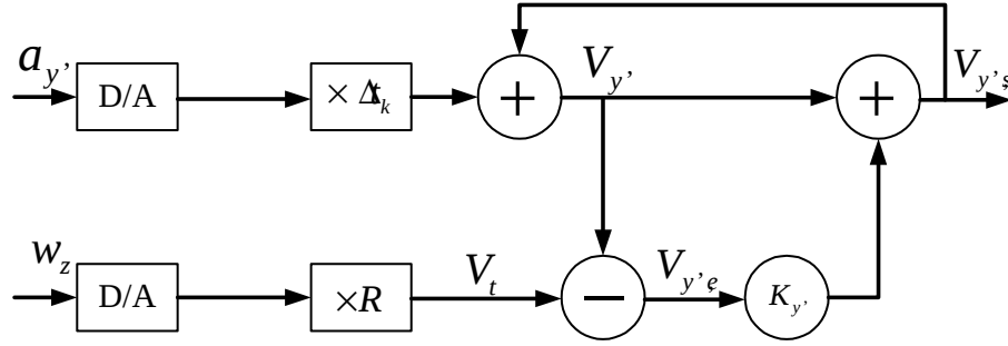
Figure 3: Iterative integration correction algorithm for velocity stabilization along the y' axis.
