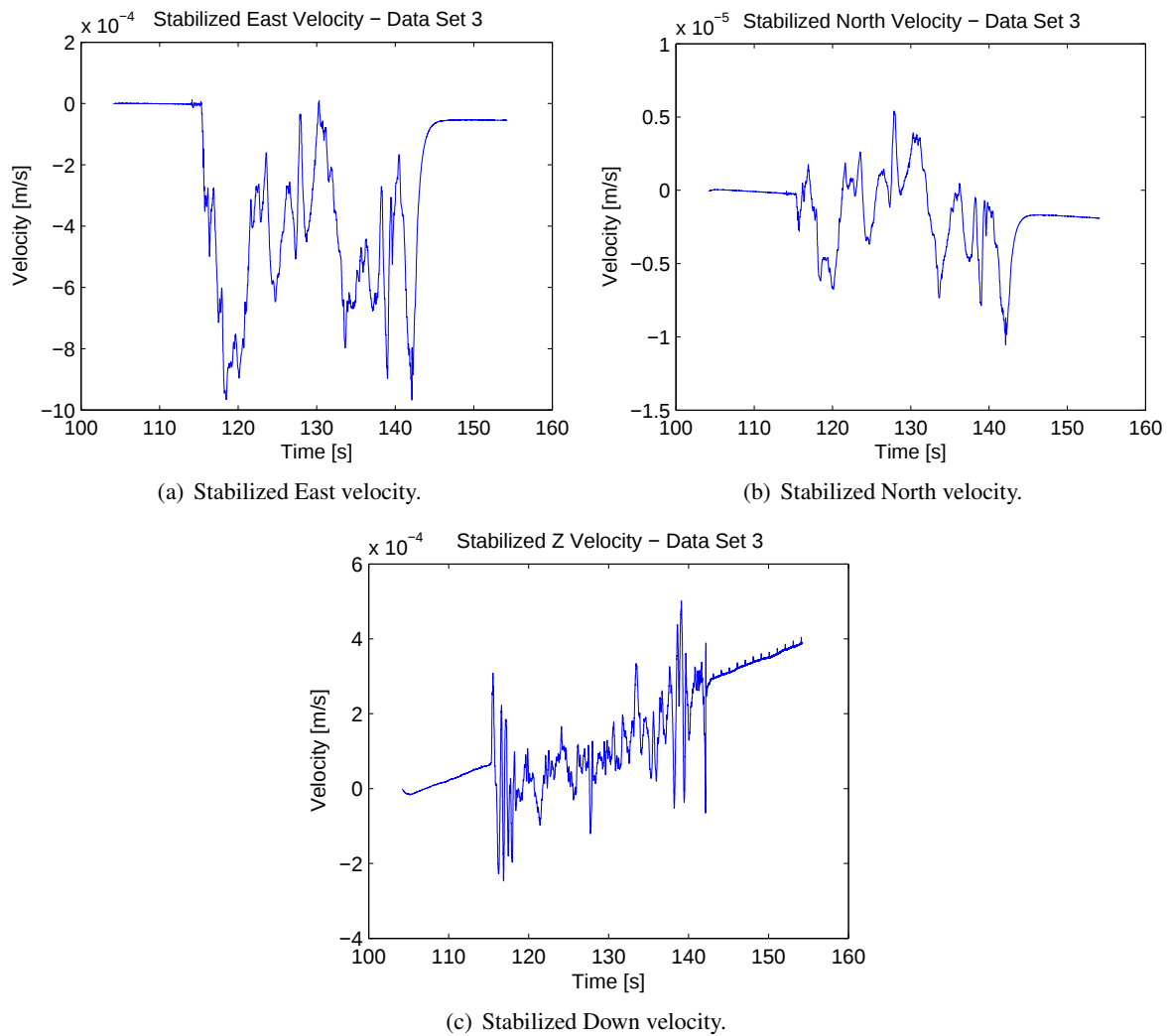
Figure 130: Stabilized velocities (in Earth frame) for data set 3, afternoon collection.
