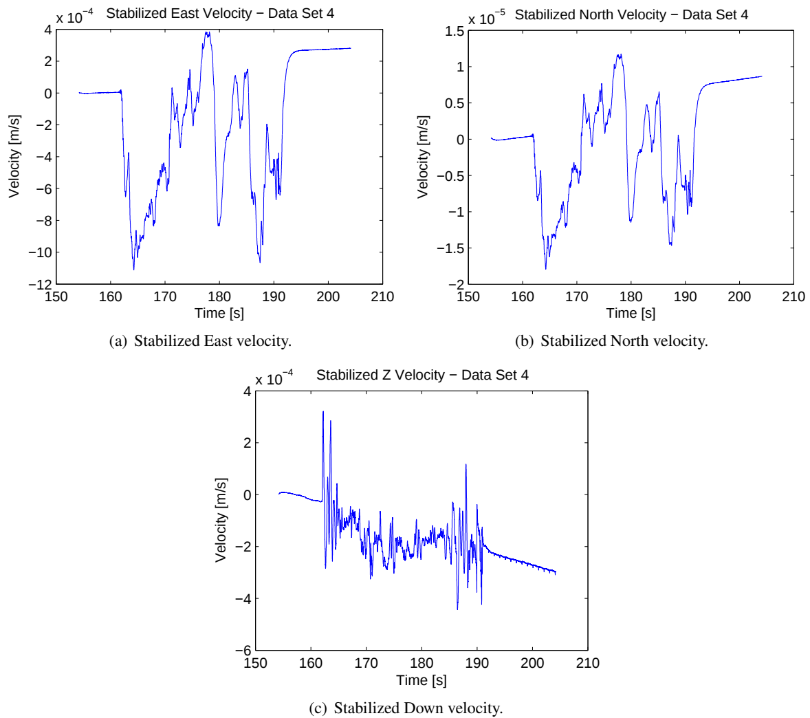
Figure 131: Stabilized velocities (in Earth frame) for data set 4, afternoon collection.
