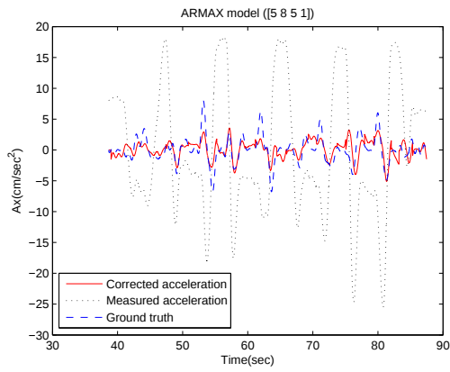
Figure 86: Estimated acceleration along x orientation. a_{meas} is input and \frac{d}{dt}a_{true} is output. na = 5 , nb = 8 , nc = 5 and nk = 1 .
