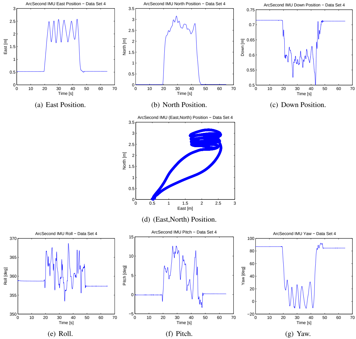
Figure 115: ArcSecond ground truth for data set 4 from the afternoon collection.
