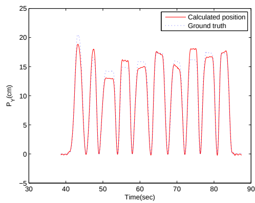
Figure 66: Position along Y orientation calculated from the estimated velocity by zero-position-update method. Sweeping motion.
