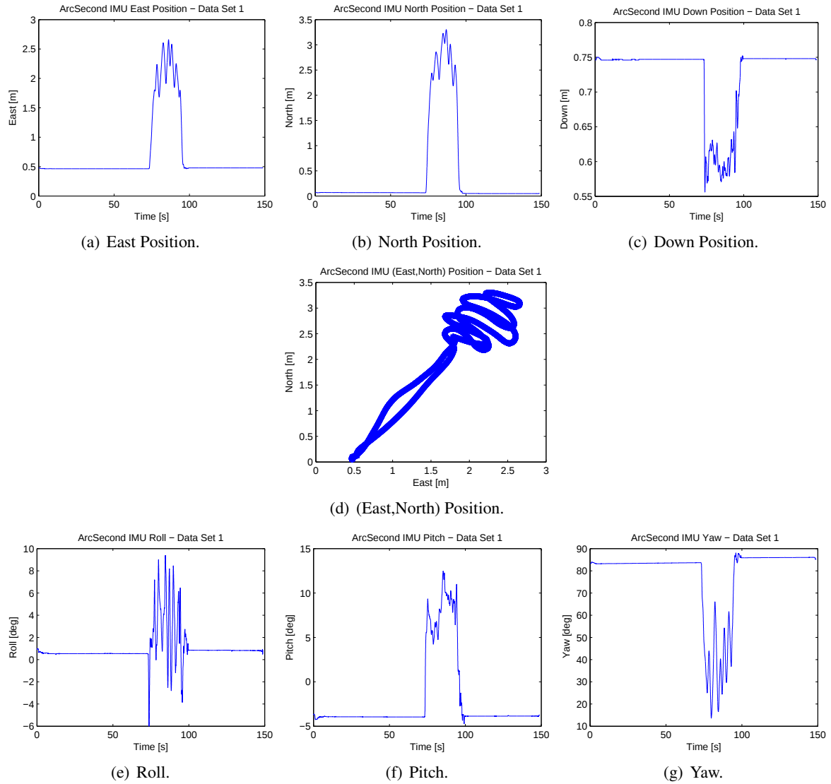
Figure 107: ArcSecond ground truth for data set 1 from the morning collection.
