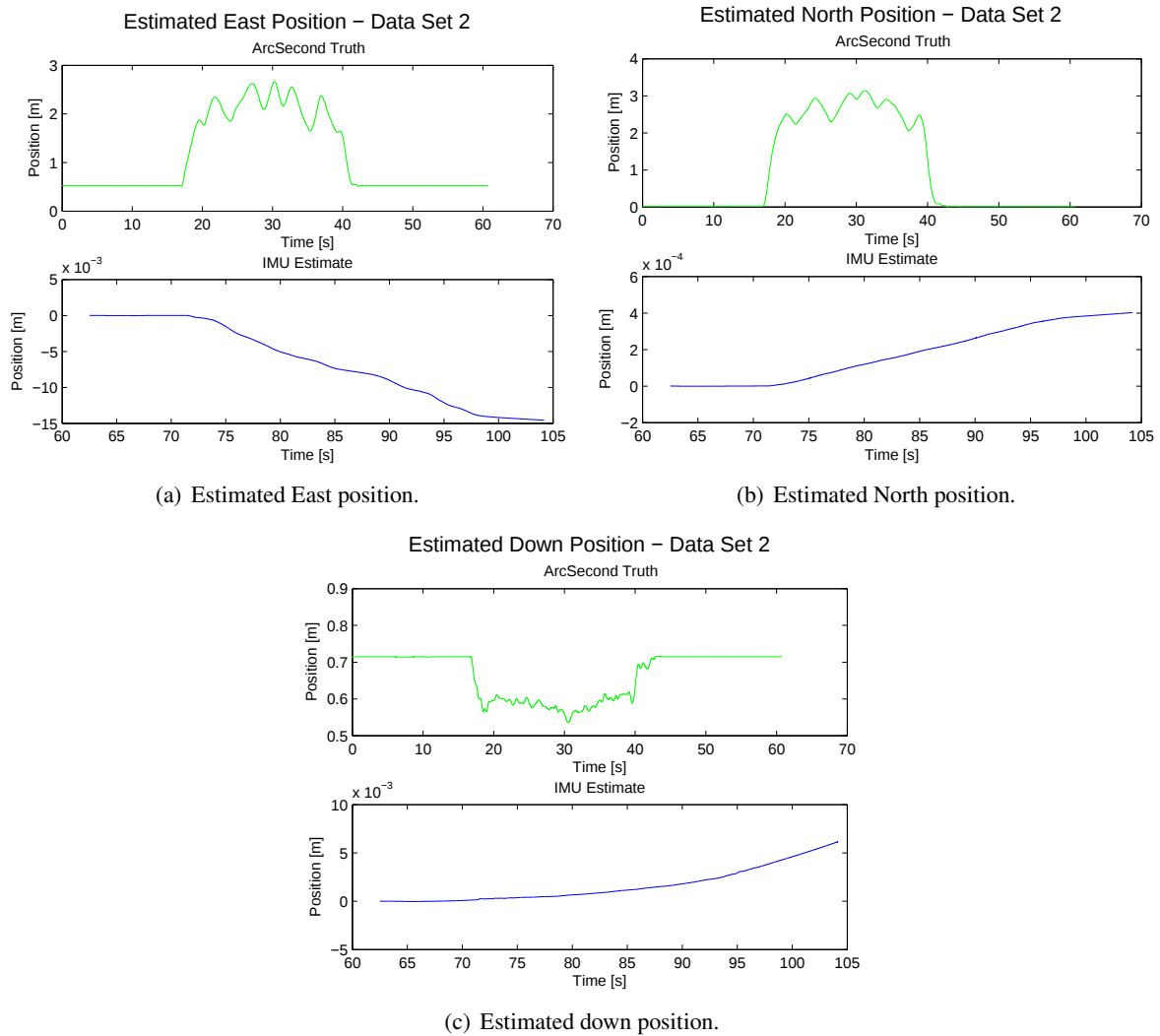
Figure 139: Estimated positions (in Earth frame) and comparison to ground truth for data set 2, afternoon collection.
