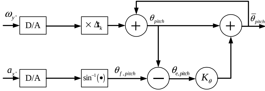
Figure 2: Iterative integration correction algorithm for pitch stabilization.
