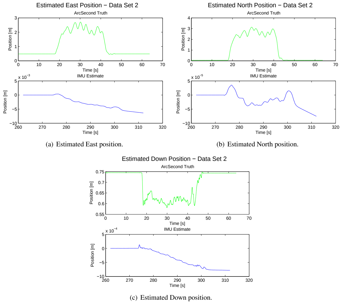
Figure 134: Estimated positions (in Earth frame) and comparison to ground truth for data set 2, morning collection.
