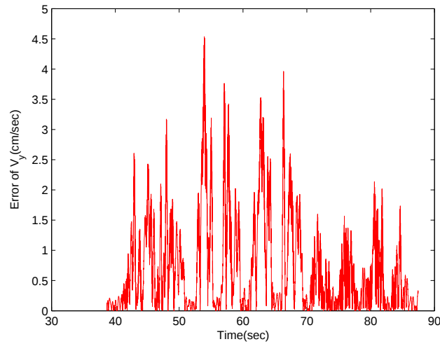
Figure 44: Calculated error of stabilized velocity along Y axes with adaptive optimal gains K_x^{(Y),s} = 0.5000 , K_x^{(Y),f} = 1.9900 , K_y^{(Y),s} = 1.9900 and K_y^{(Y),f} = 1.9000 .
