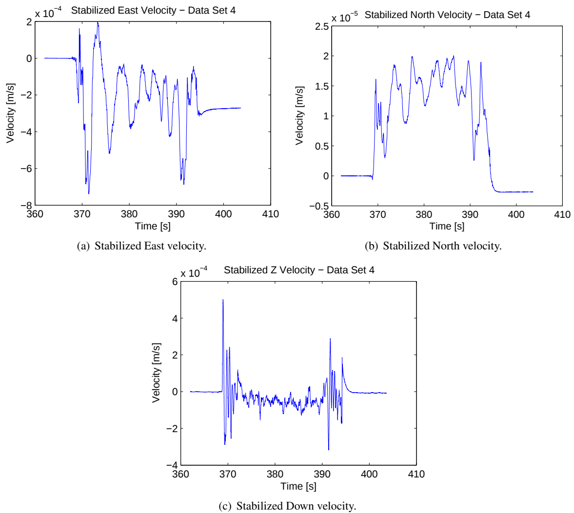
Figure 126: Stabilized velocities (in Earth frame) for data set 4, morning collection.
