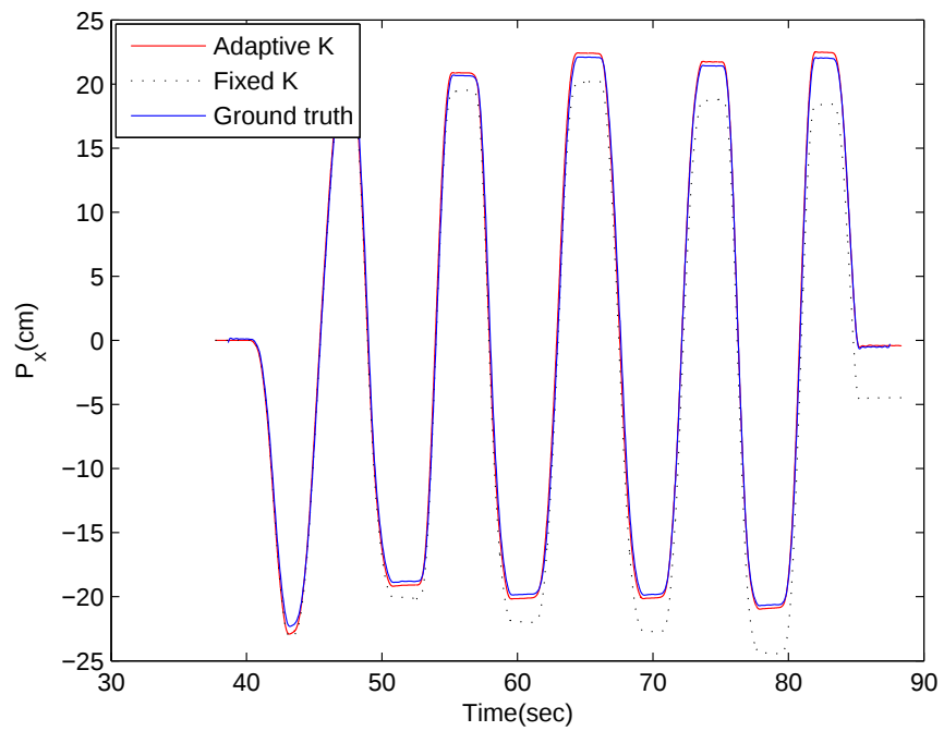
Figure 11: Stabilized positions along the x axis with adaptive K and fixed K algorithms.
