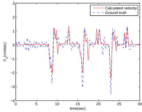
Figure 72: Calculated velocity along X orientation based on estimated acceleration. Linear motion.
