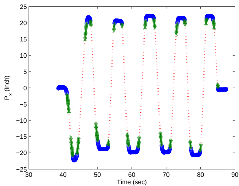
Figure 5: Example of the partition of the path along the x orientation.
