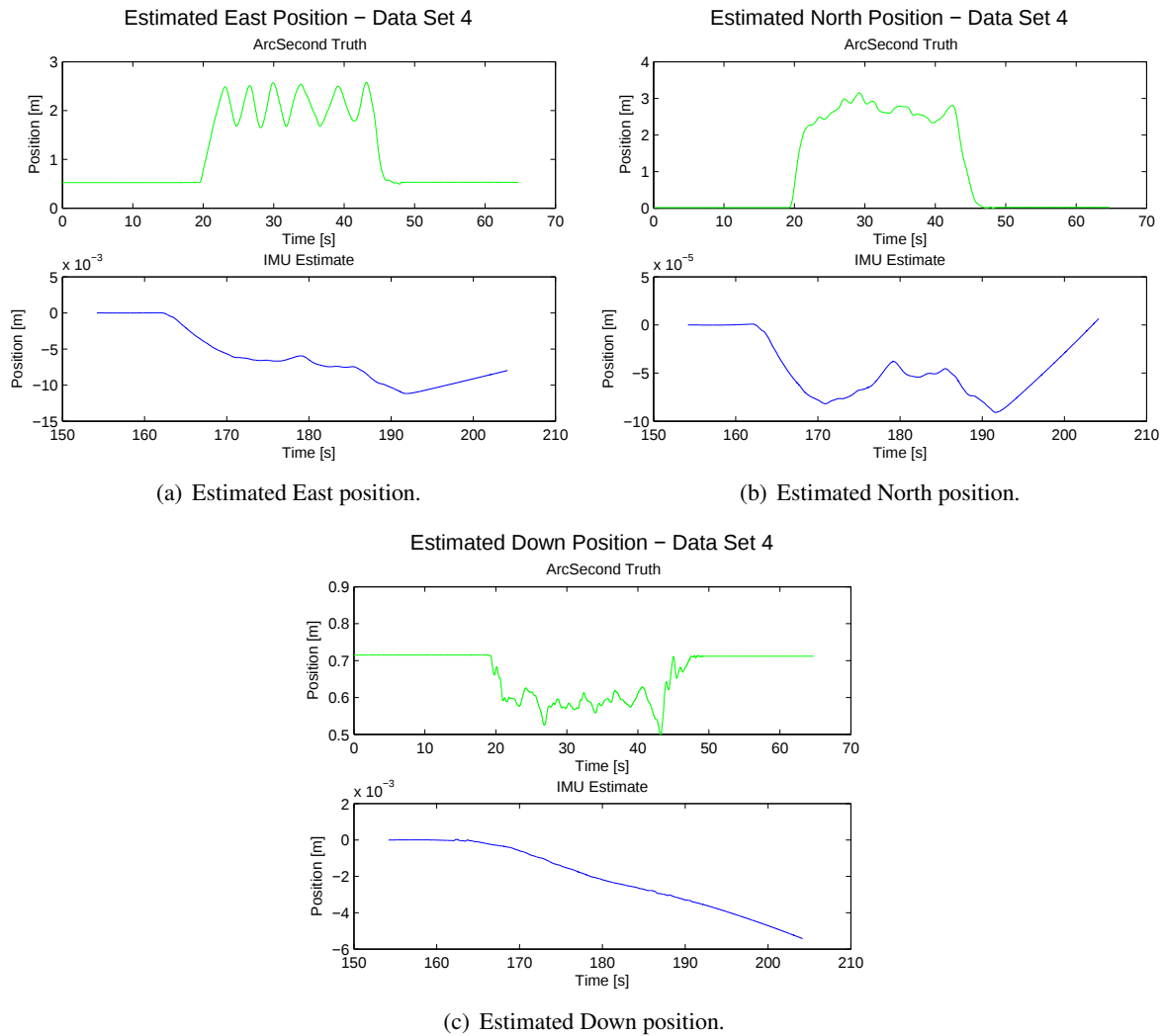
Figure 141: Estimated positions (in Earth frame) and comparison to ground truth for data set 4, afternoon collection.
