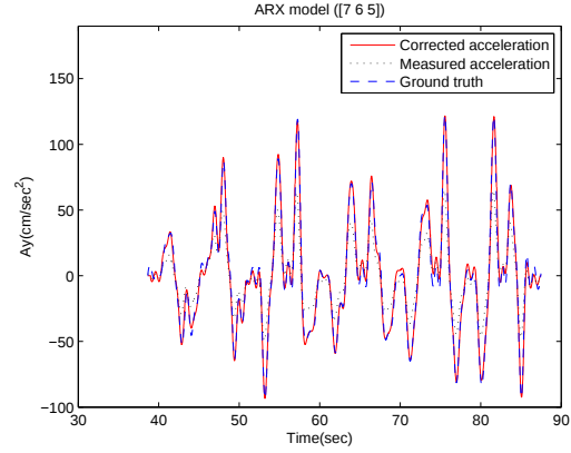
Figure 80: Estimated acceleration along y orientation. a_{meas} is input and \frac{d}{dt}a_{true} is output. na = 7 , nb = 6 and nk = 5 .
