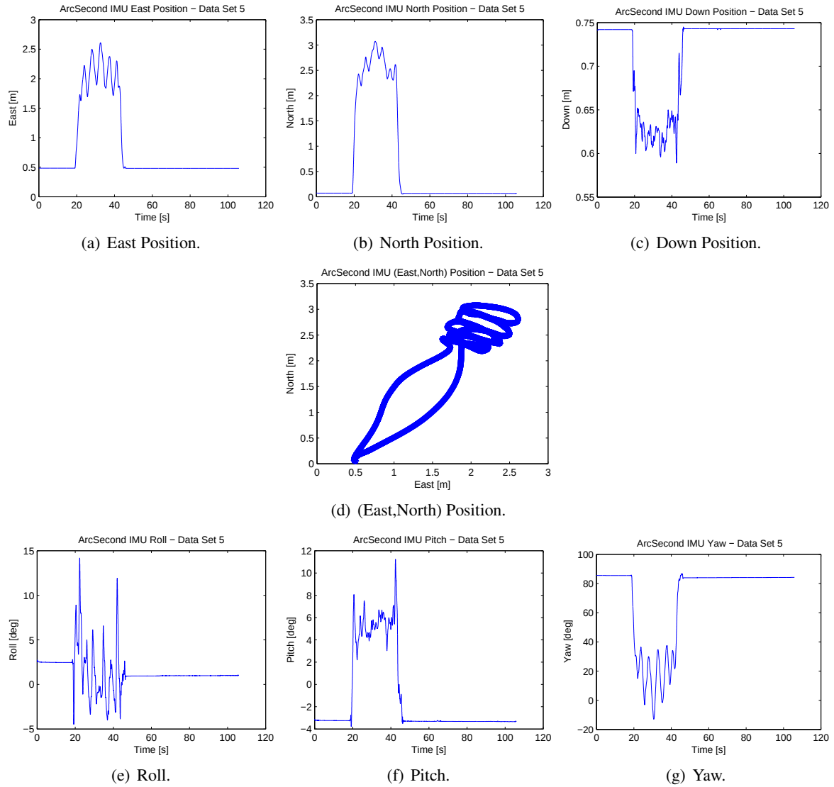
Figure 111: ArcSecond ground truth for data set 5 from the morning collection.
