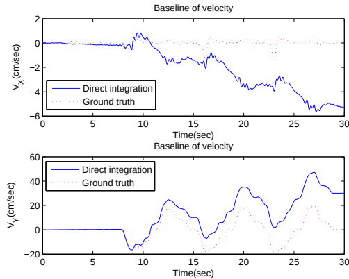
Figure 70: Velocity calculated from raw acceleration by the conventional numerical integration. Linear motion.
