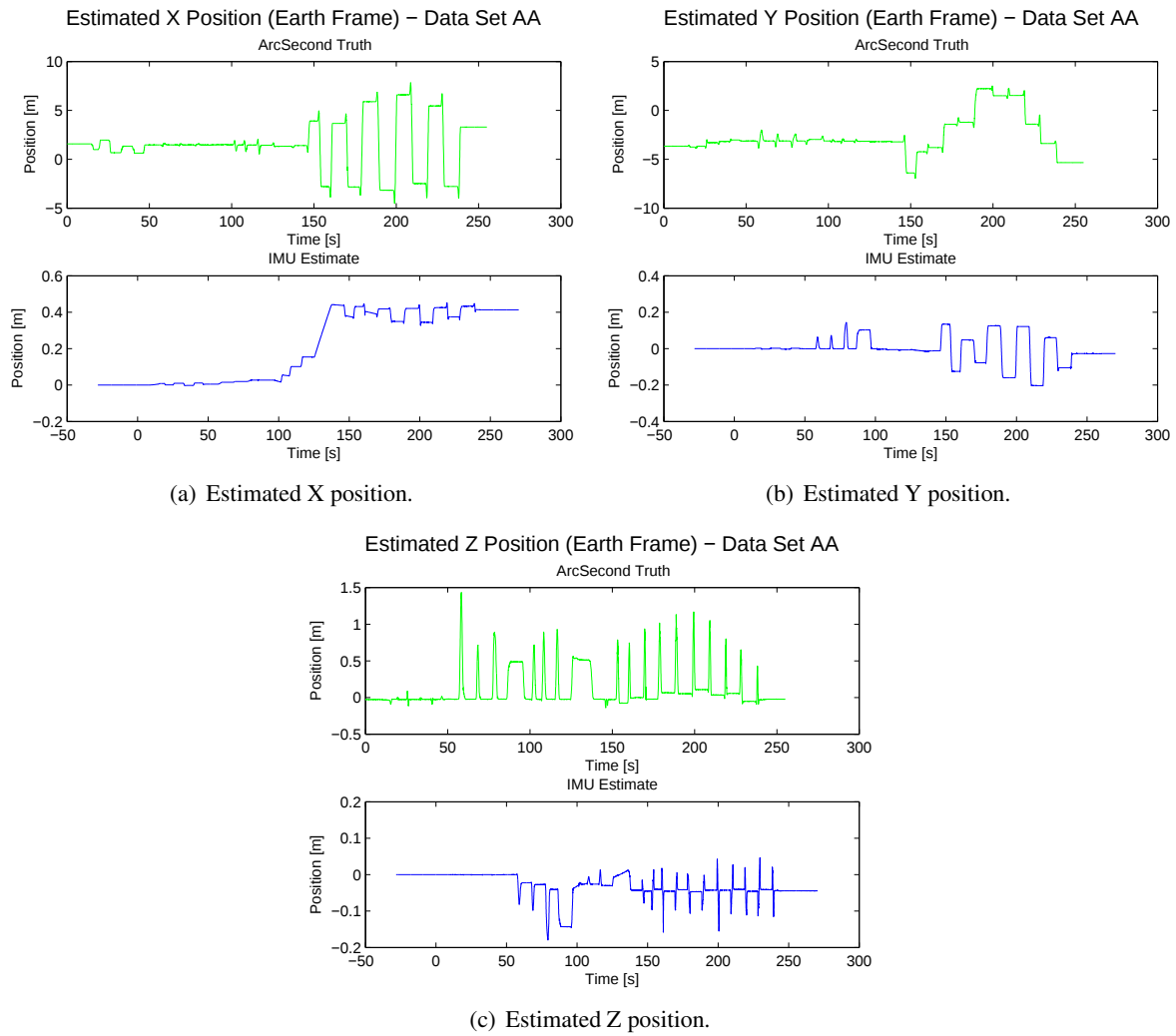
Figure 99: Estimated positions (in Earth frame) and comparison to ground truth for data set 'AA'.
