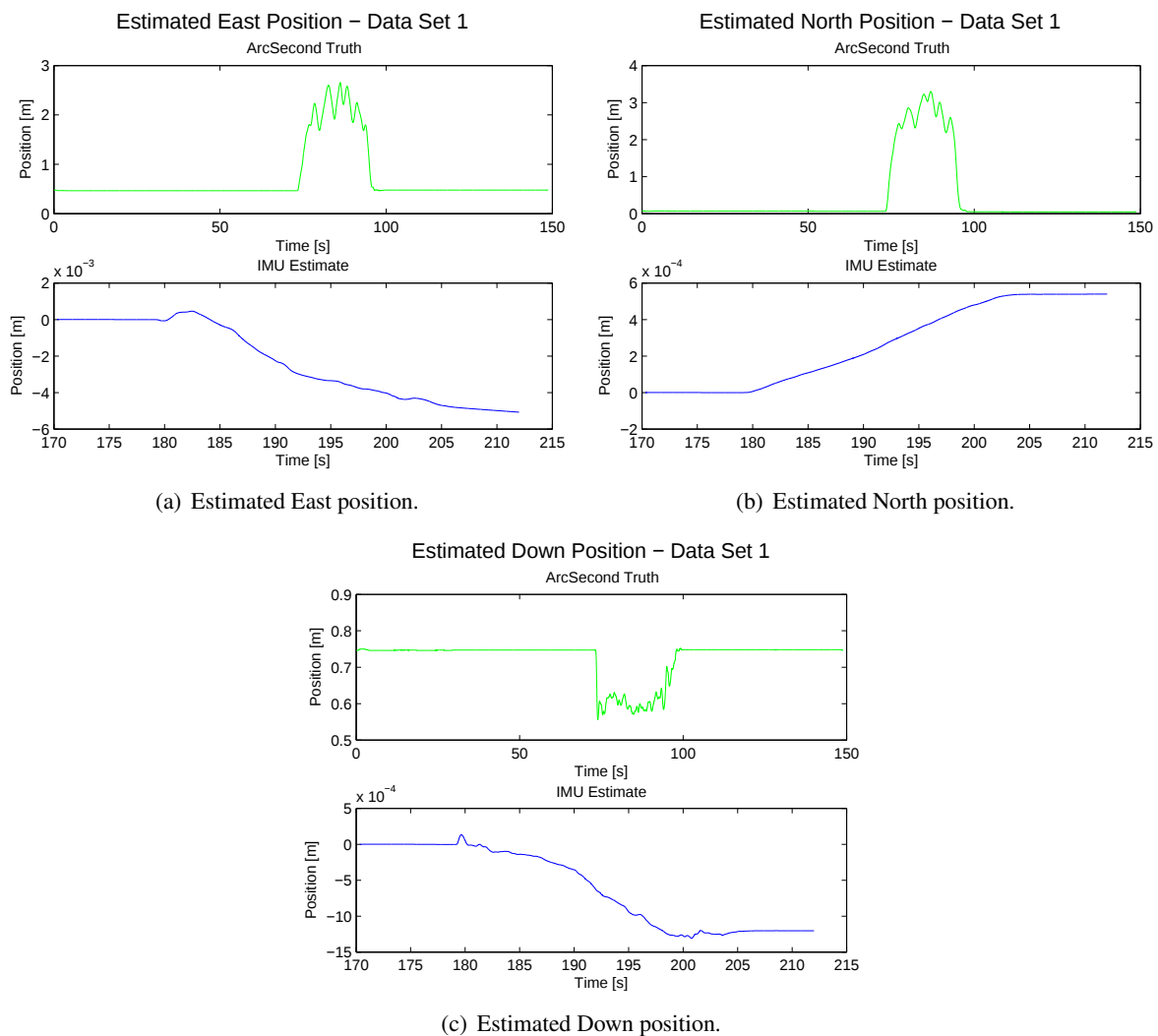
Figure 133: Estimated positions (in Earth frame) and comparison to ground truth for data set 1, morning collection.
