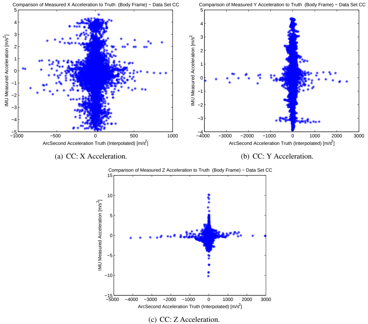
Figure 105: Comparisons of true and measured accelerations (in IMU body frame) for data set 'CC'.
