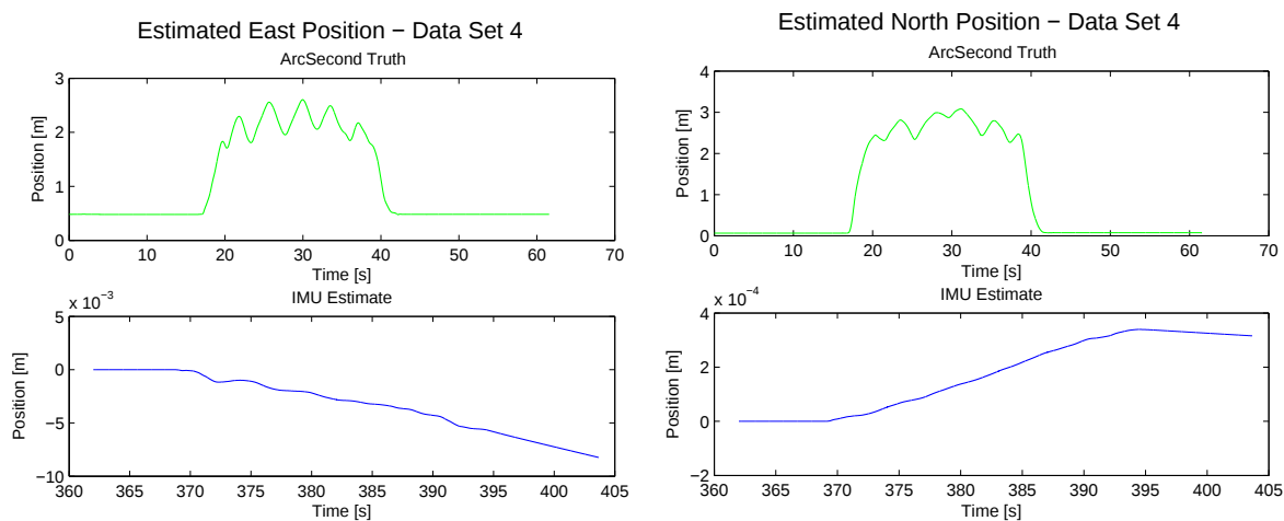
(a) Estimated East position.
