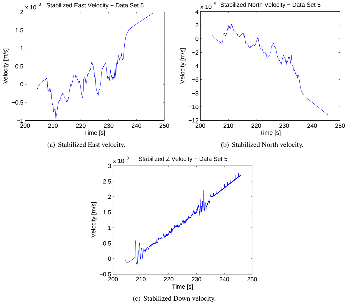
Figure 132: Stabilized velocities (in Earth frame) for data set 5, afternoon collection.
