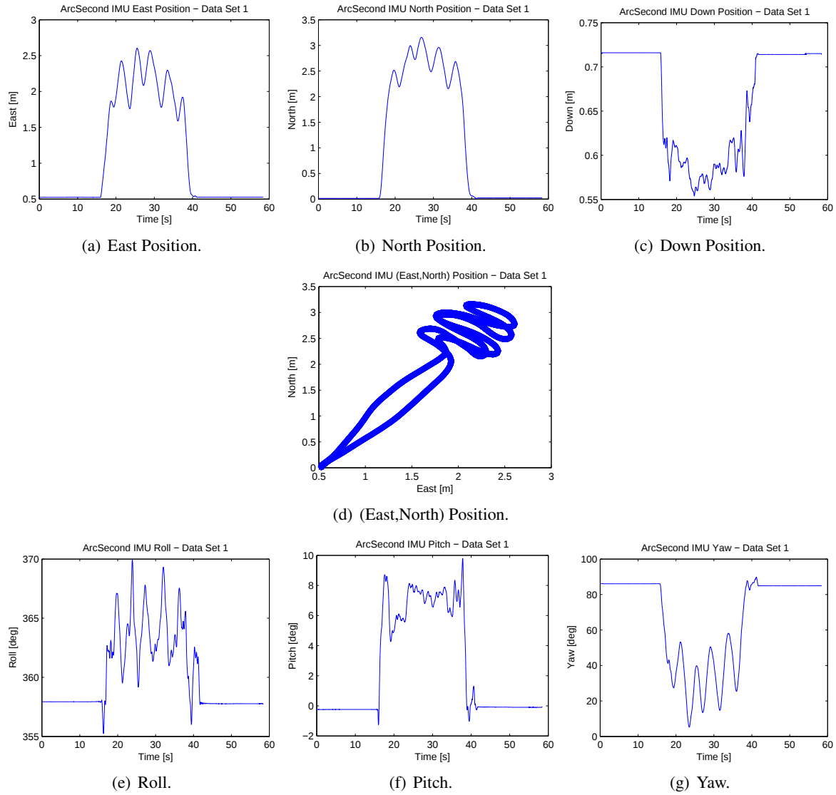
Figure 112: ArcSecond ground truth for data set 1 from the afternoon collection.
