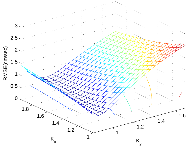
Figure 27: Root of mean square error versus gains K_x and K_y for calculating position of hand-held UXO sensor system along Y orientation.
