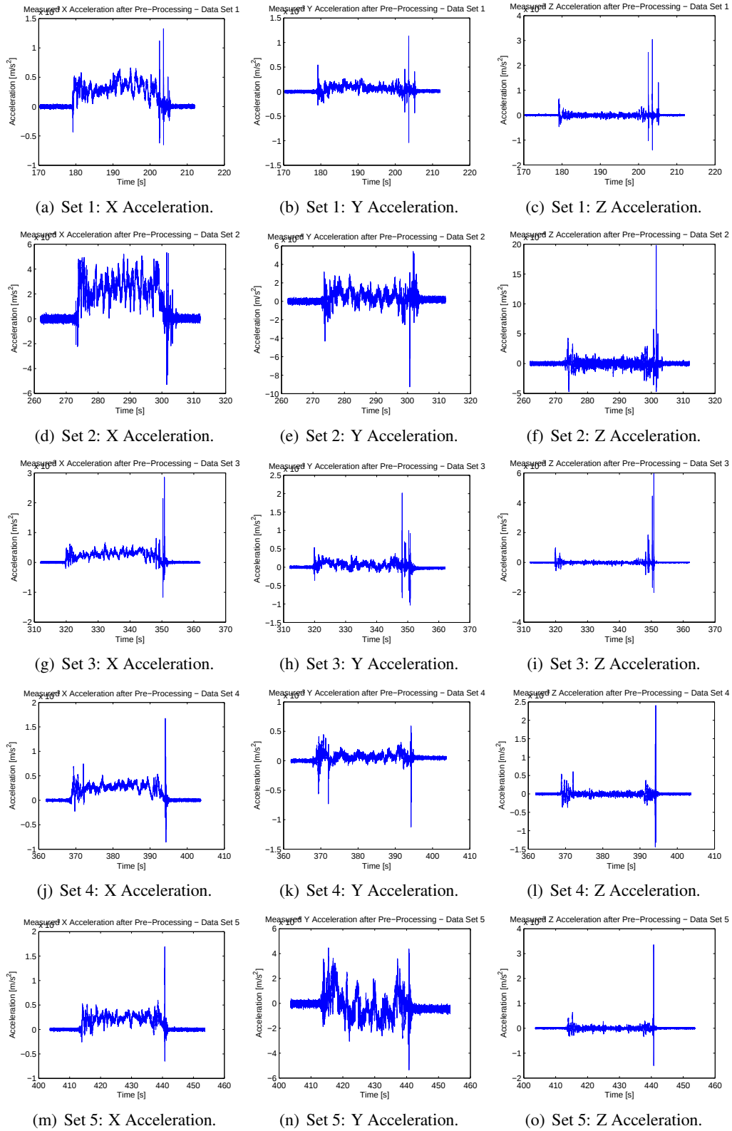
Figure 117: Measured accelerations after pre-processing.
