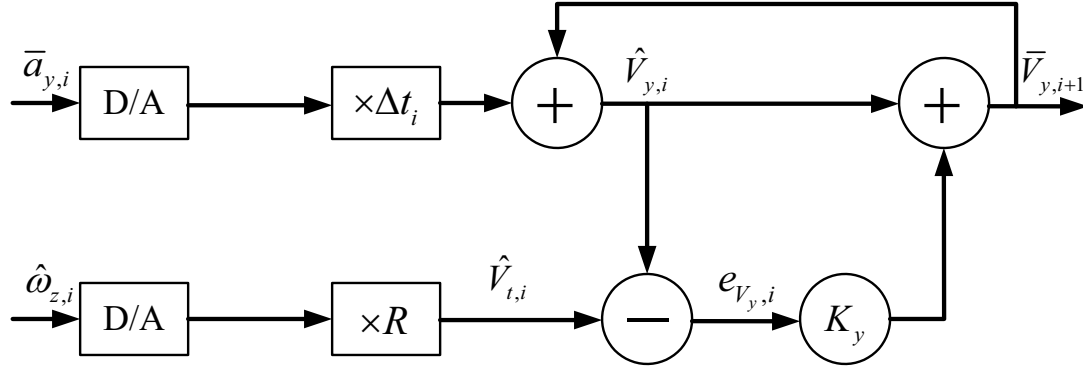
Figure 23: Iterative integration correction algorithm for velocity stabilization along y axes.
