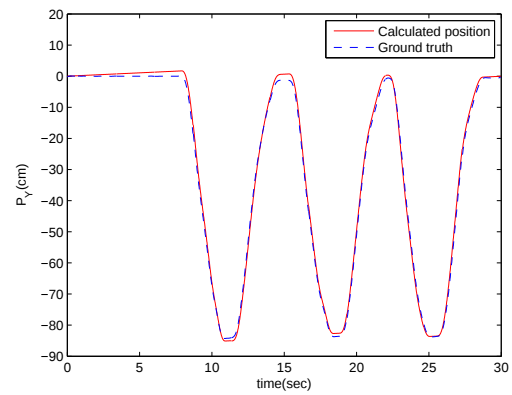
Figure 75: Calculated position along Y orientation based on estimated acceleration. Linear motion.
