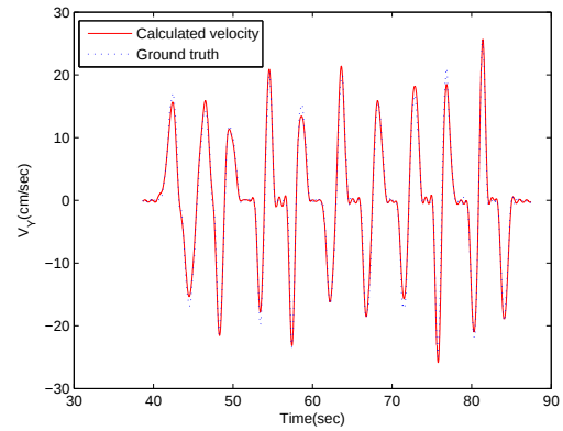
Figure 57: Calculated velocity along Y orientation based on estimated acceleration. Sweeping motion.
