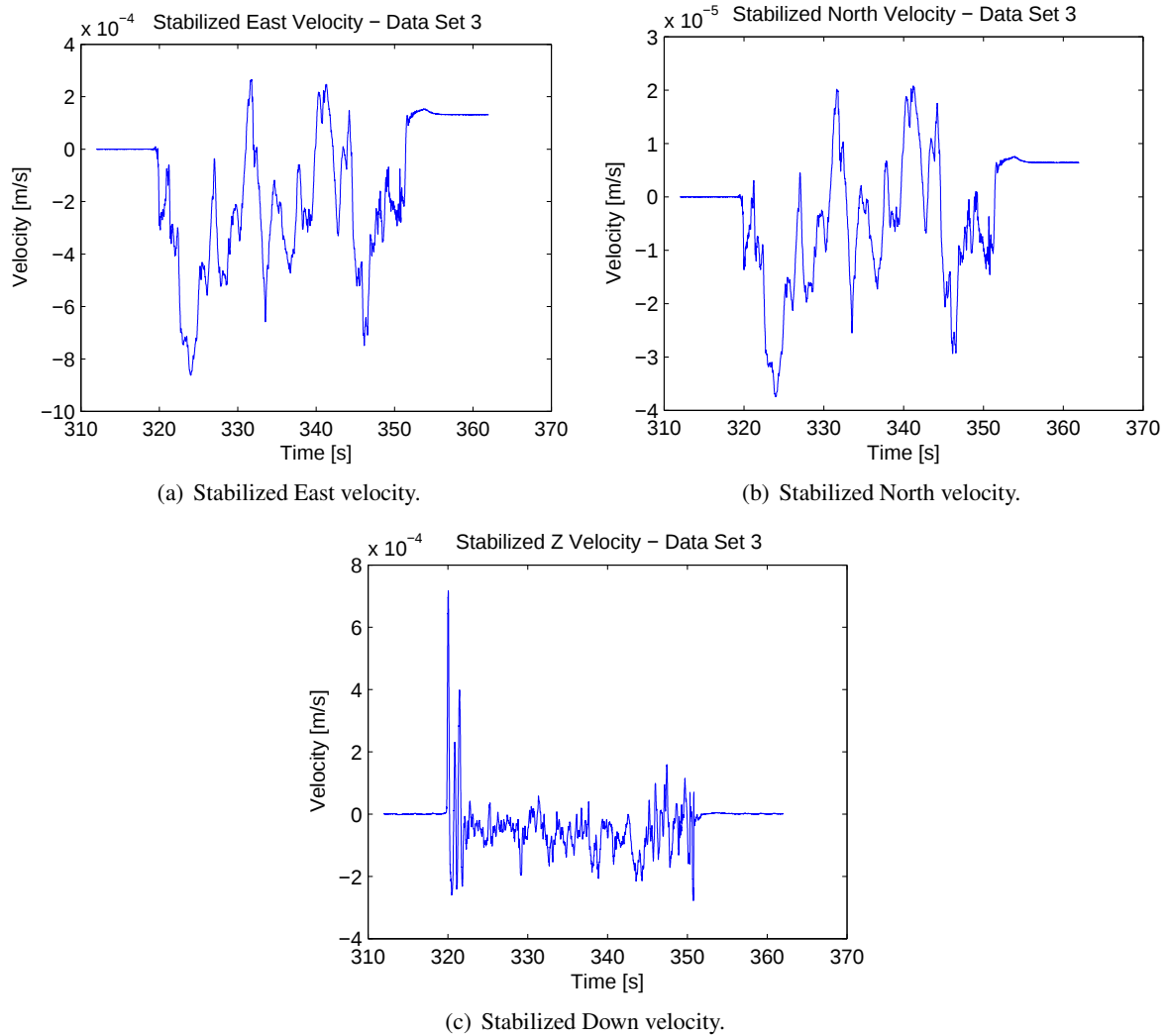
Figure 125: Stabilized velocities (in Earth frame) for data set 3, morning collection.
