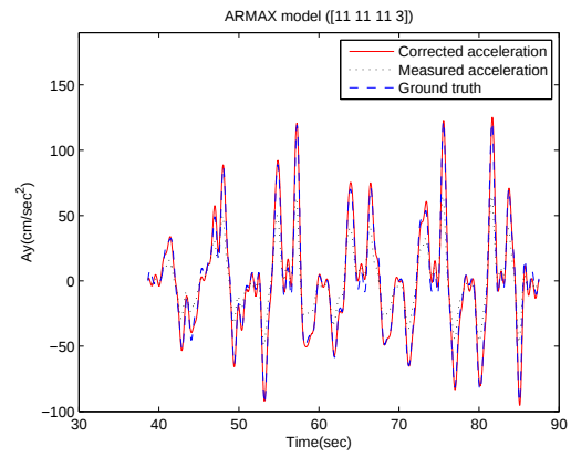
Figure 87: Estimated acceleration along y orientation. a_{meas} is input and \frac{d}{dt}a_{true} is output. na = 11 , nb = 11 , nc = 11 , and nk = 3 .
