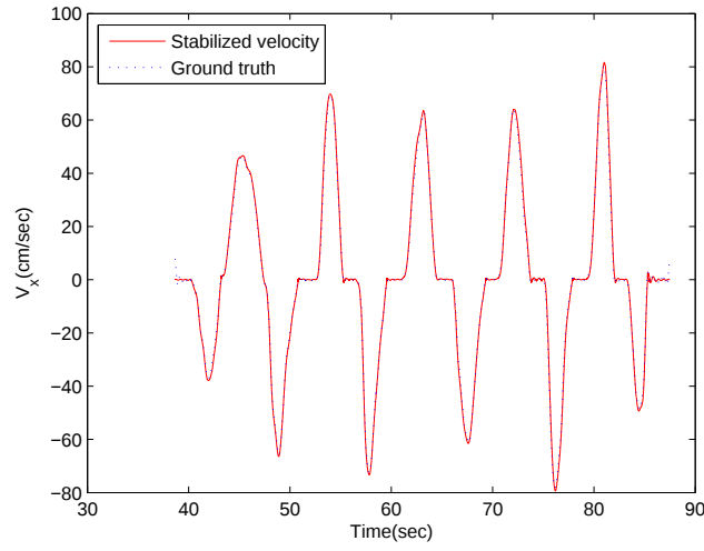
Figure 39: Stabilized velocity along X axes with adaptive optimal gains K_x^{(X),s} = 1.9950 , K_x^{(X),f} = 1.5800 , K_y^{(X),s} = 0.0950 and K_y^{(X),f} = 0.2600 .
