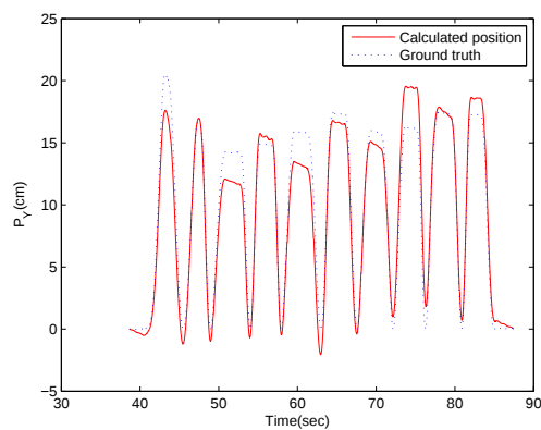
Figure 64: Position along Y orientation calculated from the estimated velocity by direct integration method. Sweeping motion.
