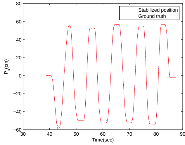
Figure 41: Stabilized position along X axes with adaptive optimal gains K_x^{(X),s} = 1.9950 , K_x^{(X),f} = 1.5800 , K_y^{(X),s} = 0.0950 and K_y^{(X),f} = 0.2600 .
