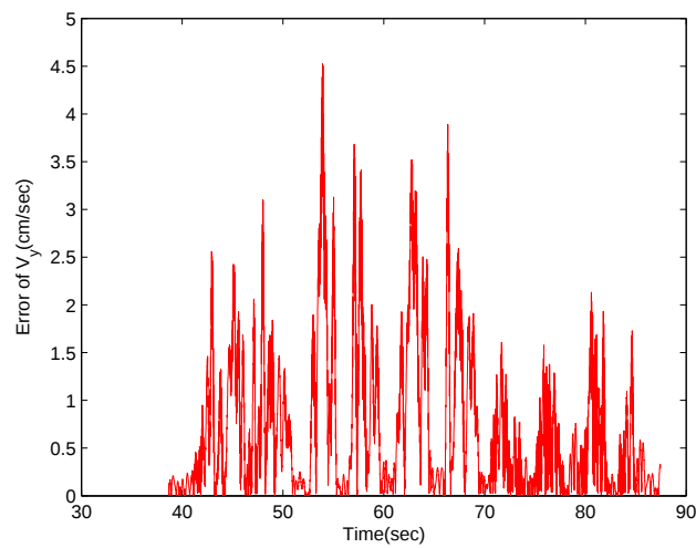
Figure 36: Calculated error of stabilized velocity along Y axes with fixed optimal gains K_x = 1.9000 and K_y = 1.8500 .
