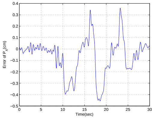
Figure 76: Calculated position error along X orientation based on estimated acceleration. Linear motion.
