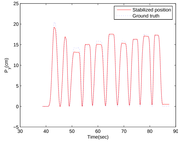
Figure 45: Stabilized position along Y axes with adaptive optimal gains K_x^{(Y),s} = 0.5000 , K_x^{(Y),f} = 1.9900 , K_y^{(Y),s} = 1.9900 and K_y^{(Y),f} = 1.9000 .
