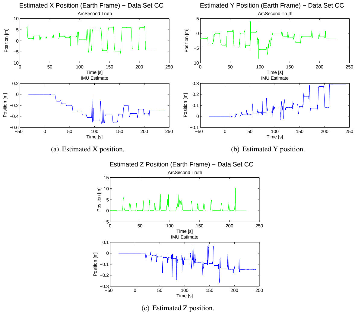
Figure 101: Estimated positions (in Earth frame) and comparison to ground truth for data set 'CC'.
