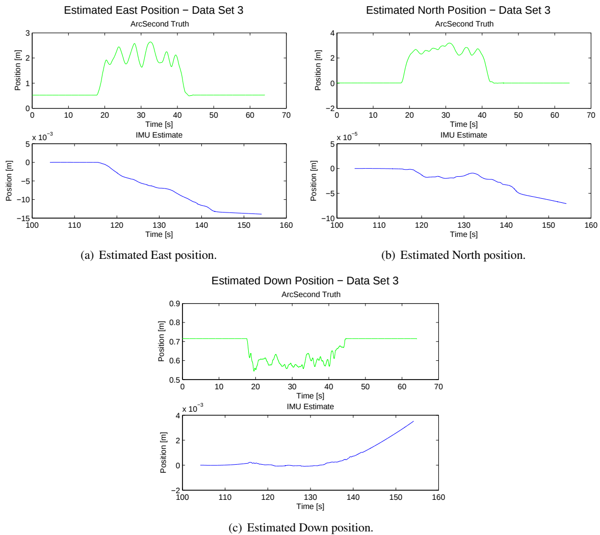
Figure 140: Estimated positions (in Earth frame) and comparison to ground truth for data set 3, afternoon collection.
