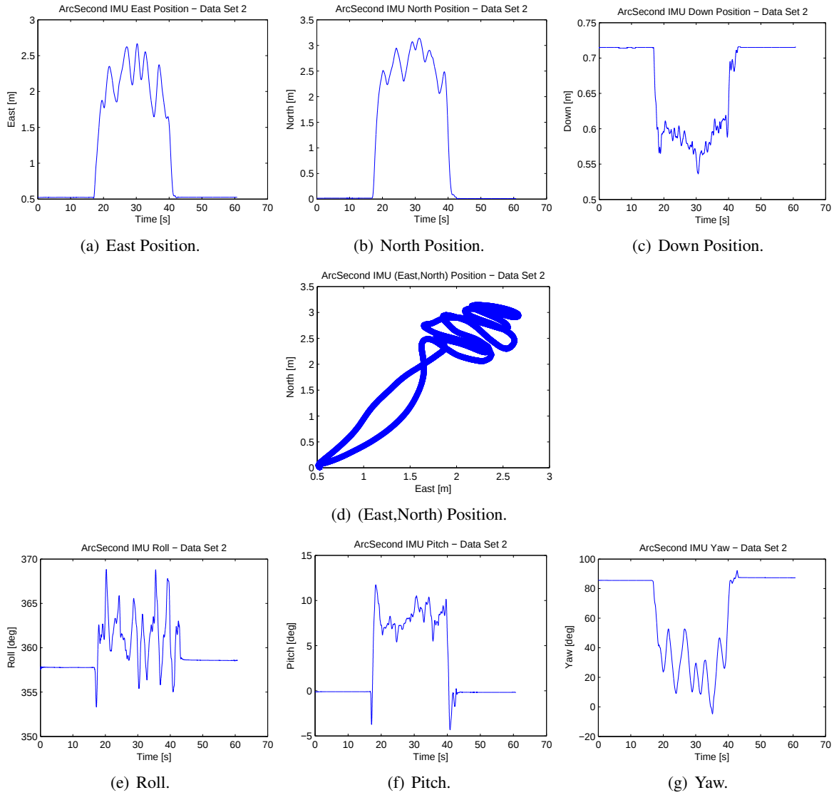
Figure 113: ArcSecond ground truth for data set 2 from the afternoon collection.
