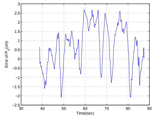
Figure 63: Position error along X orientation calculated from the estimated velocity by zero-position-update method. Sweeping motion.
