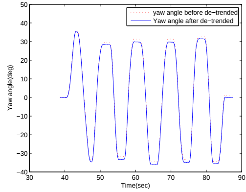
Figure 50: Yaw angle calculation before de-trended and after de-trended.
