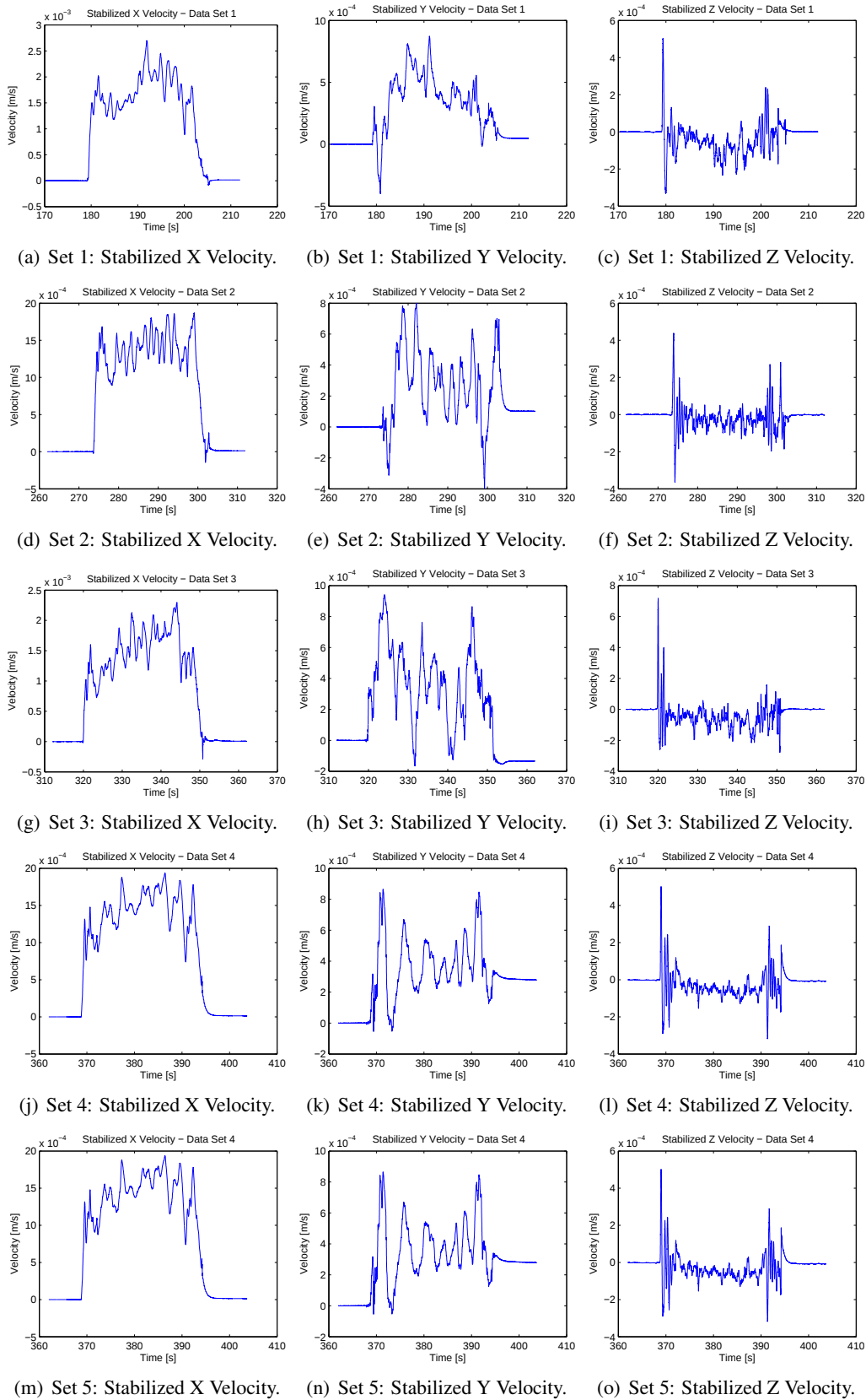
Figure 119: Stabilized velocities after bias and trend removal.
