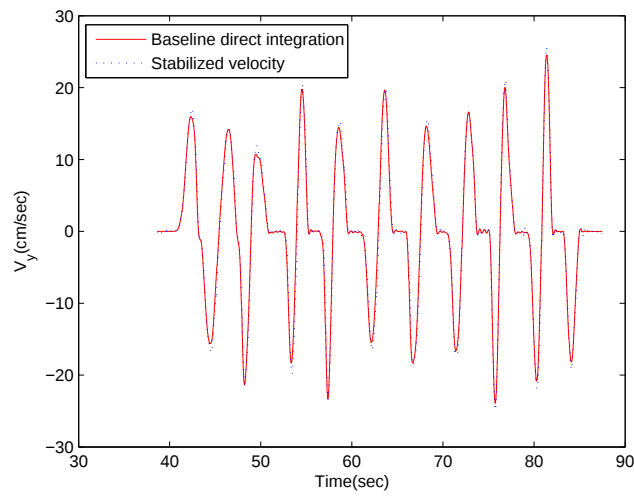
Figure 35: Stabilized velocity along Y axes with fixed optimal gains K_x = 1.9000 and K_y = 1.8500 .
