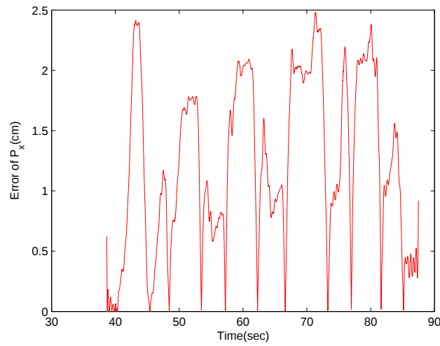
Figure 42: Calculated error of stabilized position along X axes with adaptive optimal gains K_x^{(X),s} = 1.9950 , K_x^{(X),f} = 1.5800 , K_y^{(X),s} = 0.0950 and K_y^{(X),f} = 0.2600 .
