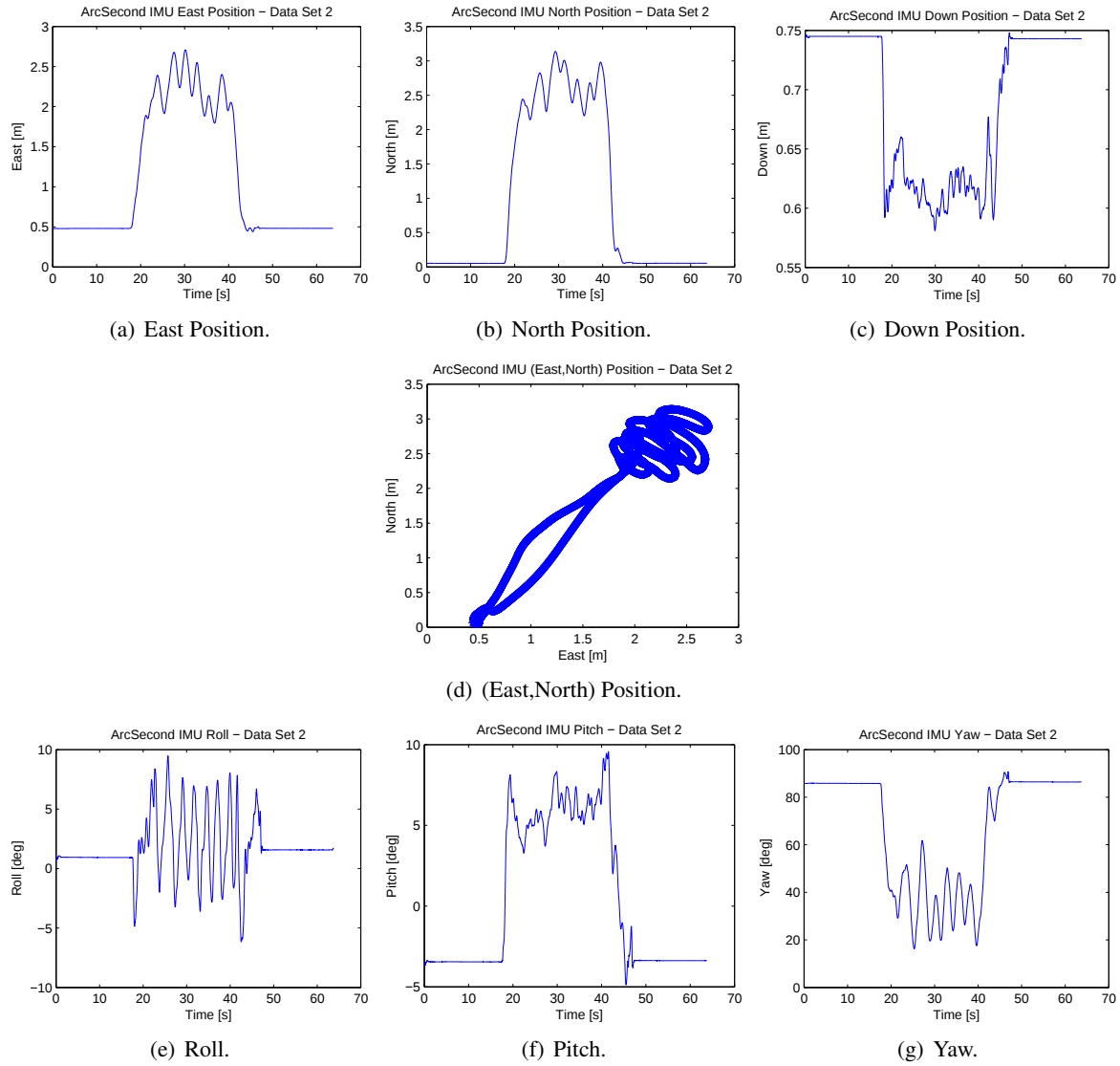
Figure 108: ArcSecond ground truth for data set 2 from the morning collection.
