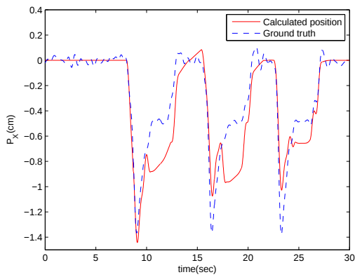
Figure 74: Calculated position along X orientation based on estimated acceleration. Linear motion.
