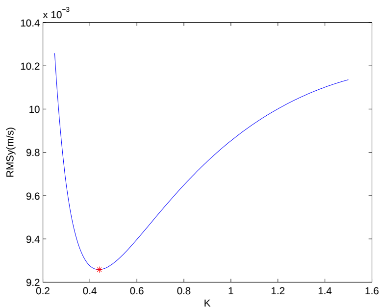
Figure 8: Example illustrating choosing K_y .
