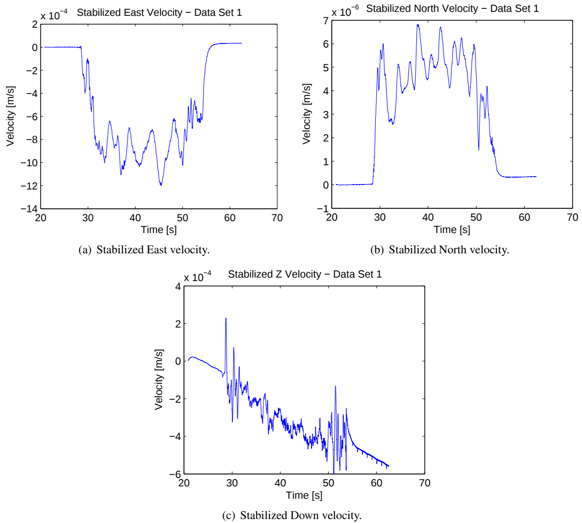
Figure 128: Stabilized velocities (in Earth frame) for data set 1, afternoon collection.
