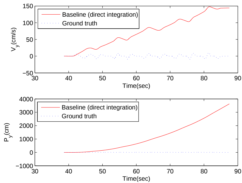
Figure 30: Calculated velocity and position along Y orientation directly using the conventional integration method.
