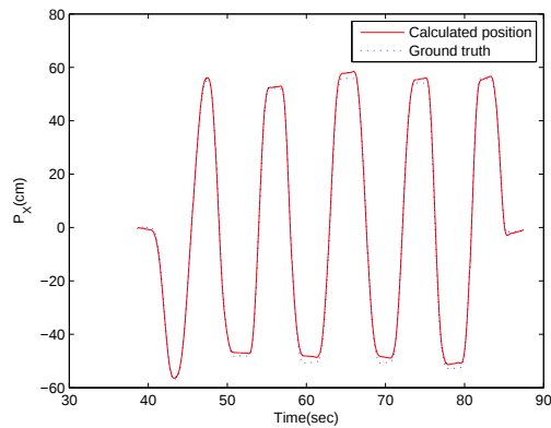
Figure 62: Position along X orientation calculated from the estimated velocity by zero-position-update method. Sweeping motion.
