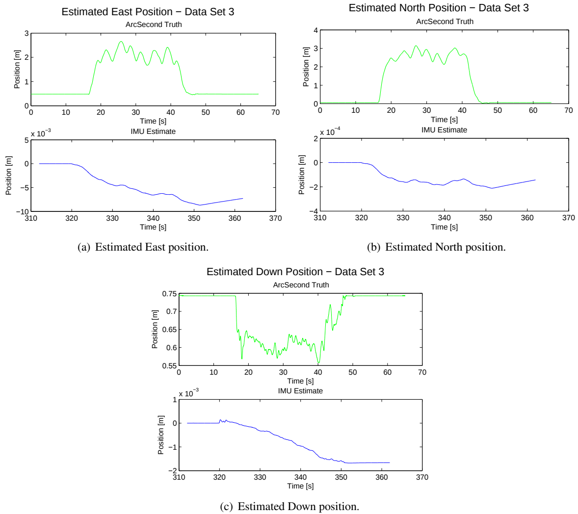
Figure 135: Estimated positions (in Earth frame) and comparison to ground truth for data set 3, morning collection.
