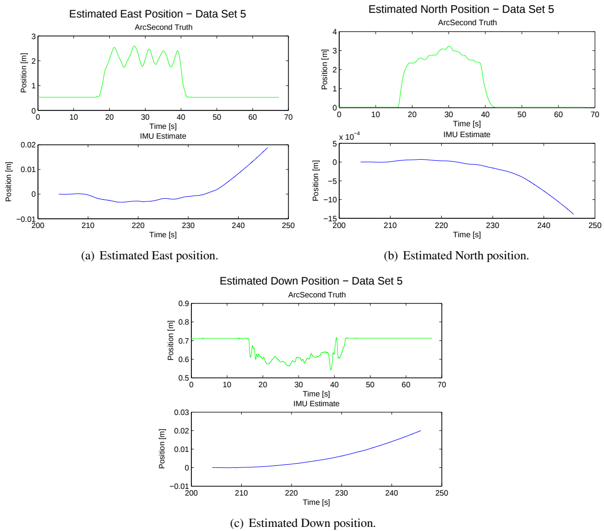
Figure 142: Estimated positions (in Earth frame) and comparison to ground truth for data set 5, afternoon collection.
