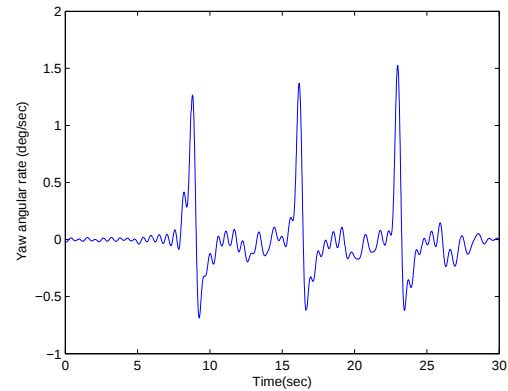
Figure 48: Yaw angular rate of linear motion of handheld UXO sensor.
