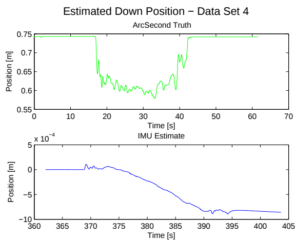
(c) Estimated Down position.
