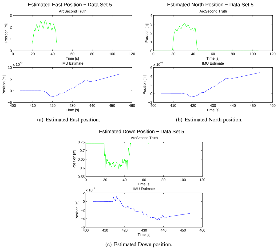
Figure 137: Estimated positions (in Earth frame) and comparison to ground truth for data set 5, morning collection.
