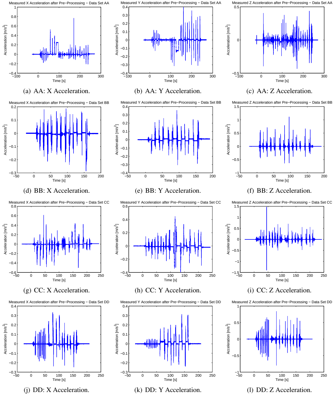
Figure 92: Measured accelerations after pre-processing.
