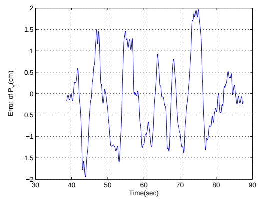
Figure 67: Position error along Y orientation calculated from the estimated velocity by zero-position-update method. Sweeping motion.
