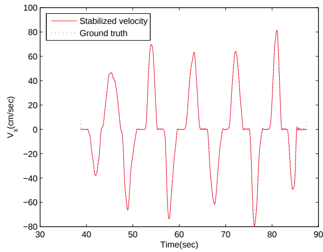
Figure 31: Stabilized velocity along X orientation with fixed optimal gains K_x = 1.9800 and K_y = 0.2800 .
