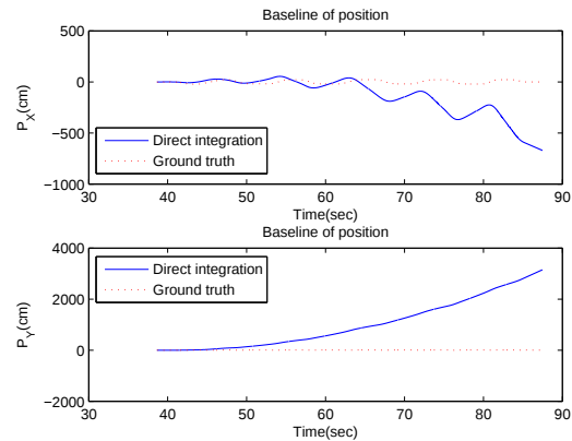
Figure 55: Position calculated from raw acceleration by the conventional numerical integration. Sweeping motion.
