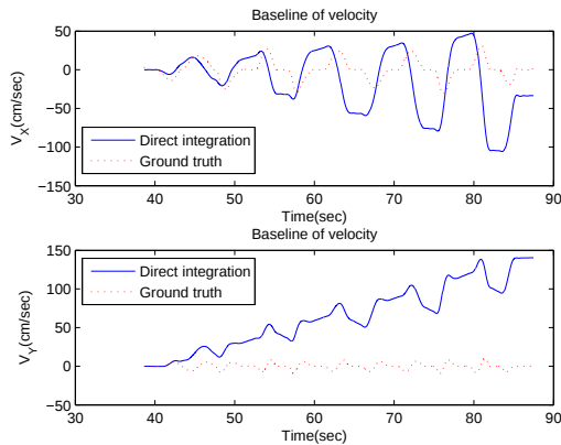
Figure 54: Velocity calculated from raw acceleration by the conventional numerical integration. Sweeping motion.
