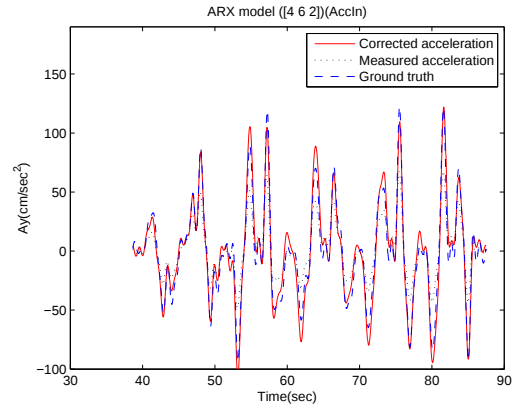
Figure 82: Estimated acceleration along y orientation. a_{meas} is input and a_{true} is output. na = 4 , nb = 6 and nk = 2 .
