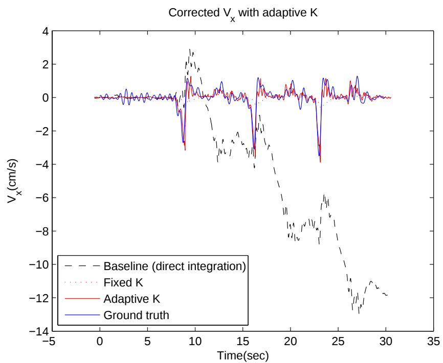
Figure 15: Calculated velocity along the x axis based on the linear data.
