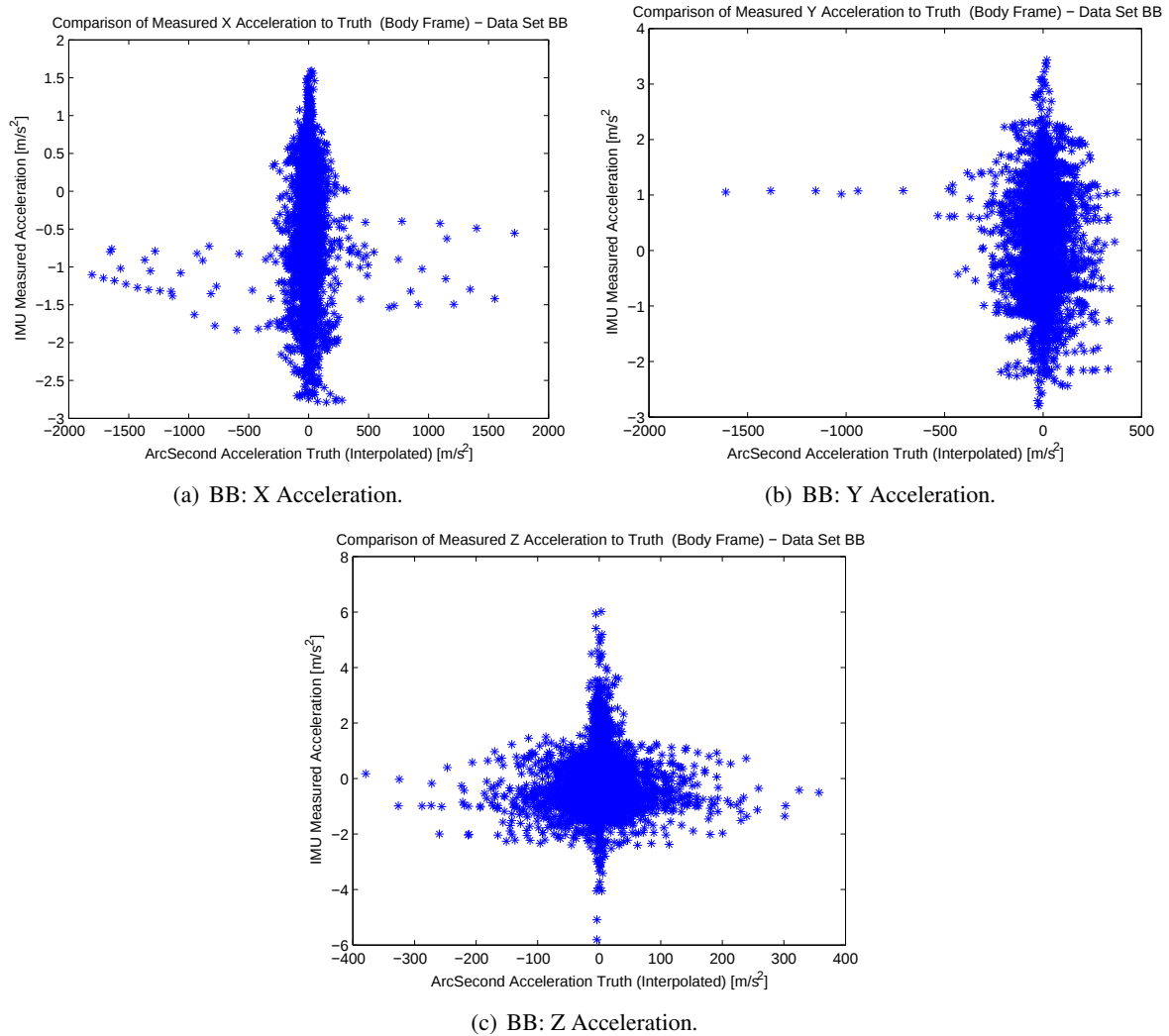
Figure 104: Comparisons of true and measured accelerations (in IMU body frame) for data set 'BB'.
