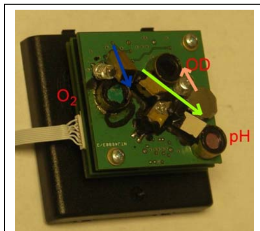
Figure 11. Detection block. The arrows show the spatial direction of light emissions
