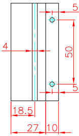
A View
