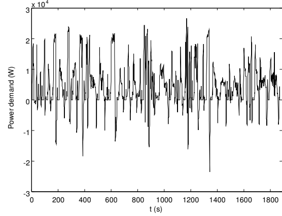
Fig. 8. Load profile of OCC.
