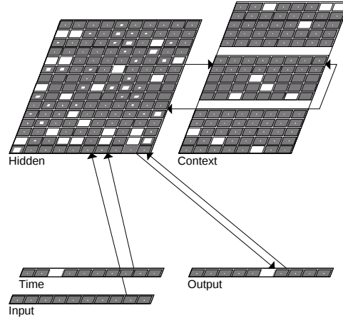
Figure 1: Phonological loop model. Ten different input symbols are possible at each time step (one unit out of ten activated in the Input layer). A sequence is encoded in one pass by presenting the Input together with the sequential location in the Time input layer for each step in the sequence. The simulated basal ganglia gating mechanism (implemented by fiat in script code) uses the time input to trigger intracellular maintenance currents in the corresponding stripe region of the context (PFC) layer (stripes are shown as the three separate groups of units within the Context layer; individual context units also had an excitatory self-connection for maintenance). Thus, the first stripe must learn to encode the first input, etc. Immediately after encoding, the network is then trained to produce the correct output in response to the time input, without any Input activation (the activation state shown is the network correctly recalling the third item in a sequence). The hidden layer must therefore learn to decode the context representations for this recall phase. Generalization testing involved presenting untrained sequences.
