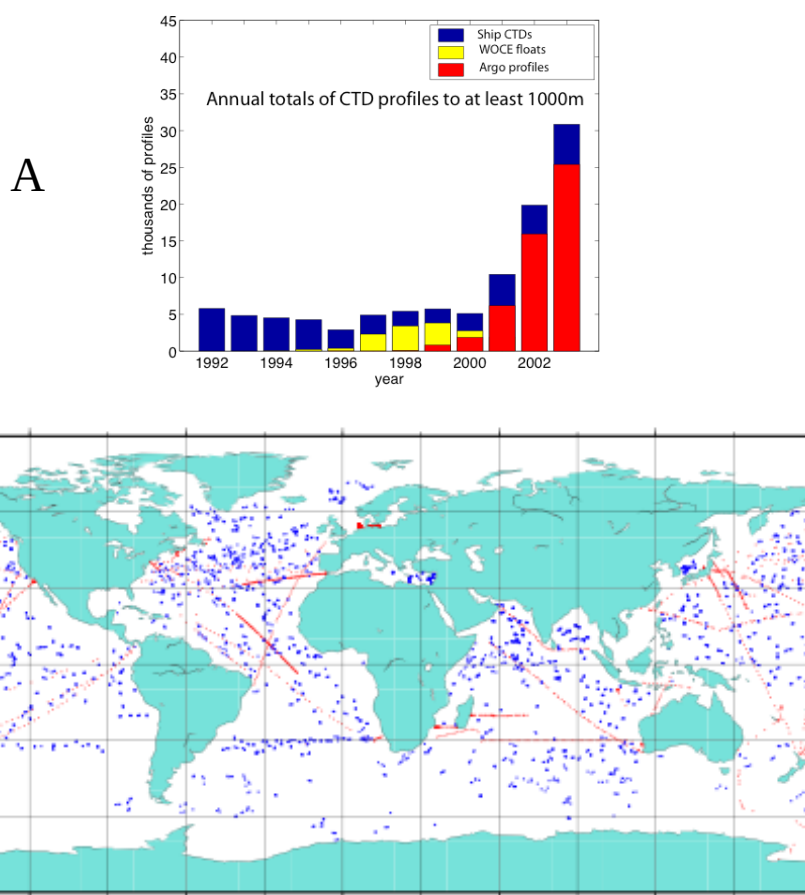
Fig 2A CTD profile data to depths of 1000m by year. Prior to 1996, all were ship based. Profiling floats developed during WOCE (1990-1997) were the forerunner of Argo. Ship based profiles, with absolute salinity calibrations, are still needed to update ocean climatologies used for Argo float calibrations. (Courtesy of Josh Willis, SIO) 2B Data delivered in real time during December 2003 from Argo (3001 CTD profiles typically to over 1000m - Blue dots) and from the High density XBT network (temperature to typically 750m – Red dots). Courtesy AOML.
