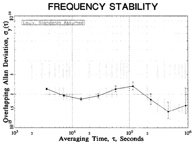
Figure 6. Allan Deviation of USNO MC – AOG6 (after initial settling)
