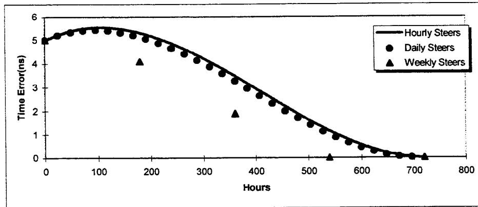
Figure 2. Minimal Control Effort Simulations: Initial Time Error=5 ns, Freq. Error= 3 \times 10^{-15}
