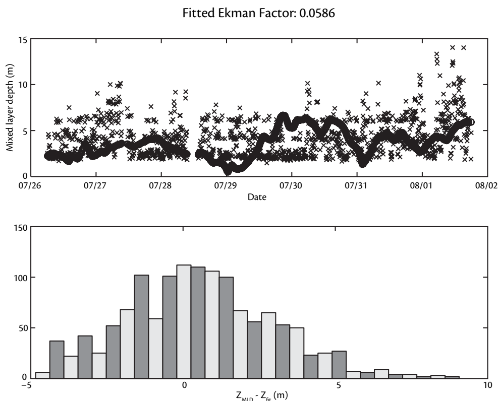
Figure 3. Uncertainties in multiple model parameters. Example of the mixing-layer depth factor over the MAB shelfbreak front region. This factor is the proportionality “Ekman factor ( E_k )” linking the Ekman depth to the turbulent friction velocity and the Coriolis frequency. Top: Fitted mixed-layer depth (dark continuous curve) and estimated mixed-layer depths (crosses) computed for every Seasoar ocean data profile and the corresponding local atmospheric model of wind-stress (Baugmarter and Anderson, 1996) at the profile location and time. Bottom: Distribution of the misfit between: (1) mixed-layer depths estimated from the wind-stress and the ocean data; and (2), the fitted mixed-layer depth (dark curve on top). The fitted Ekman factor is 0.0586.
