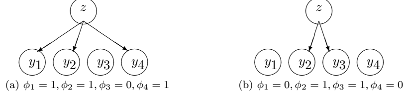
Figure 4.4: An example graphical model for the probability model in Equation (4.5) for the case of four features ( d = 4 ) with different indicator variables. \phi_l = 1 corresponds to the existence of an arc from z to y_l , and \phi_l = 0 corresponds to its absence.
