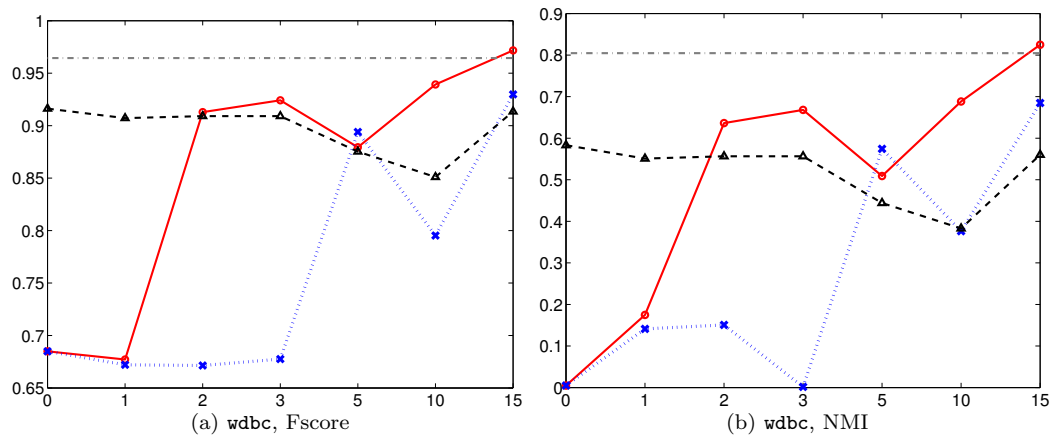
Figure 5.9: F-score and NMI for different algorithms for clustering under constraints for the data sets wdbc . The results of the proposed algorithm, Shental , and Basu are represented by the red solid line, blue dotted lines and the black dashed line, respectively. The performance of a classifier trained using all the labels is shown by the gray dashdot line. The horizontal axis shows the number of constraints as the percentage of the number of data points.
