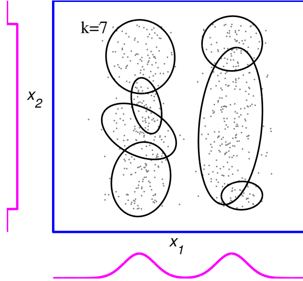
Figure 4.1: An irrelevant feature ( x_2 ) makes it difficult for the Gaussian mixture learning algorithm in [81] to recover the two underlying clusters. Gaussian mixture fitting finds seven clusters when both the features are used, but identifies only two clusters when the feature x_1 is used. The curves along the horizontal and vertical axes of the figure indicate the marginal distribution of x_1 and x_2 , respectively.
