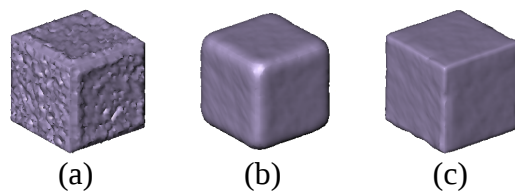
Figure 5.2: (a) Initialization from noisy data. Resulting model for (b) isotropic reconstruction, and (c) anisotropic reconstruction with \alpha = 10 .
