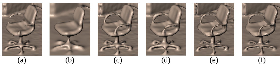
Figure 5.4: Results for the surface area reconstruction with weights (a) 1, and (b) 10, isotropic reconstruction with weights (c) 1, and (d) 10, anisotropic reconstruction with weights (e) 1, and (f) 10.
