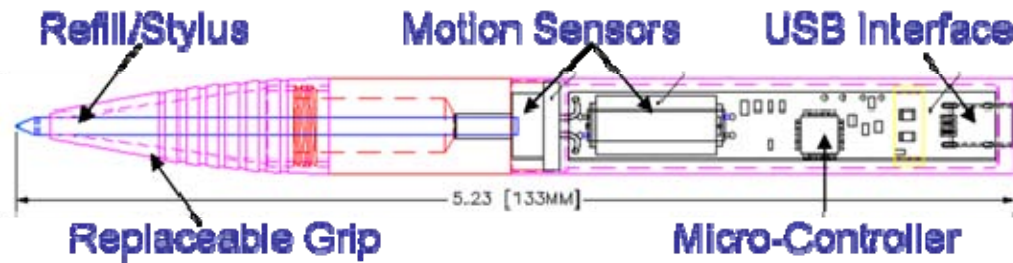
Figure 15. DynaSig Bio-Pen Components
