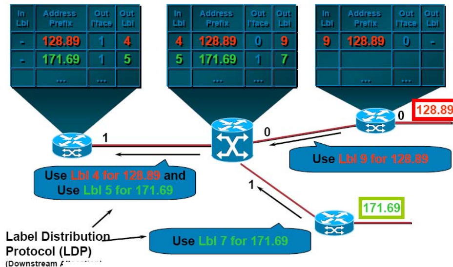
Figure 6. A MPLS network example: Assigning Labels (From: [17])
