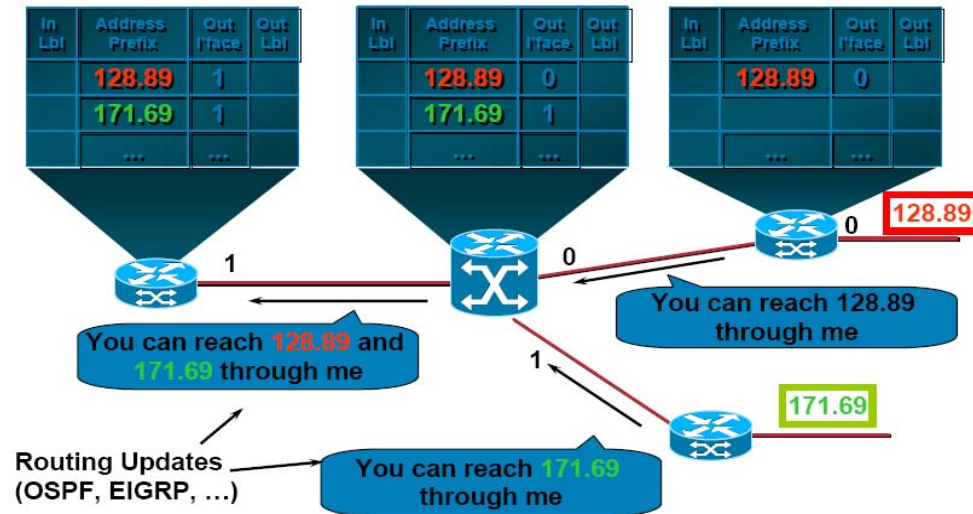
Figure 5. A MPLS network example: Exchange routing information (From: [17])
