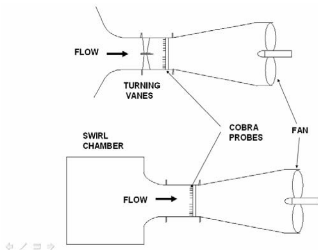
Figure 9. Generator Wind Tunnel Test Installations
