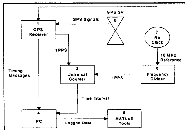
Figure 5: External Oscillator Test Setup
