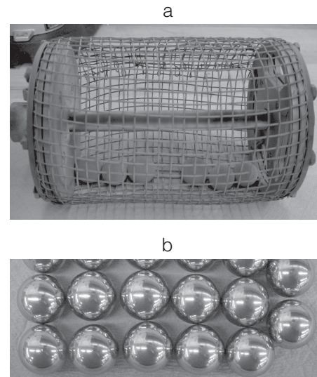
Figure 4. (a) Cage used for applying Re coatings on 18 graphite cores and (b) polished cores with surface finish <Ra8.
