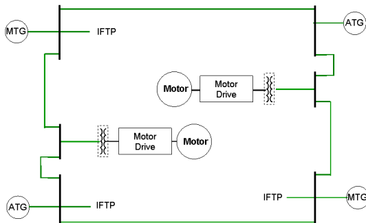
Fig. 2. Notional IPS Medium Voltage AC Distribution System
