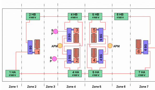
Fig. 1. Notional AC-Zonal Distribution System
