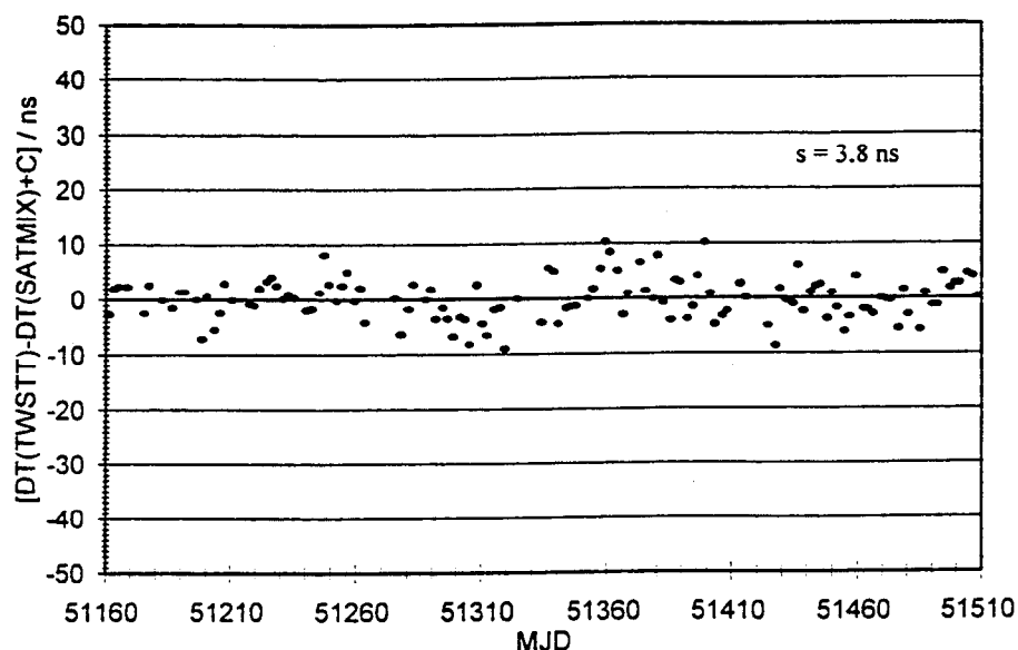
Figure 8: Difference between the measurement results of two time comparison methods (TWSTT method and SATMIX method). s: standard deviation. C: constant. MJD: Modified Julian Date, MJD 51160: December 13, 1998. DT(TWSTT) = UTC(PTB) - UTC(TUG) : determined by the TWSTT method DT(SATMIX) = UTC(PTB) - UTC(TUG) : determined by the SATMIX method.
