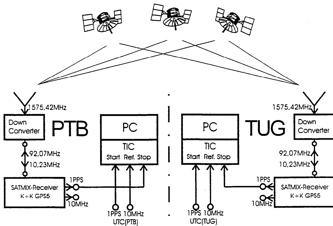
Figure 3: Block diagram of the setup for SATMIX time scale comparisons UTC(PTB)-UTC(TUG).
