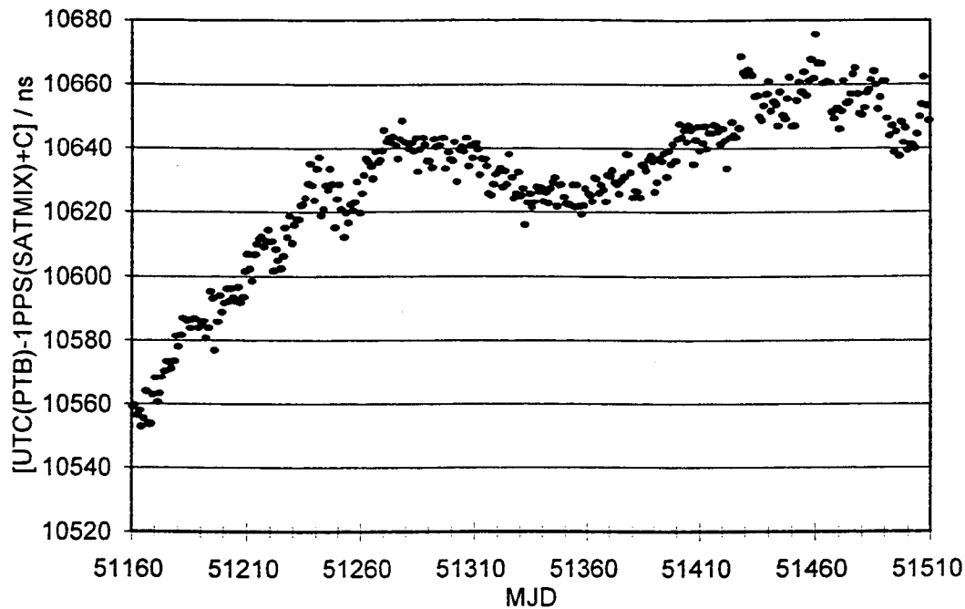
Figure 4: Daily mean values of the time differences \text{UTC(PTB)} - 1\text{PPS(SATMIX)} measured at the PTB in Braunschweig. MJD: Modified Julian Date, MJD 51160: December 13, 1998.
