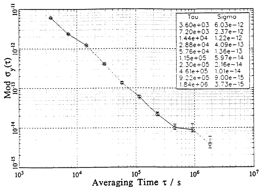
Figure 6: Relative frequency instability of the 1PPS(SATMIX) output signal, expressed by the modified Allan standard deviation \text{Mod } \sigma_y(\tau) , calculated from the hourly mean values of the time differences UTC(PTB) - 1PPS(SATMIX).
