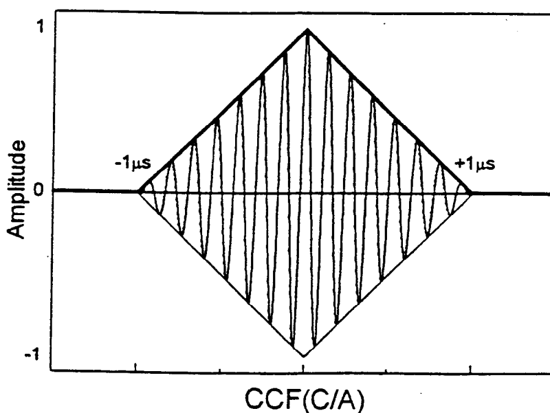
Figure 1: Cross-correlation function CCF(C/A) for C/A code synchronization. The indicated carrier oscillations illustrate the advantages of carrier-phase smoothing because of the steep slope of the carrier zero-crossings compared with the CCF(C/A) .
