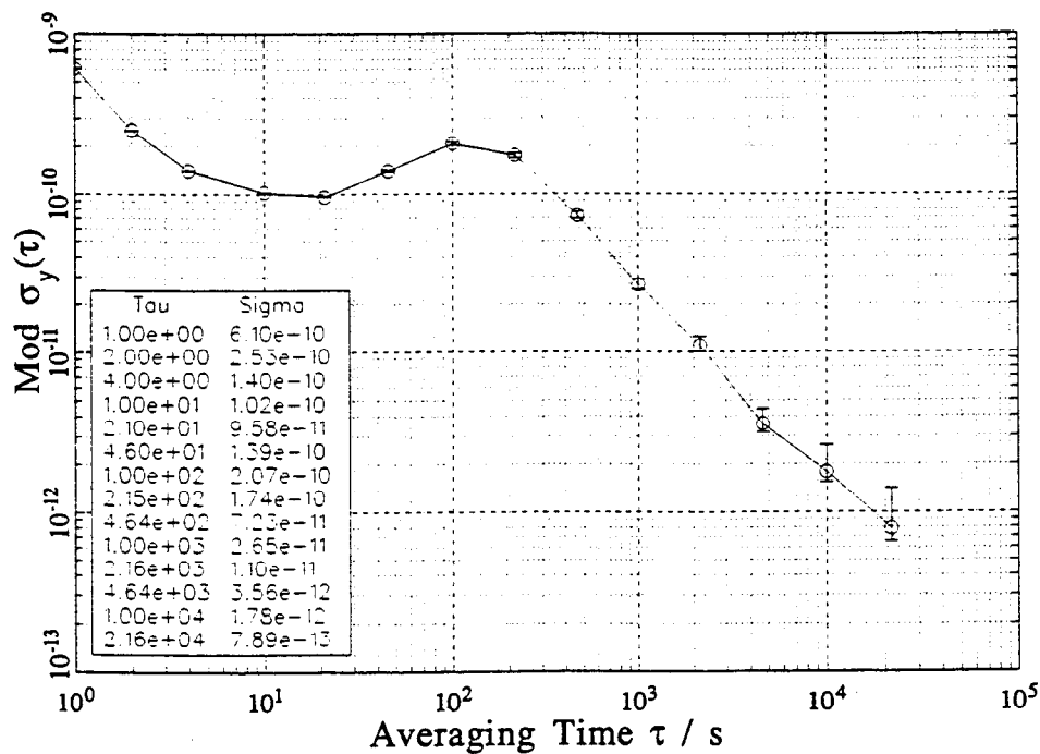
Figure 5: Relative frequency instability of the 1PPS(SATMIX) output signal, expressed by the modified Allan standard deviation \text{Mod } \sigma_y(\tau) , determined from the time differences \text{UTC(PTB)} - 1\text{PPS(SATMIX)} measured every second.
