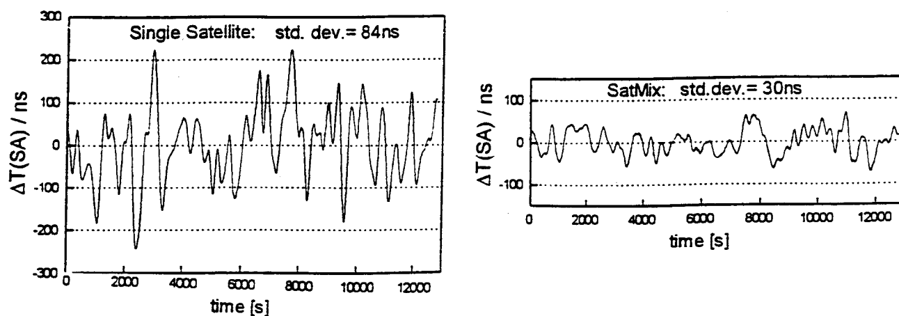
Figure 2: Phase time variations \Delta T(SA) of the receiver output signal caused by the "Selective Availability." On the left: reception of a single satellite only. On the right: Multiplex reception and SATMIX averaging of all satellites in view.
