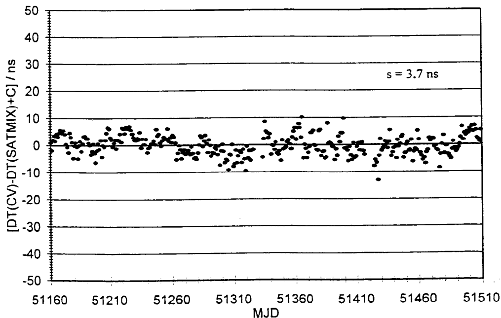
Figure 7: Difference between the measurement results of two time comparison methods (CV method and SATMIX method). s: standard deviation. C: constant. MJD: Modified Julian Date. MJD 51160: December 13, 1998 DT(CV) UTC(PTB)-UTC(TUG): determined by the CV method DT(SATMIX) UTC(PTB)-UTC(TUG): determined by the SATMIX method.
