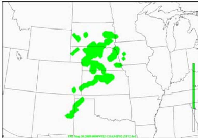
Figure 66. 080529NAM-WRF 12Z Run – 12-hr Forecast (valid 30/00Z). 1× Filter – Theta-e and LR Intersections (green area).
