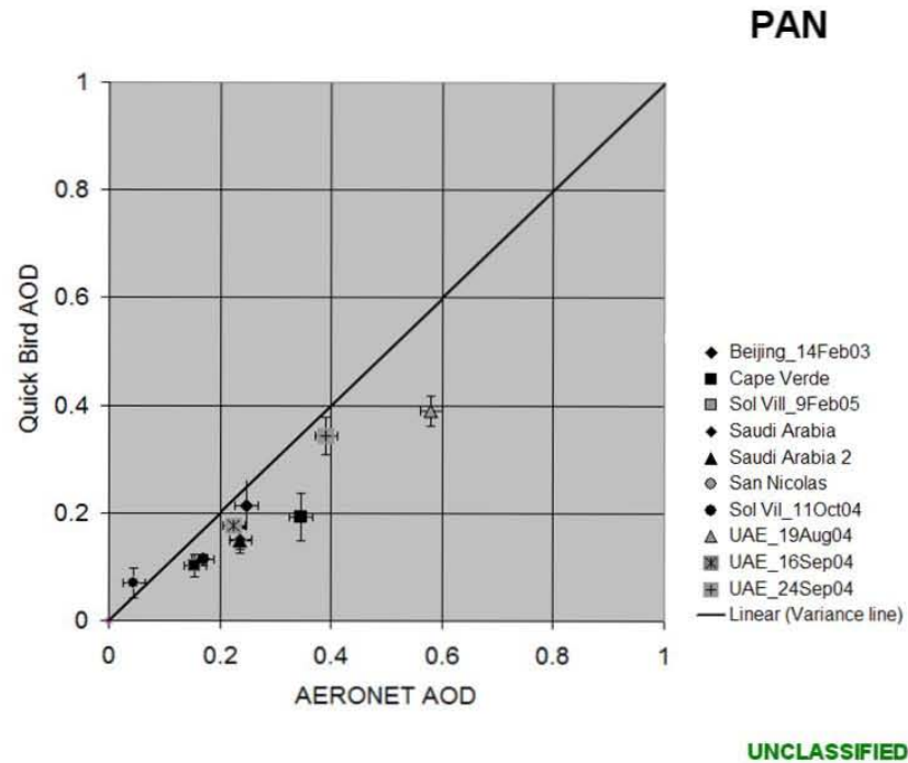
Figure 2. The graphic shows examples of the panchromatic AOD retrieval low bias for several case studies in various locations worldwide. (After: Durkee 2008)
