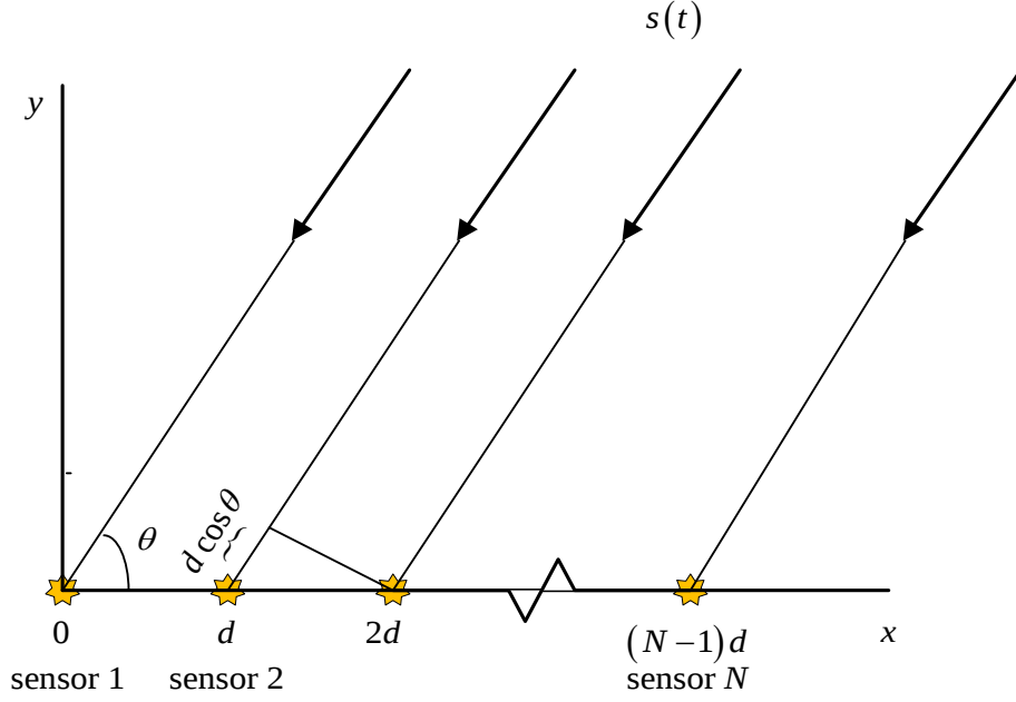
Figure 2. Uniform linear array of N sensors with inter-element spacing d . The source is located in the far field.
