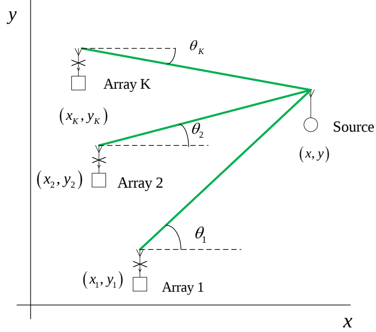
Figure 14. LOS DOA-based source localization using three arrays.
