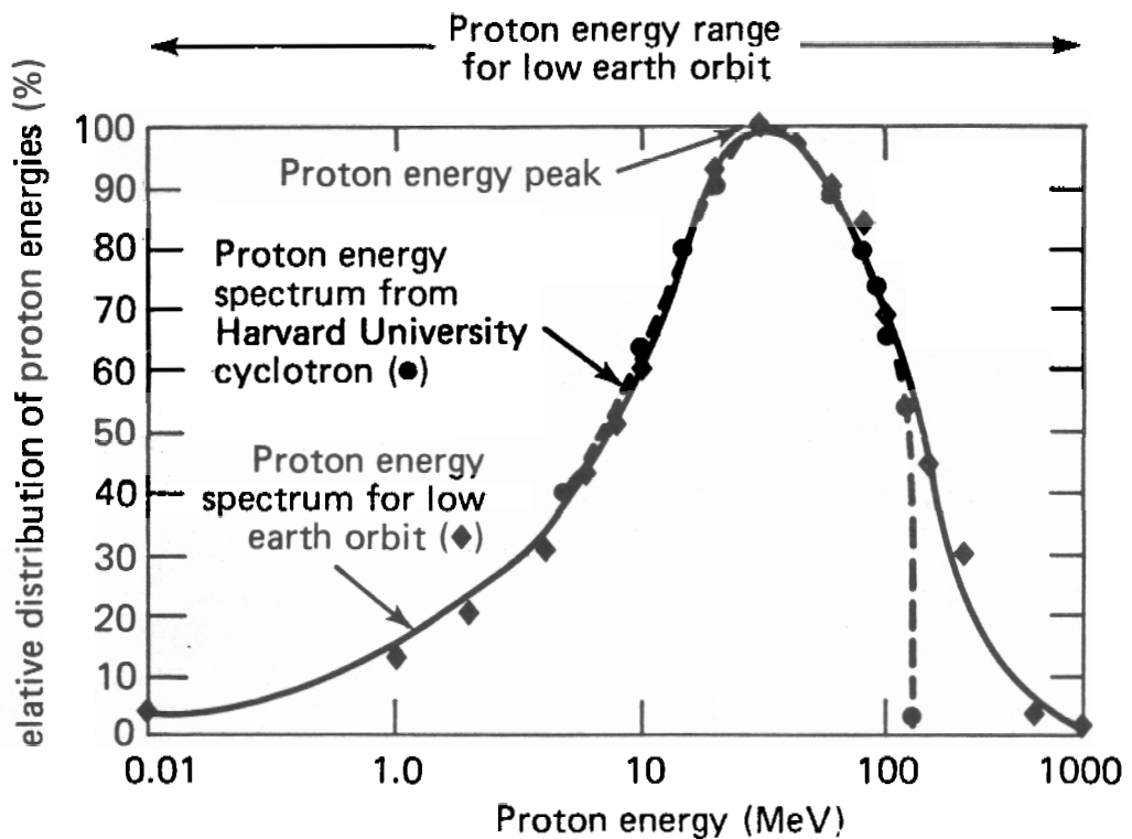
Figure 16. Low earth orbit and cyclotron proton spectra.
