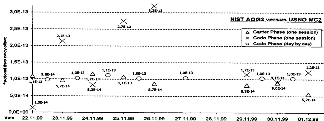
Figure 12: Frequency Transfer, PN versus Carrier Phase
