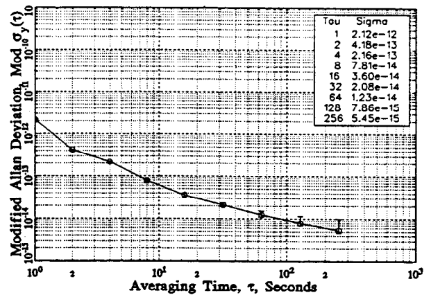
Figure 8: MDEV, carrier phase, signal 2.5 MChip/s, USNO vs. NIST
