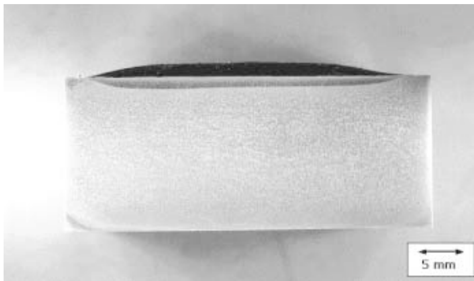
Figure 4. Nickel-aluminum-bronze on 4140 steel using a high-power CO 2 laser.
