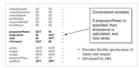
Figure 7. Constraint map for power section.
