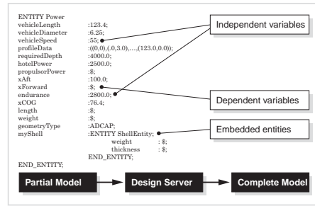
Figure 5. Clear text encoding for a power section.
