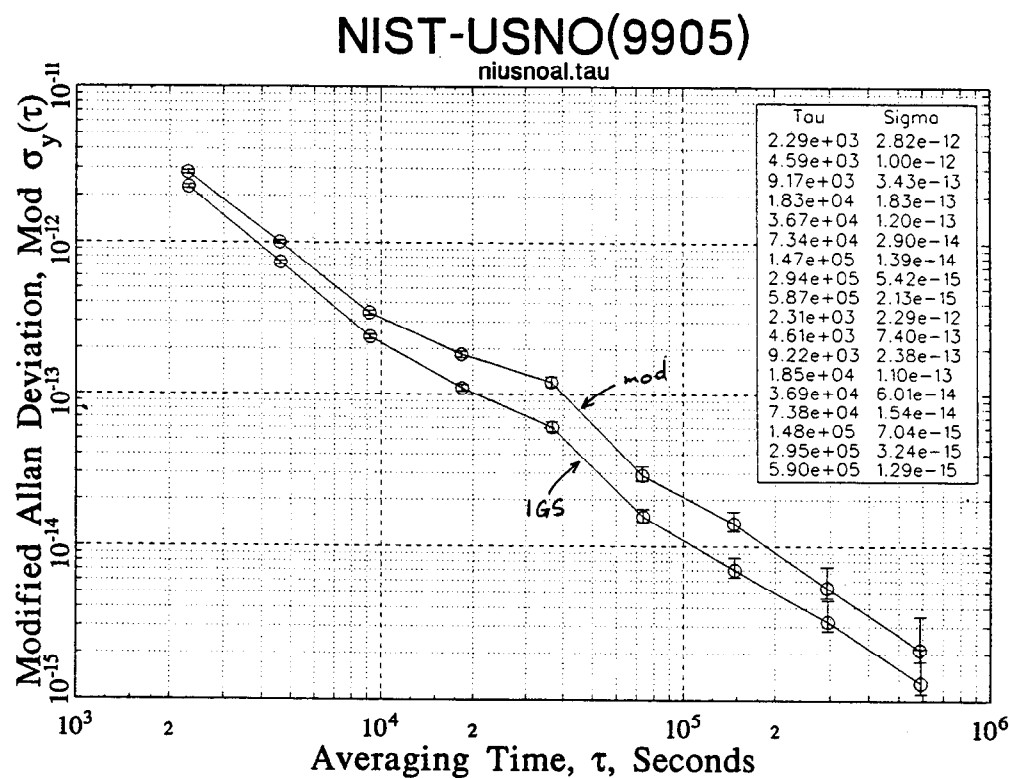
Figure 2: Stabilities of NIST (USA) – USNO (USA) common views for May 1999 (labels as in Fig. 1).
