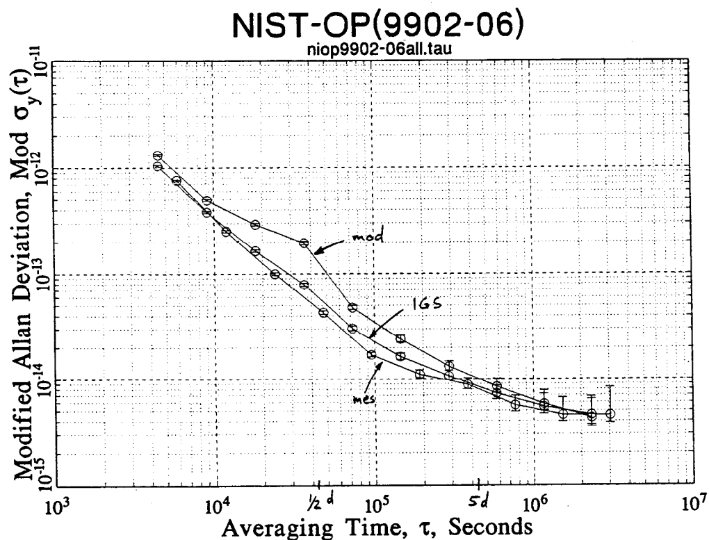
Figure 8: Stabilities of NIST (USA) – OP (France) common views for February through June 1999 (labels as in Fig. 1).
