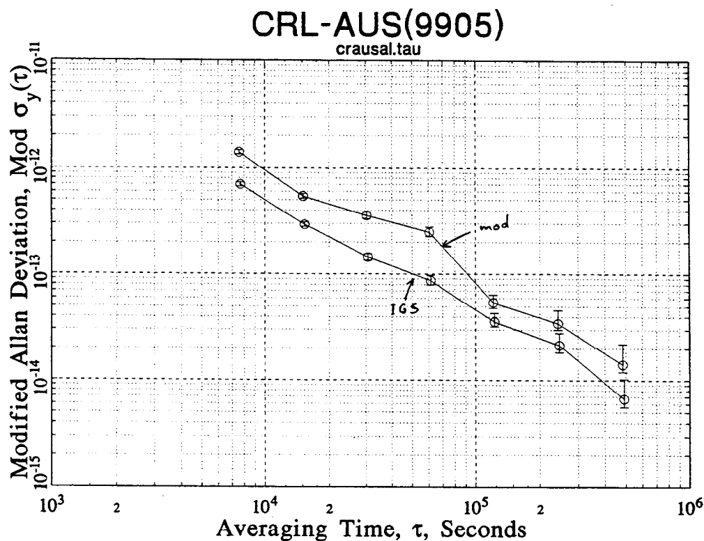
Figure 3: Stabilities of CRL (Japan) – AUS (Australia) common views for May 1999 (labels as in Fig. 1).
