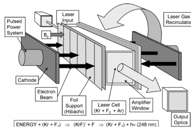
Fig. 1. The main components of an electron beam pumped KrF laser.
