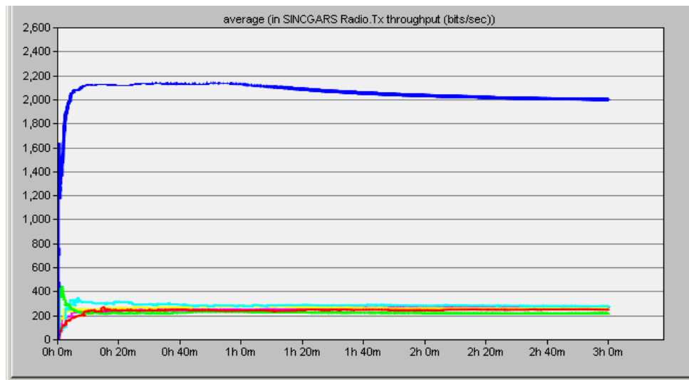
Figure 40. SINGARS Platoon (All): Average Tx Throughput
