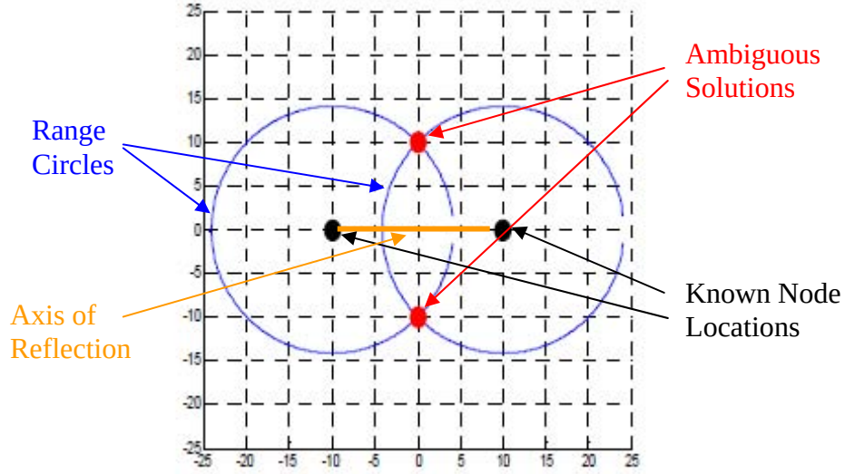
Figure 15. Two-node, two-range solution set (after [3]).
