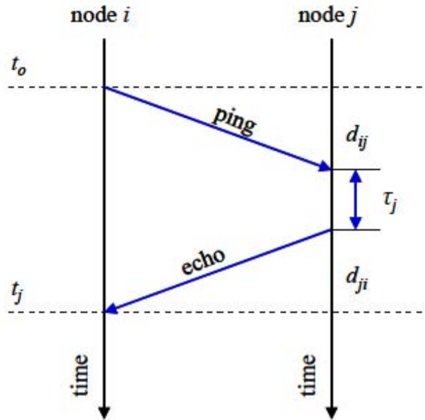
Figure 6. Seaweb ranging process (from [2]).
