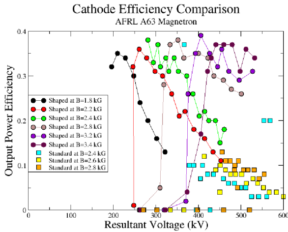
Fig. 3 Higher efficiency for the shaped cathode
