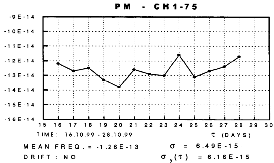
Fig.6. Frequency stability of the passive hydrogen maser at \tau = 1 day.
