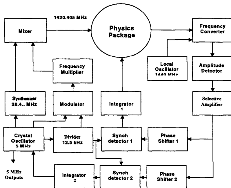
Fig.3. Block diagram of the passive hydrogen maser.
