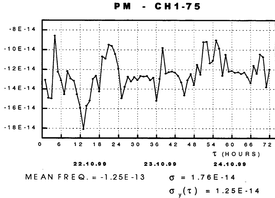
Fig.5. Frequency stability of the passive hydrogen maser at \tau = 1 hour.
