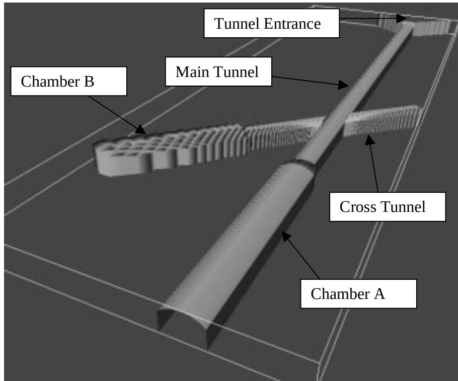
Figure 4. Large Scale Alvtdalen Tunnel, ARA SHARC Model
