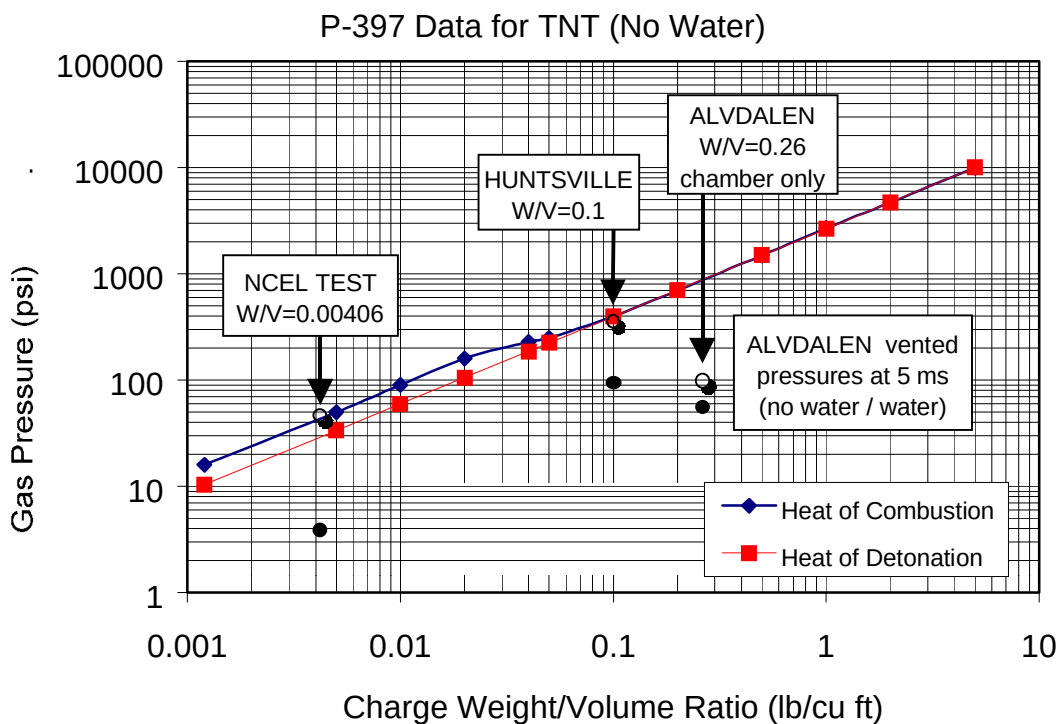
Figure 6. Gas pressure mitigation in the feasibility tests.
