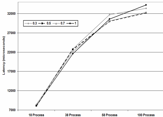
Figure 8: Average Latency.
