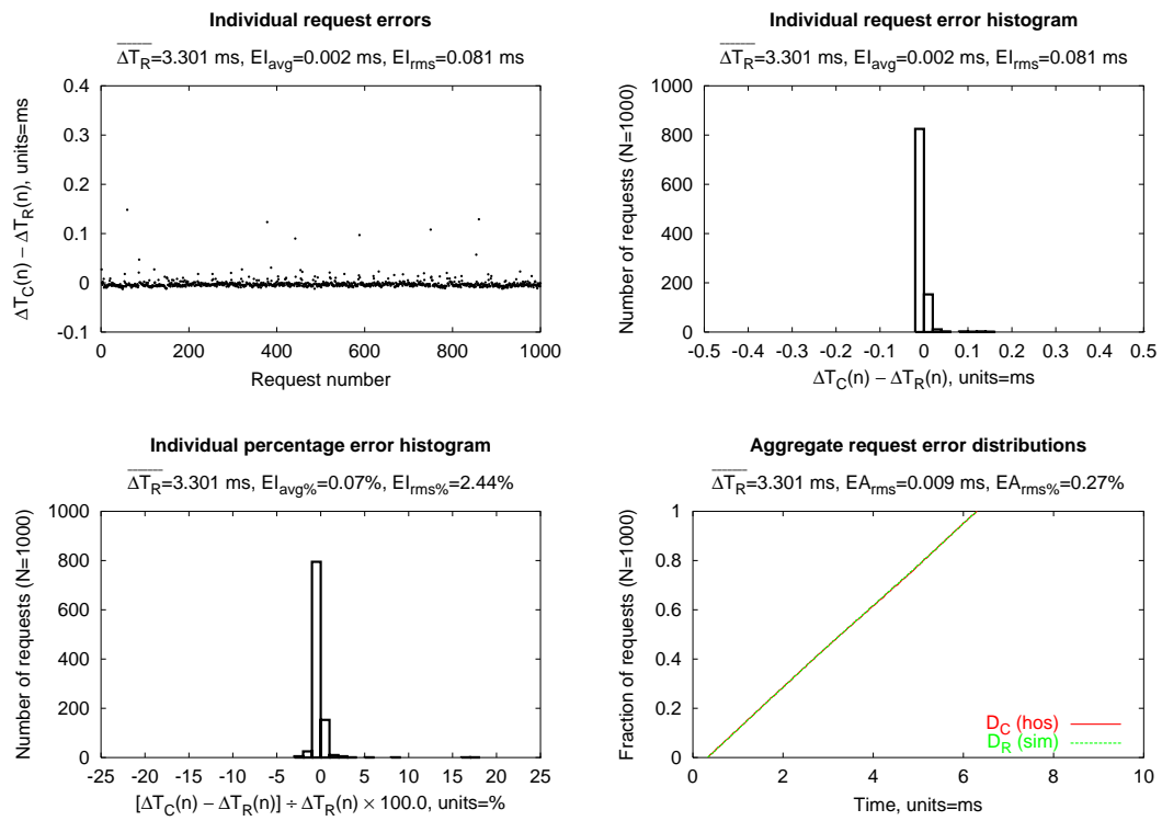
Figure 5.29: E_{1 \rightarrow 3} : \Delta T_{lookahead} = 30 \mu\text{s} , \Delta T_{skew} = 60 \mu\text{s} , Adaptec, 4 KB Writes.
