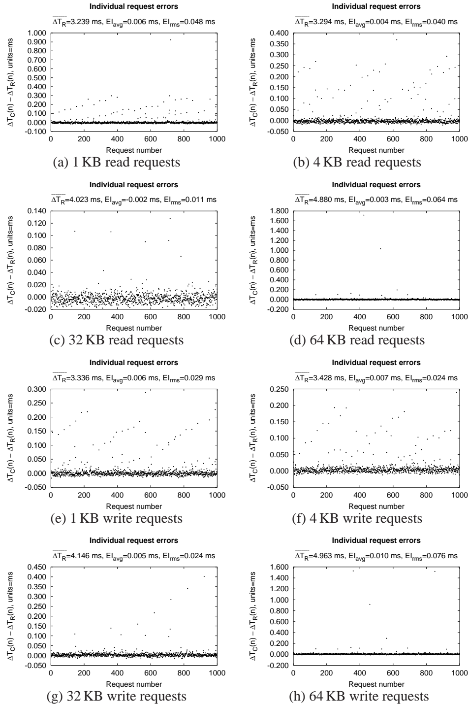
Figure D.10: E_{1 \rightarrow 3} : \Delta T_{lookahead}=30 \mu s , \Delta T_{skew}=151 \mu s , QLogic.
