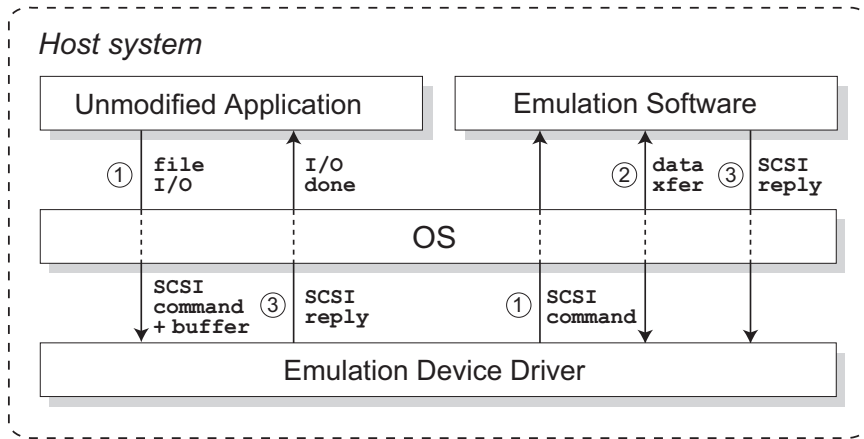
Figure 3.2: Communication paths under local emulation. As described in Section 3.2.2.1, emulation software communicates directly with a modified device driver in the kernel when run locally. The three external interactions shown here are explained in detail in Section 3.2.1.
