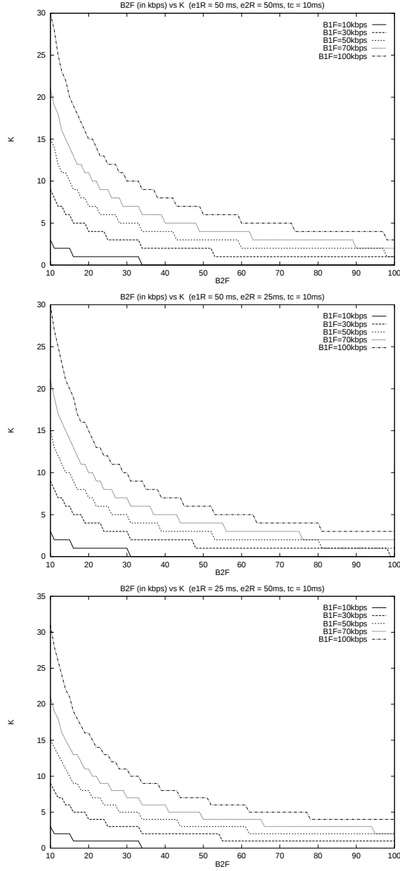
Figure 6.4: Graphing K analytically: 10\text{kbps} \leq B_{1F}, B_{2F} \leq 100\text{kbps}
