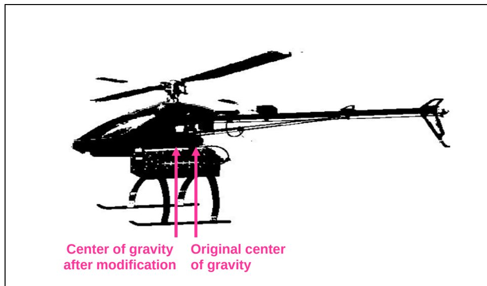
Figure 4. CG is shifted \sim 1.75 in forward.
