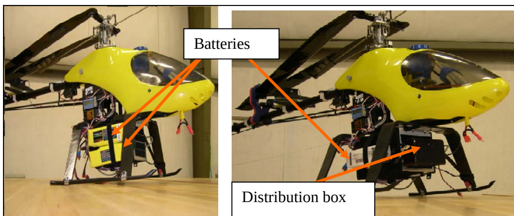
Figure 3. The original configuration is shown on the left. A third battery on the other side of the original electronics box is not visible here. The new configuration with a power distribution box is shown on the right.
