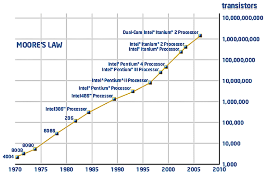
Figure 3 Moore's Law 41
