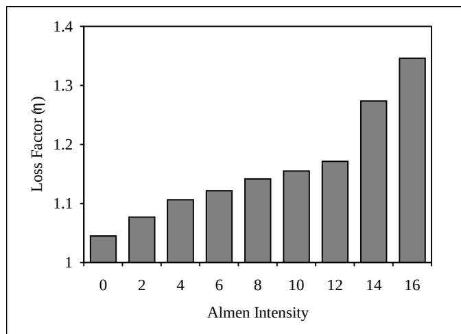
Figure 9 — The loss factor \eta defined in Equation 1 as a function of the peening intensity.
