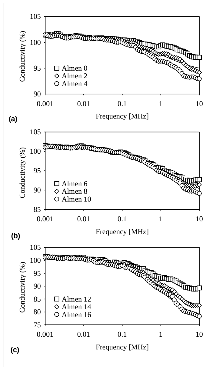
Figure 8 — The measured apparent electrical conductivity of nine C11000 specimens of varying surface roughness as a function of frequency.
