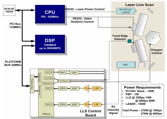
Figure 3. Synchronous scan imager block diagram.
