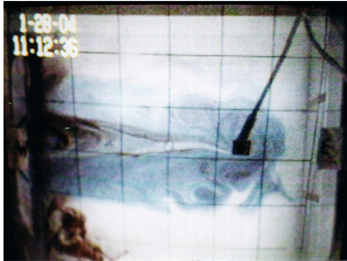
Figure B-2: A photograph of the steady state circulation pattern (visualized by colored dye) that shows a zonal jet at the latitude of the forcing flanked by a pair of counter-rotating recirculation gyres consistent with the numerical simulations.
