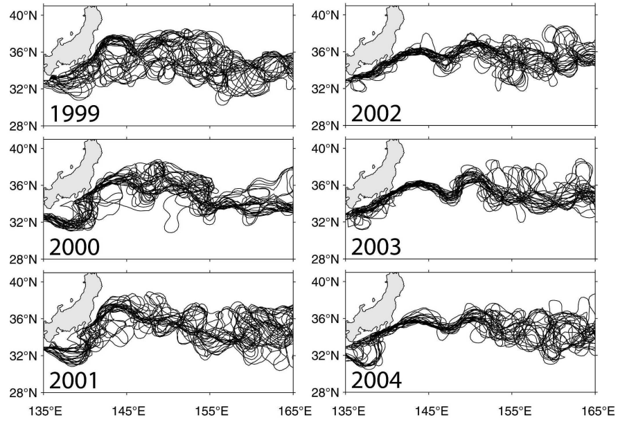
Figure 1-5: The contrast in the jet's meandering in the strongly meandering state (1999-2001) vs. the weakly meandering state (2002-2004) as seen by superimposed paths of the Kuroshio and Kuroshio Extension defined by the 170-cm contours in the weekly SSH fields. Here paths are plotted every 14 days (from Qui and Chen, 2005).
