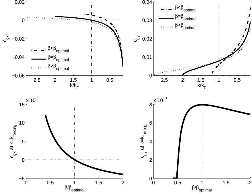
Figure 2-10: A visualization of the effect of changing the population of waves excited by the forcing on energy radiation from the plunger. As \beta is increased from \beta < \beta_{\text{optimal}} to \beta > \beta_{\text{optimal}} , waves with eastward zonal group velocity ( c_{gx} > 0 ) are included in the population of excited waves. \beta_{\text{optimal}} is set by the conditions of c_{gx} = 0 and c_{gy} maximized at the forcing scale k_F .
