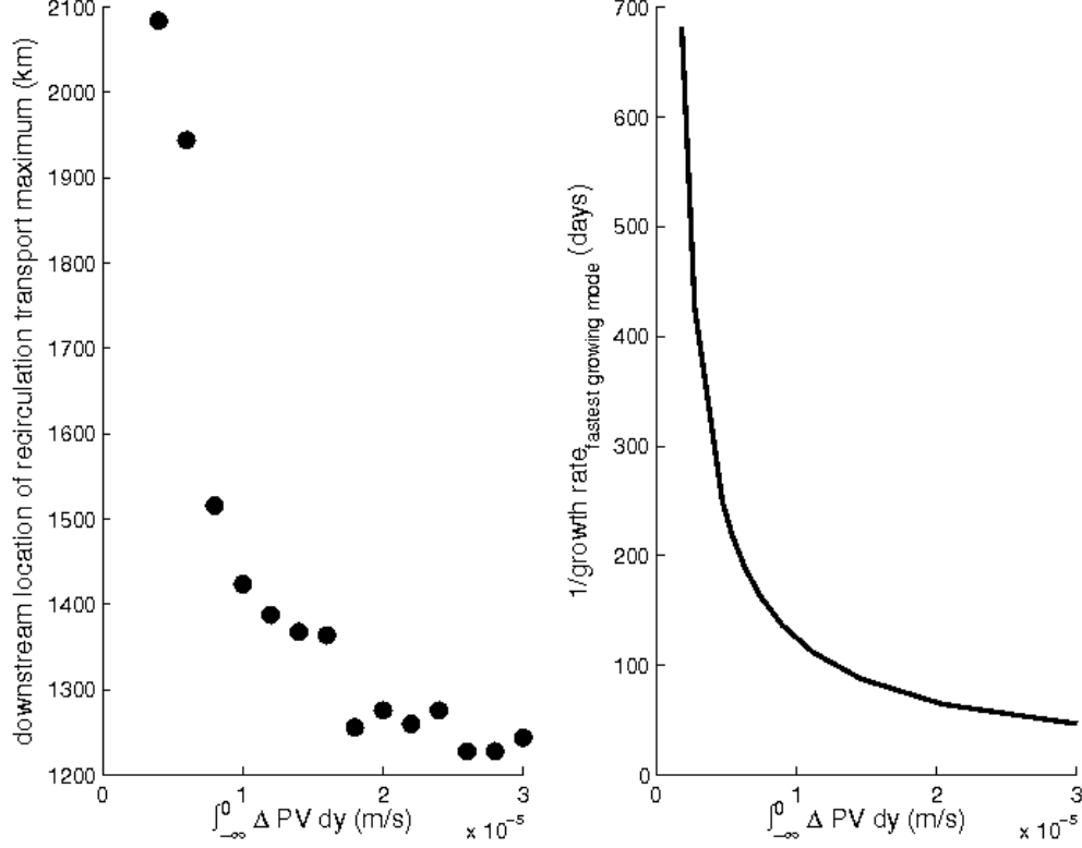
Figure 3-14: The dependence of recirculation zonal extent (as measured by the downstream location of maximum time-mean recirculation transport, \bar{\psi}_{max} - \bar{\psi}_{min} ) ( left ) vs. inverse growth rate (from the linear stability calculation for the inflowing jet profile) ( right ) on forcing amplitude.
