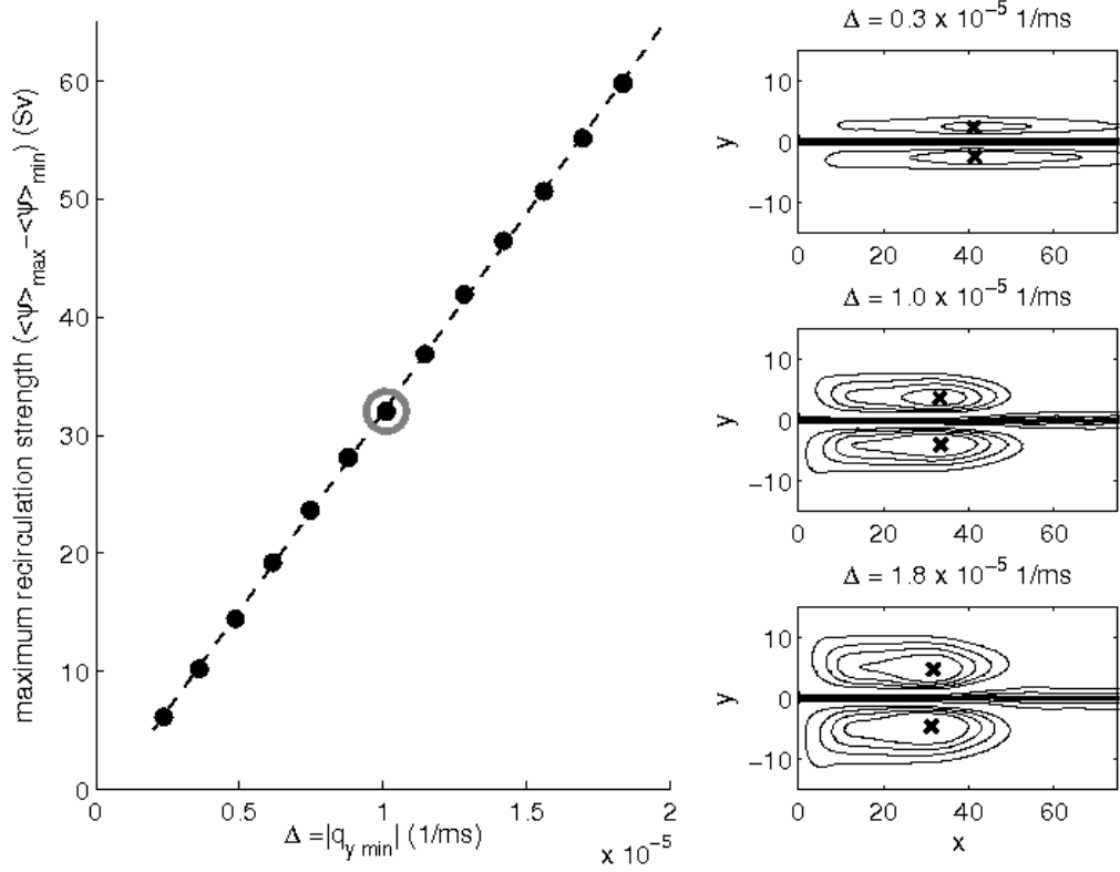
Figure 3-12: The dependence of the mean recirculation strength (as measured by the maximum time-mean recirculation transport, \bar{\psi}_{\max} - \bar{\psi}_{\min} ) on the supercriticality of the inflowing jet, \Delta (as measured by the depth of the negative region in the jet's meridional PV gradient profile, |q_{y \min}| ) in a physically relevant range of parameters ( 0.04 \leq \beta \leq 0.4 ) ( left ). An estimate for the supercriticality of the KE, determined from the synoptic mean velocity profile of the Kuroshio jet at the point of separation from the coast derived from satellite altimetry data (see Figure C-1), is indicated by the gray circle. The time-mean circulation (streamfunctions) for small ( top ), moderate ( middle ), and large ( bottom ) inflowing jet supercriticalities showing the changing nature of the recirculation gyres as the entering jet becomes increasingly unstable ( right ).
