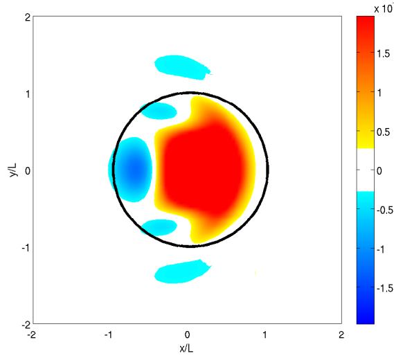
Figure 2-4: Eddy enstrophy destruction ( \overline{\vec{u}'\zeta' \cdot \nabla \zeta} ) (color) which indicates the direction of the eddy vorticity transport relative to the prevailing gradient (positive implies an eddy vorticity flux up the mean vorticity gradient; negative implies an eddy vorticity flux down the mean vorticity gradient).
