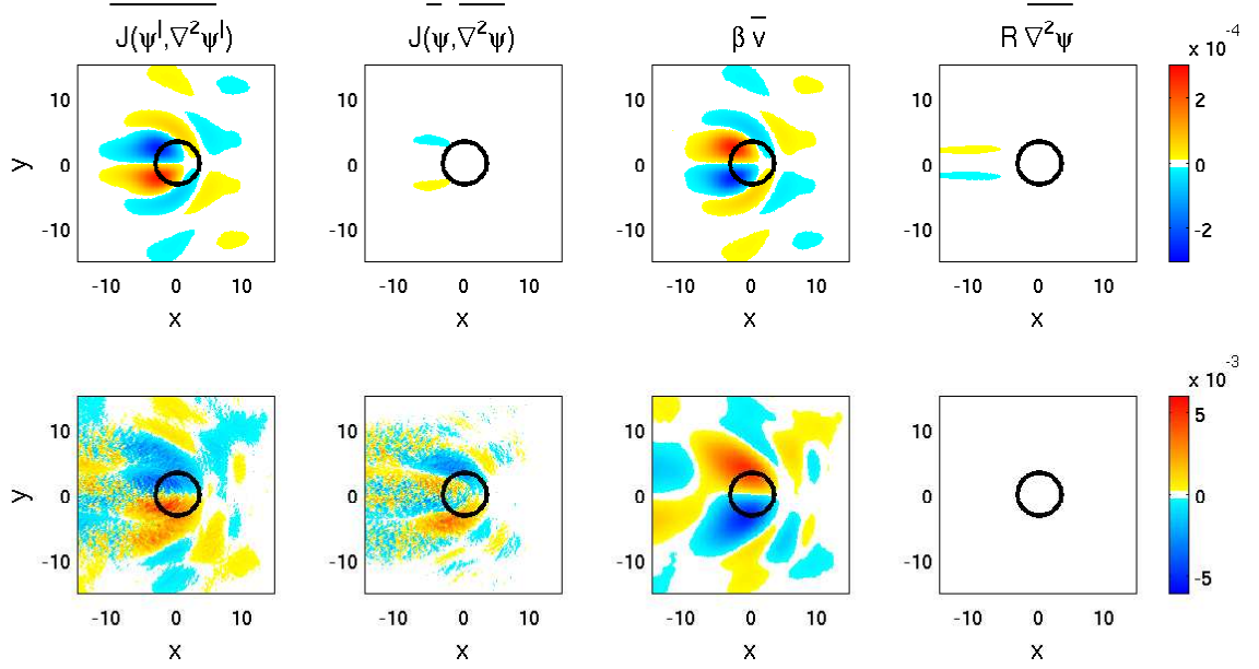
Figure 2-23: The time-mean vorticity balance: \overline{J(\psi', \nabla^2 \psi')} + \overline{J(\bar{\psi}, \nabla^2 \bar{\psi})} + \beta \bar{v} = -\overline{R \nabla^2 \bar{\psi}} for the weakly nonlinear case ( top ) vs. the strongly nonlinear case ( bottom ).
