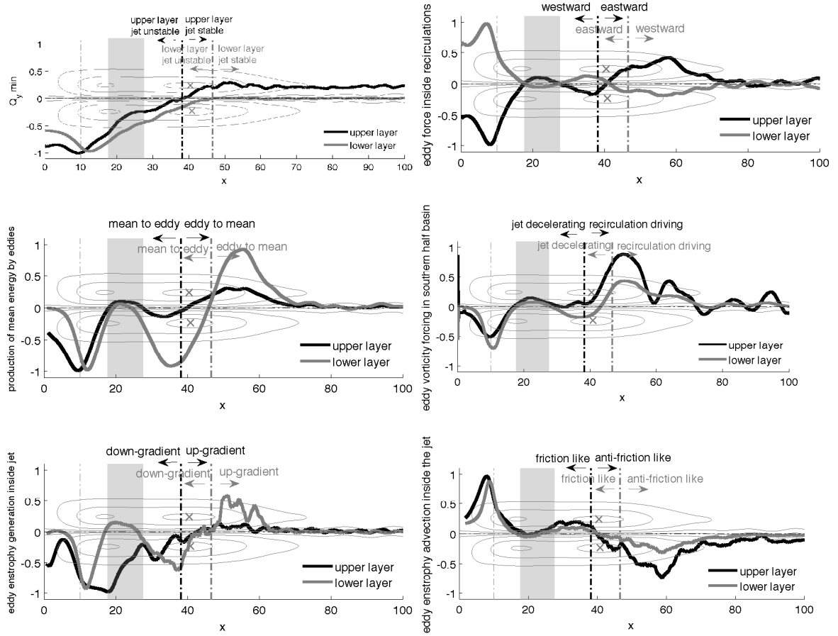
Figure 3-23: As in Figure 3-9, the downstream evolution of (a) the time-mean jet's stability properties ( \bar{q}_{ny \min} ) ( upper left ) (b) the effective eddy force ( upper right ) (c) the production of mean kinetic energy by the eddies ( middle left ) (d) the sense of the eddy vorticity forcing ( middle right ) (e) the eddy enstrophy destruction inside the time-mean jet ( lower left ) and (f) the sign of the eddy enstrophy advection ( lower right ). Properties of the upper layer are plotted in black and properties of the lower layer are in gray. The background contours are that of the barotropic streamfunction ( \psi_{BT} = \frac{1}{S_2}\psi_1 + \frac{1}{S_1}\psi_2 ). The shaded region denotes the boundaries of a new upstream region that is a feature of the mixed instability case. See the text for a full discussion.
