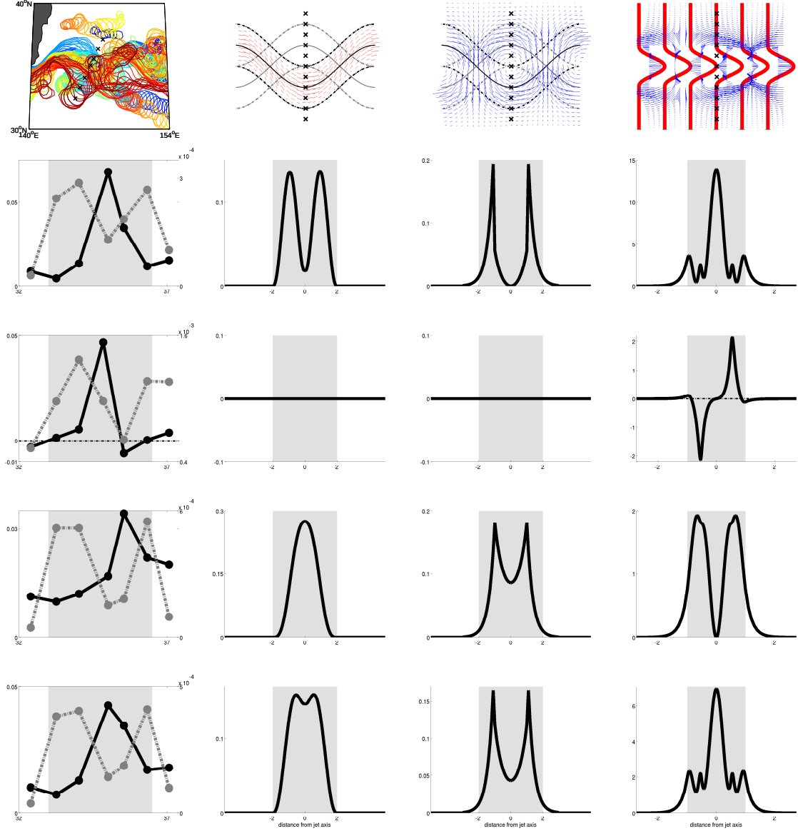
Figure 4-24: The cross-jet distributions of \overline{u'u'} ( 2^{nd} row), \overline{u'v'} ( 3^{rd} row), \overline{v'v'} ( 4^{th} row) and \overline{EKE} = \frac{1}{2} (\overline{u'u'} + \overline{v'v'}) ( 5^{th} row) observed at the KESS mooring array ( 1^{st} column) compared to those of various idealized models: 1. a meandering jet ( 2^{nd} column) 2. the Rossby wave field generated by a meandering jet ( 3^{rd} column) and 3. a barotropically unstable jet ( 4^{th} column). The KESS observations are shown for the upper ocean (at 250 m depth) in black scaled by the left-hand axes, and the deep ocean (averaged over 1500 m, 2000 m, 3500 m and 5000 m depth) in gray scaled by the right-hand axes. Velocity fields were band-passed filtered in the mesoscale range (periods of 10 - 100 days) before the variances and covariances were computed to clarify the cross-jet variations. The gray shading indicates the width of the time-mean jet in all columns.
