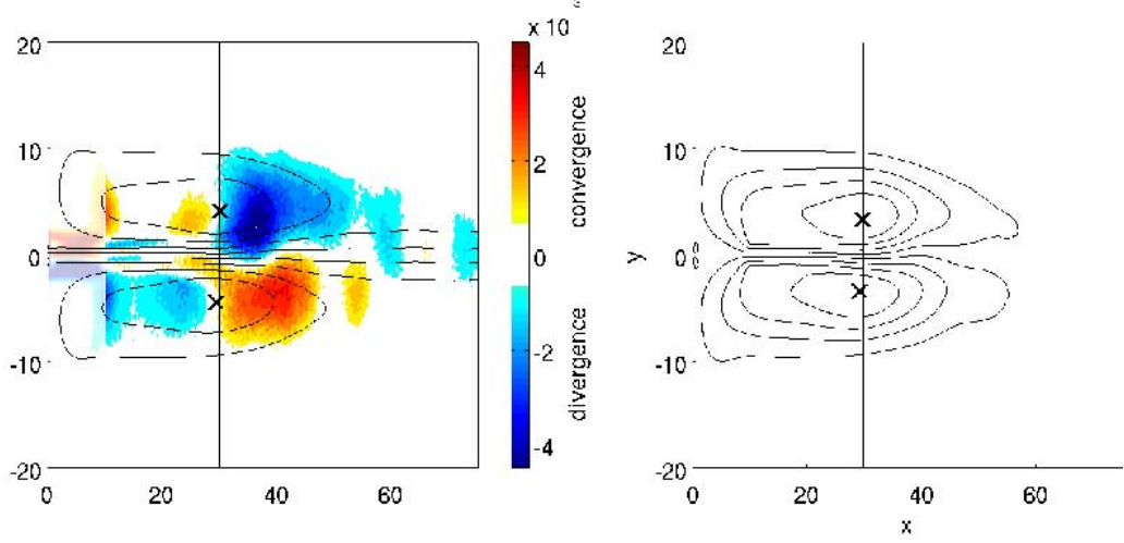
Figure 3-3: The eddy vorticity forcing (the negative of the divergence of the eddy vorticity flux (-\nabla \cdot (\mathbf{u}'q')) = -\overline{(u'u')_{xy}} + \overline{(v'v')_{xy}} + \overline{(u'v')_{xx}} - \overline{(u'v')_{yy}} ) (color) overlaid on the properties of the time-mean streamfunction ( left ). The time-mean circulation driven by the eddy vorticity forcing, computed as the solution to the linear vorticity equation forced statically by the above eddy vorticity forcing field ( right ).
