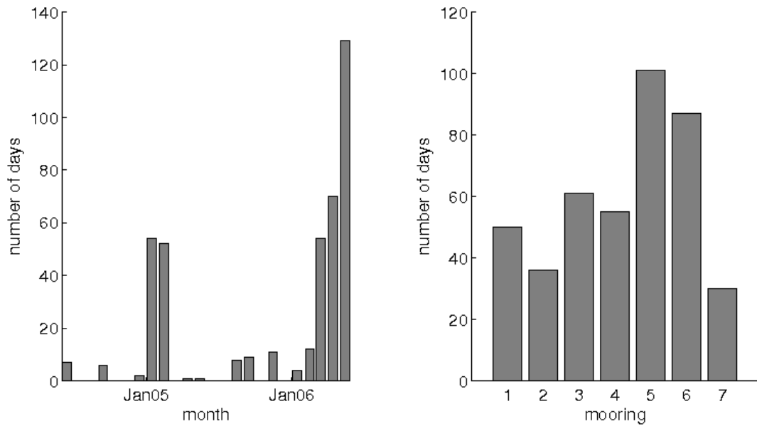
Figure 4-15: Histograms showing the distribution of “ring events” (days when a ring was present at a mooring location based on the temperature criterion described in Appendix D) in time ( left ) and space ( right ). Bins are months and moorings respectively, with “1” denoting the mooring K1 (the northern-most mooring in the array) and “7” denoting the mooring K7 (the southern-most mooring in the array). Note that if a ring was present at more than one mooring on a given day, it is counted as more than one day, resulting in counts in some months that exceed the number of days in that month.
