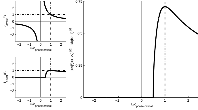
Figure 2-20: An explanation for the asymmetry in the rectification response for U < U_{\text{optimal}} vs. U > U_{\text{optimal}} based on the changing relation between k and l for a Rossby wave with |k| > B vs. |k| < B . For |k| > B (corresponding to U < U_{\text{optimal}} if one takes k to be the arrested wavenumber), k \ll l , but near |k| = B , l increases rapidly to a comparable magnitude ( left ). This produces a rapid increase in the relative magnitude of kl (characteristic of the size of \overline{u'v'} ) ( right ). For |k| < B (corresponding to U > U_{\text{optimal}} again if k is taken to be the arrested wavenumber) however, the change in both k and l is much slower, and hence they remain of comparable magnitude over a much larger range of k / U . This may account for the much slower change in rectification effectiveness observed.
