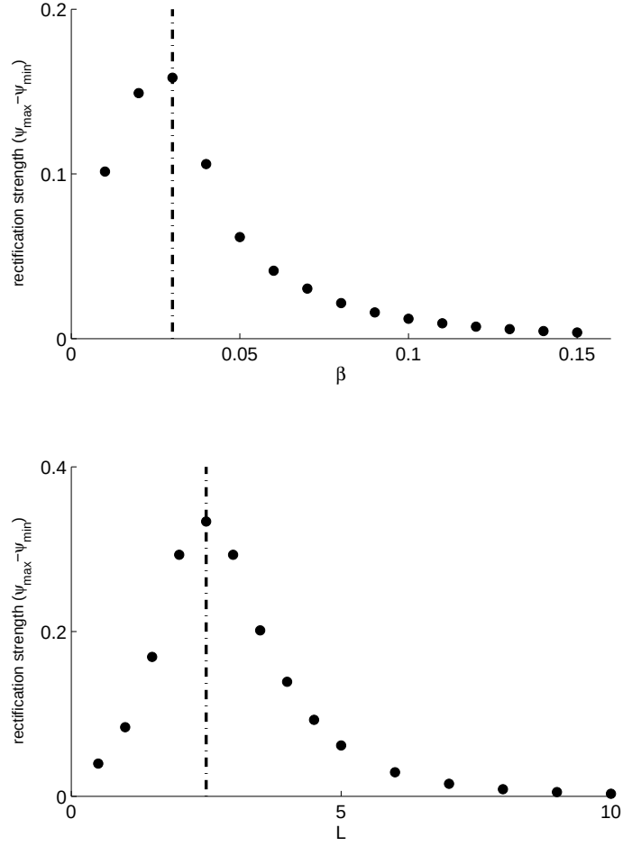
Figure 2-6: Dependence of mean rectified flow strength ( \bar{\psi}_{\max} - \bar{\psi}_{\min} ) (“rectification effectiveness”) on select parameters of the problem: \beta ( top ) and forcing length scale L ( bottom ). Dashed lines indicate the parameter value corresponding to the peak or optimal response in the observed non-monotonic dependence of rectified flow strength on each of these parameters.
