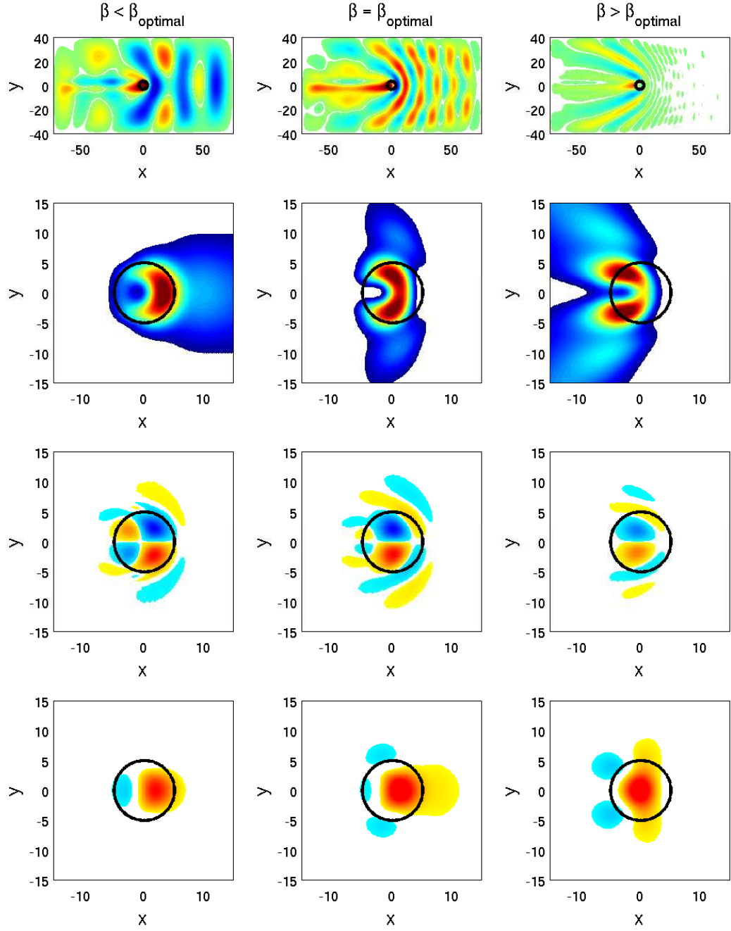
Figure 2-9: The effect of varying \beta from \beta < \beta_{\text{optimal}} to \beta > \beta_{\text{optimal}} on: (a) the population of waves excited (1 st row); (b) the orientation of energy radiation from the forcing (2 nd row); (c) the patterns of eddy relative vorticity flux divergence (3 rd row); (d) the patterns of eddy zonal momentum flux divergence (4 th row).
