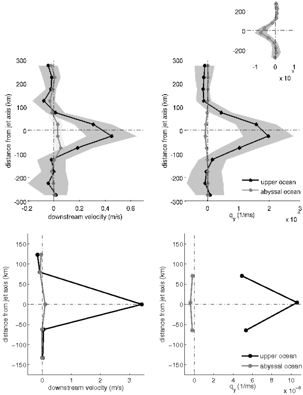
Figure 4-21: An approximate “upper layer” (black) and “lower layer” (gray) jet profile ( left ) formed by the velocity at 250 m depth and an average of the velocities at the abyssal depths respectively as measured by the KESS mooring array for the synoptic mean ( top ) and an extreme snapshot ( bottom ). Again shading in the synoptic mean indicates the mean \pm one standard deviation. The corresponding layered versions of the meridional PV gradient ( q_{1y} = -U_{1yy} + \beta + \frac{f^2}{N^2 D_1^2}(U1 - U2) and q_{2y} = -U_{2yy} + \beta + \frac{f^2}{N^2 D_2^2}(U2 - U1) ) using the above jet profiles and layer depths of 800 and 4000 m for D_1 and D_2 respectively ( right ). Here N is the buoyancy frequency, taken to be 0.005 \frac{1}{s} . All other symbols have been defined previously in the text.
