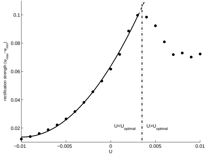
Figure 2-16: Dependence of mean rectified flow strength ( \overline{\psi}_{max} - \overline{\psi}_{min} ) (“rectification effectiveness”) on the value of the constant zonal background flow U .
