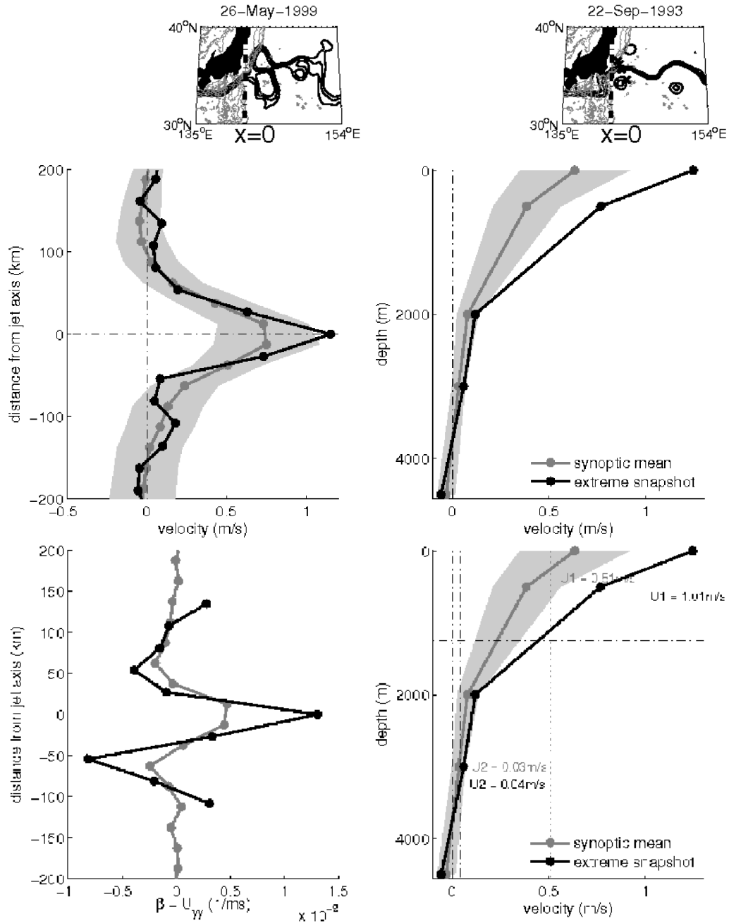
Figure 4-28: Synoptic (stream-coordinate) mean ( gray ) and an extreme snapshot ( black ) of the horizontal jet structure at 141.3°E (evaluated from the surface geostrophic velocity derived from the 14-year altimetry record) ( upper left ) and the vertical jet structure at the same approximate location (evaluated from the KERE mooring array) ( upper right ). Grey shading denotes the synoptic mean \pm one standard deviation. Snapshots of the KE jet state visualized via SSH (as in Figure 4-20) at the times corresponding to the extreme snapshots are above. Region bathymetry is shown in these snapshots by the gray contours (contours are at 2000, 4000, 6000 and 8000 m respectively), and the location of the KERE moorings is shown in the upper right by the xs. The implication of these shear magnitudes on the barotropic ( lower left ) and baroclinic ( lower right ) stability properties of the jet as in Figure 4-20 are shown in the lower panels.
