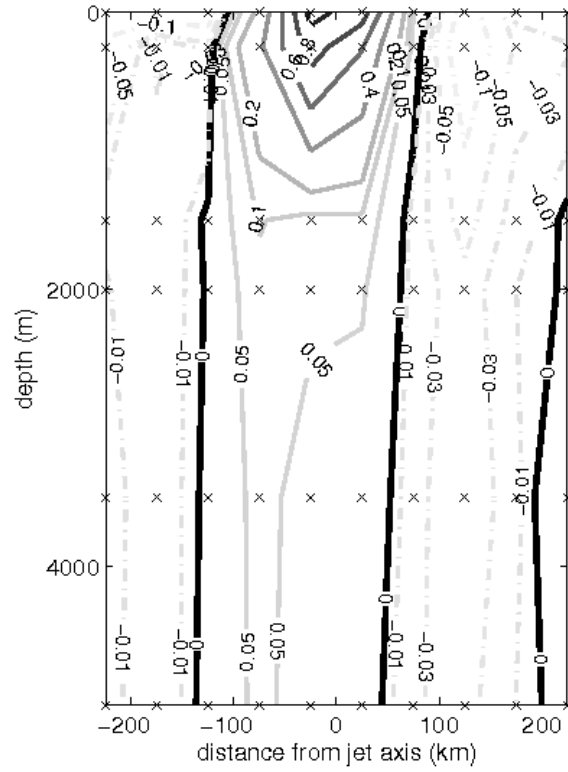
Figure 4-10: A contour plot of time-mean downstream velocity (in m/s) as a function of depth and distance from the jet axis summarizing the stream-coordinate description of the KESS period time-mean jet structure. Solid contours indicate positive (downstream) values while dashed contours indicate negative (upstream) values. Data locations are indicated by xs : an array of ten 50 km wide bins of distance from the jet axis in the horizontal, and six levels in the vertical (including velocity derived from satellite altimetry at the surface).
