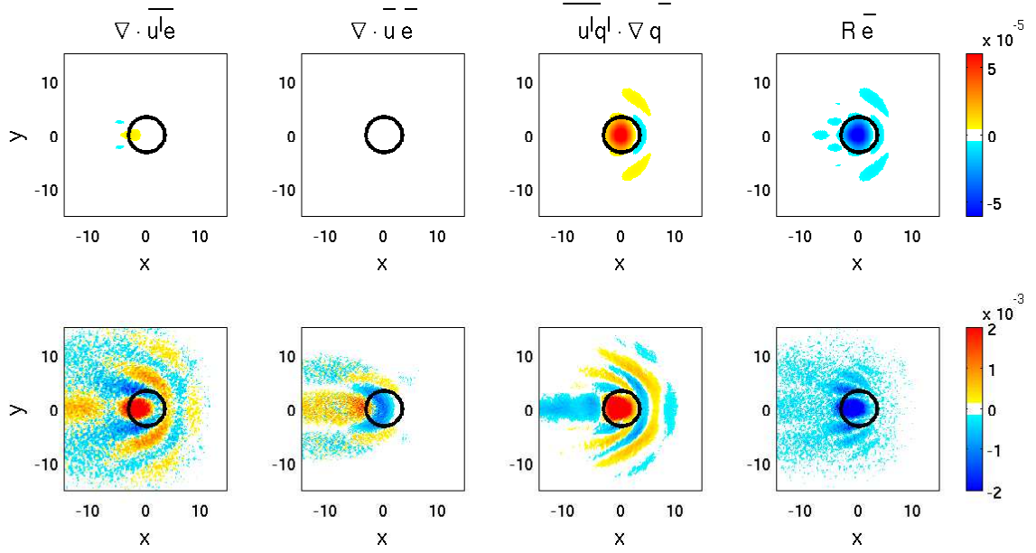
Figure 2-24: The time-mean enstrophy variance ( \frac{\zeta'^2}{2} ) budget: \nabla \cdot \overline{\mathbf{u}'\frac{\zeta'^2}{2}} + \overline{\mathbf{u}} \cdot \nabla \overline{\frac{\zeta'^2}{2}} + \overline{\mathbf{u}'\zeta'} \cdot \nabla \overline{\mathbf{q}} = -R\frac{\zeta'^2}{2} for the weakly nonlinear case ( top ) vs. the strongly nonlinear case ( bottom ).
