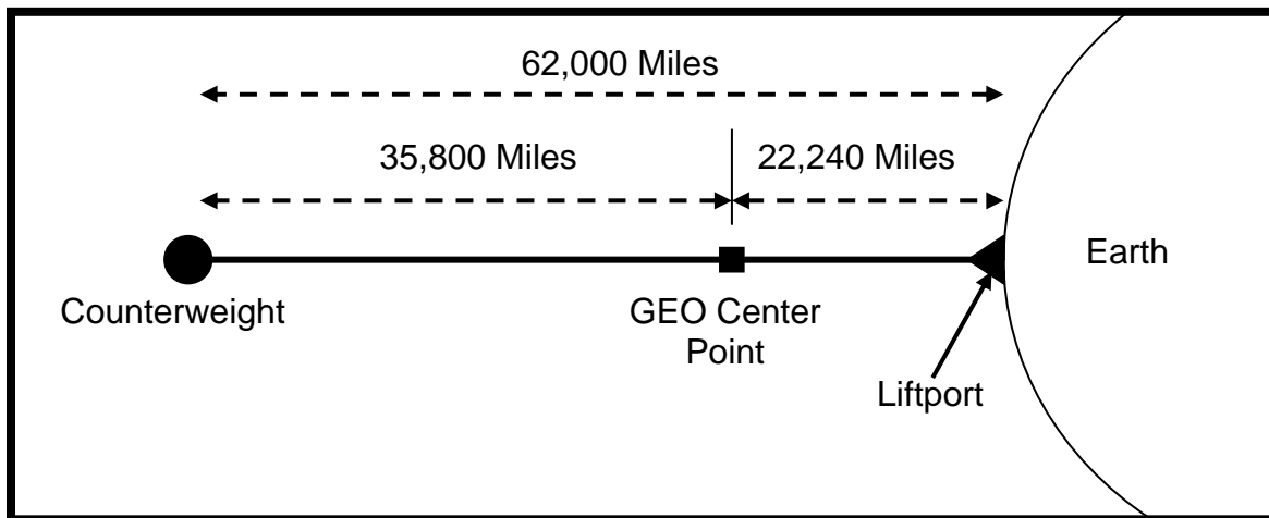
Space Elevator Basic Layout
