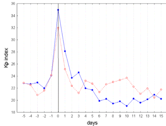
Fig.3. Kp-index for magnetic clouds with right-handed rotation (solid line, blue) and left-handed rotation (dashed line, red).
