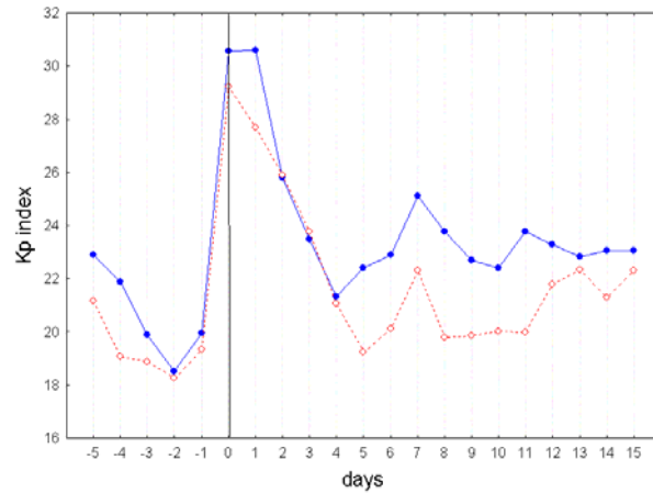
Fig.2. Kp index for high-speed solar wind in Westerly (solid line, blue) and Easterly (dashed line, red) phases of QBO.
