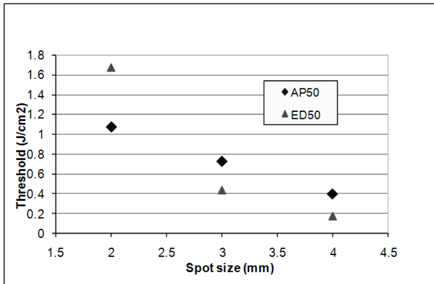
Figure 4: Radiant exposure ( \text{J}/\text{cm}^2 ) values for skin damage and action potential thresholds at 1064 nm.
