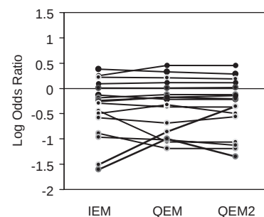
FIGURE 1. Estimation of adjusted individual effect sizes (IEM) using the QEM and QEM2 models with weight-adjusted effect sizes. The 2 discordant studies under QEM2 are those by Lasierra and Schreiber.
